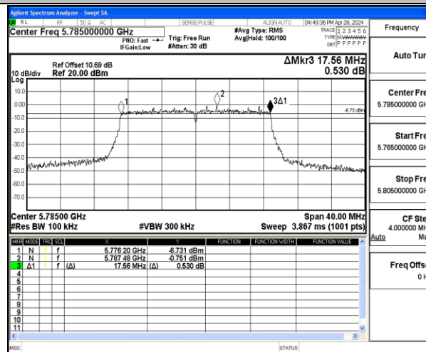
11N20MIMO-Ant1-5785-PASS
