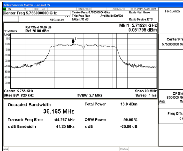
11AC40MIMO-Ant2-5755
