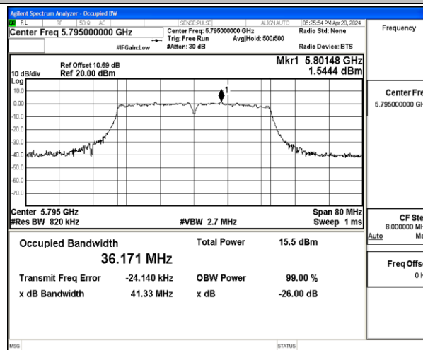
11AC40MIMO-Ant2-5795
