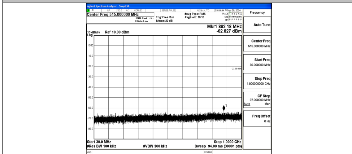
11N20MIMO-Ant1-2462-30~1000-PASS
