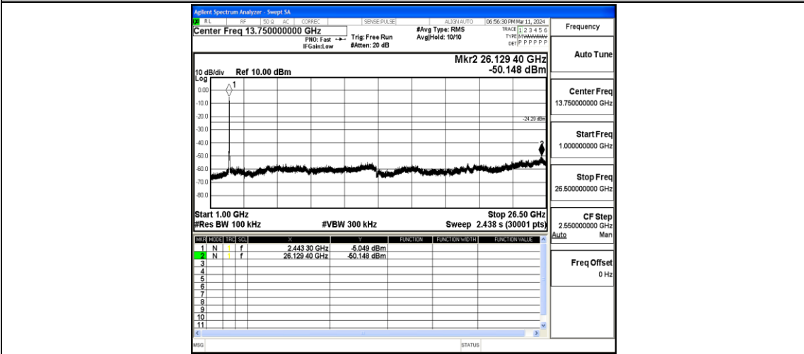
11N40MIMO-Ant1-2452-1000~26500-PASS
