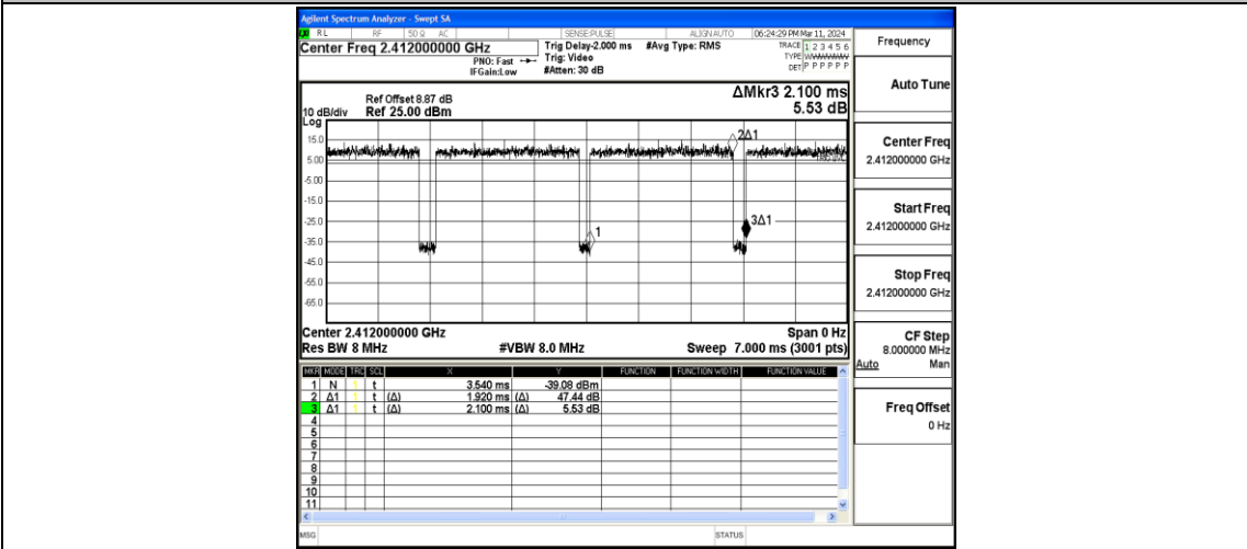
NTVN-11N20MIMO-Ant2-2412
