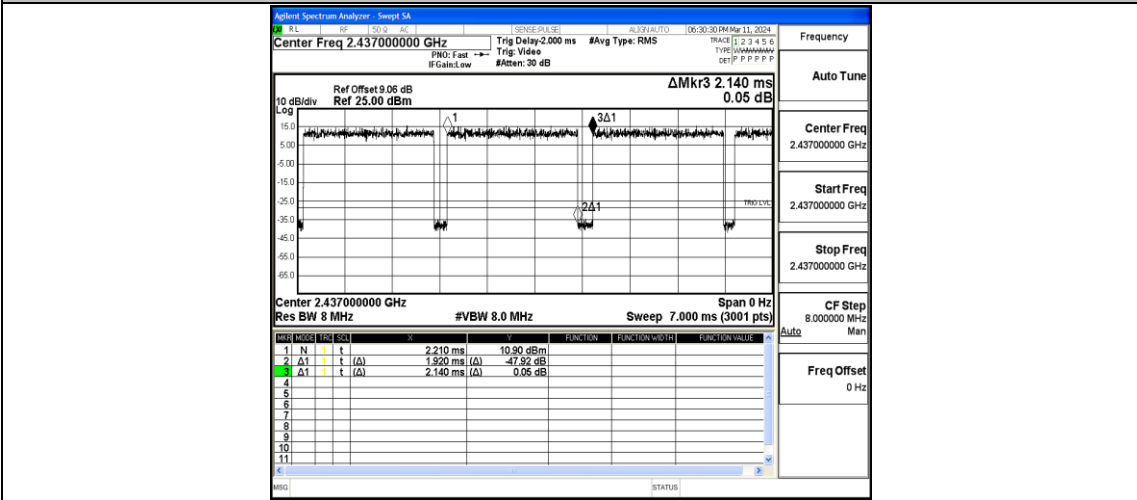
NTVN-11N20MIMO-Ant1-2437
