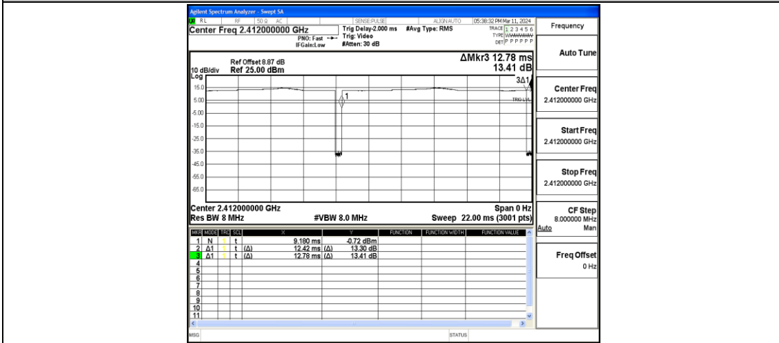
NTNV-11B-Ant2-2412
