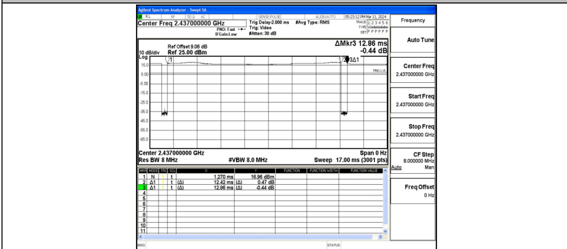
NTNV-11B-Ant1-2437
