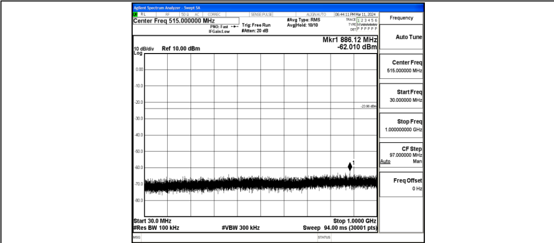
11N40MIMO-Ant1-2422-30~1000-PASS
