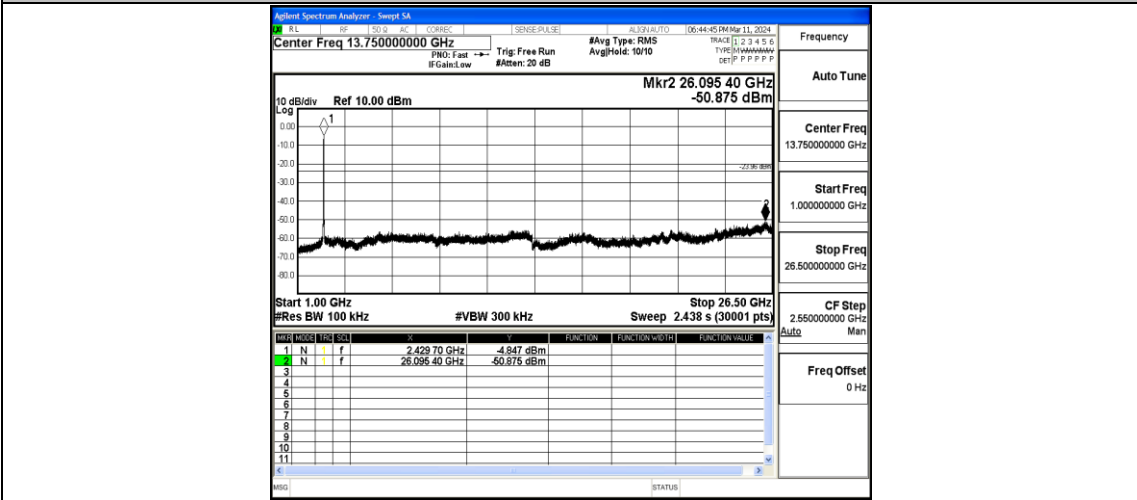
11N40MIMO-Ant1-2422-1000~26500-PASS
