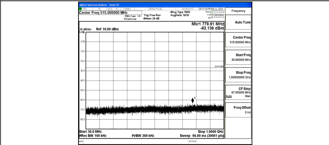
11N40MIMO-Ant2-2422-30~1000-PASS
