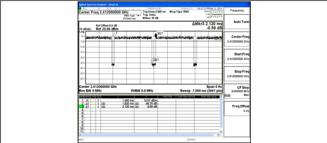
NTVN-11N20MIMO-Ant1-2412
