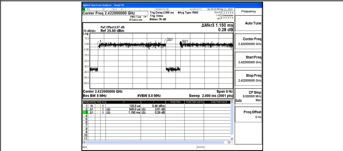
NTVN-11N40MIMO-Ant2-2422
