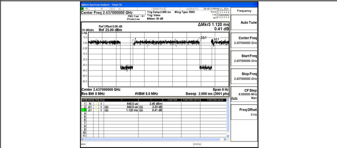
NTVN-11N40MIMO-Ant1-2437
