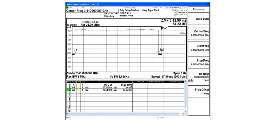
NTNV-11B-Ant1-2412
