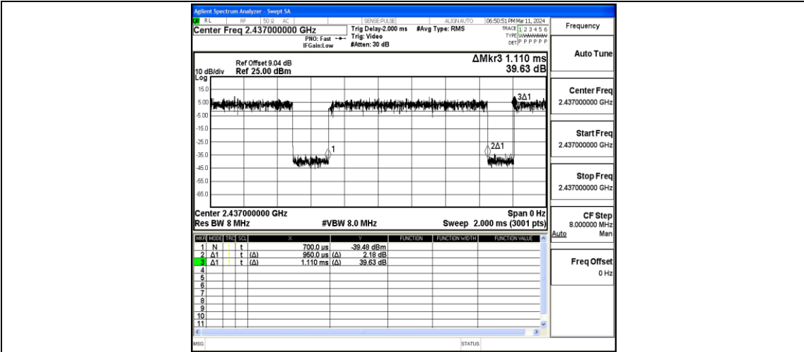
NTVN-11N40MIMO-Ant2-2437
