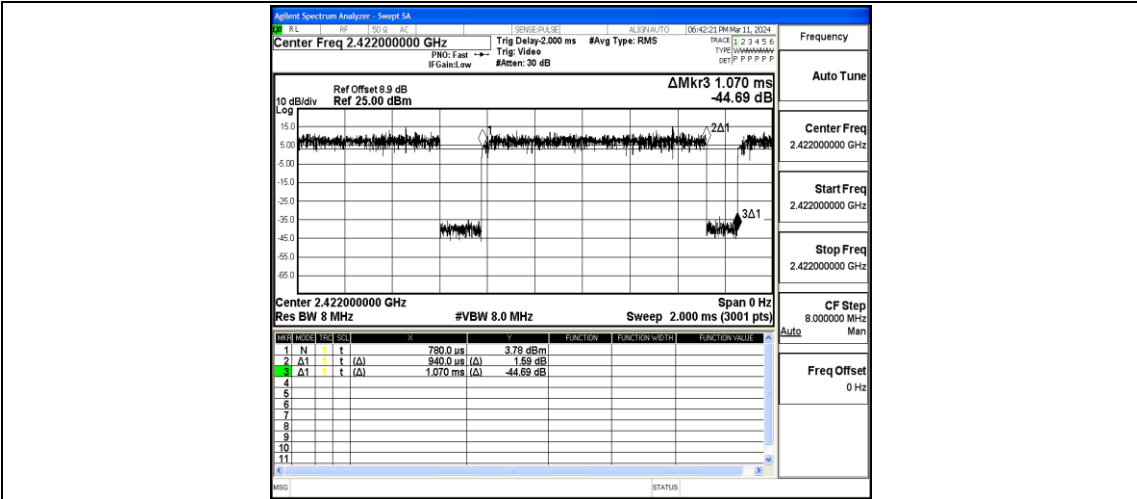
NTVN-11N40MIMO-Ant1-2422
