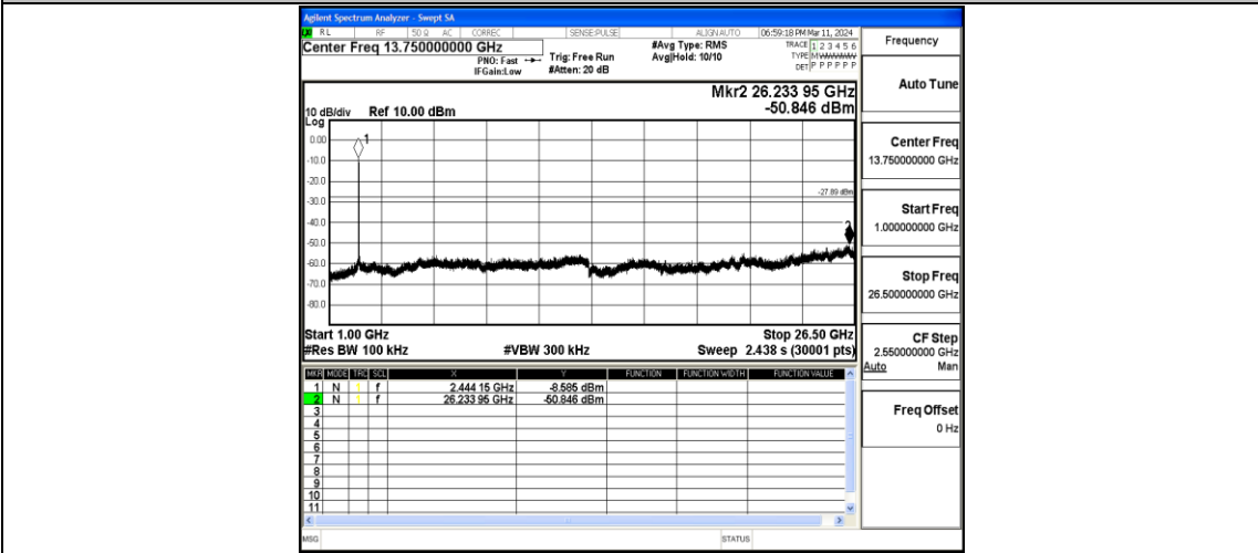
11N40MIMO-Ant2-2452-1000~26500-PASS
