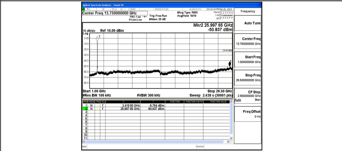
11N40SISO-Ant1-2422-1000~26500-PASS
