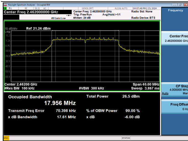
6 dB Bandwidth (802.11n_HT20-CH 11)
