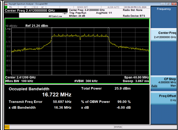
6 dB Bandwidth (802.11g-CH 1)
