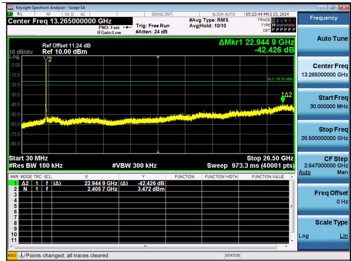
Spurious Emission (30 MHz – 26.5 GHz)
