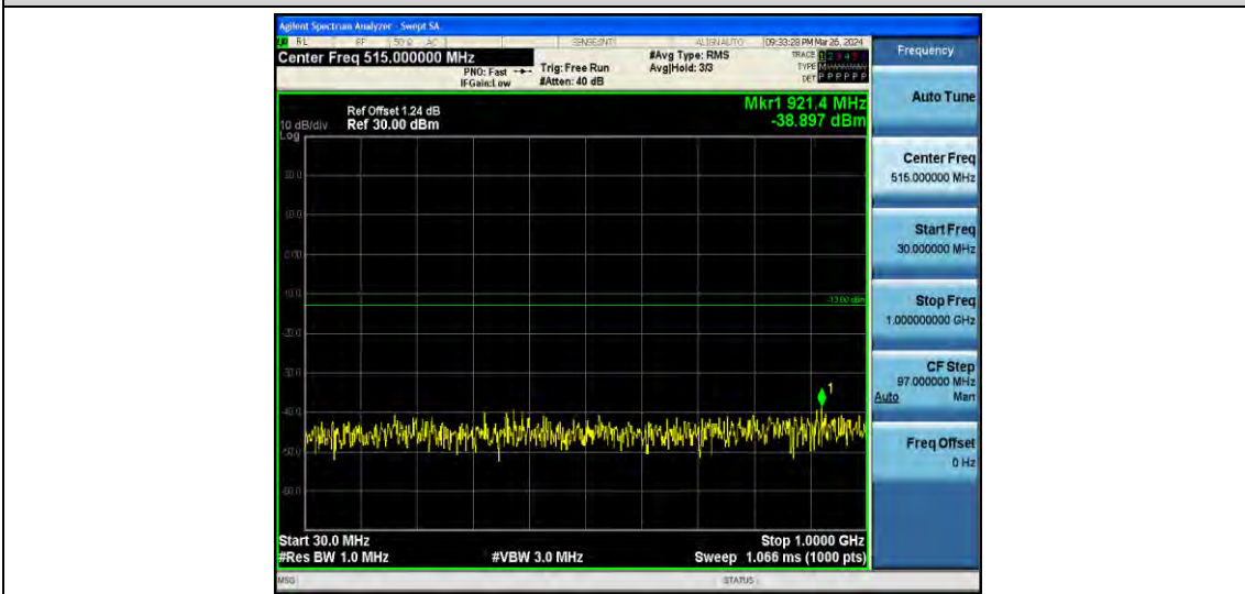
Band4-10MHz-16QAM-20000-1RB#0-Range2:1000~20000MHz
