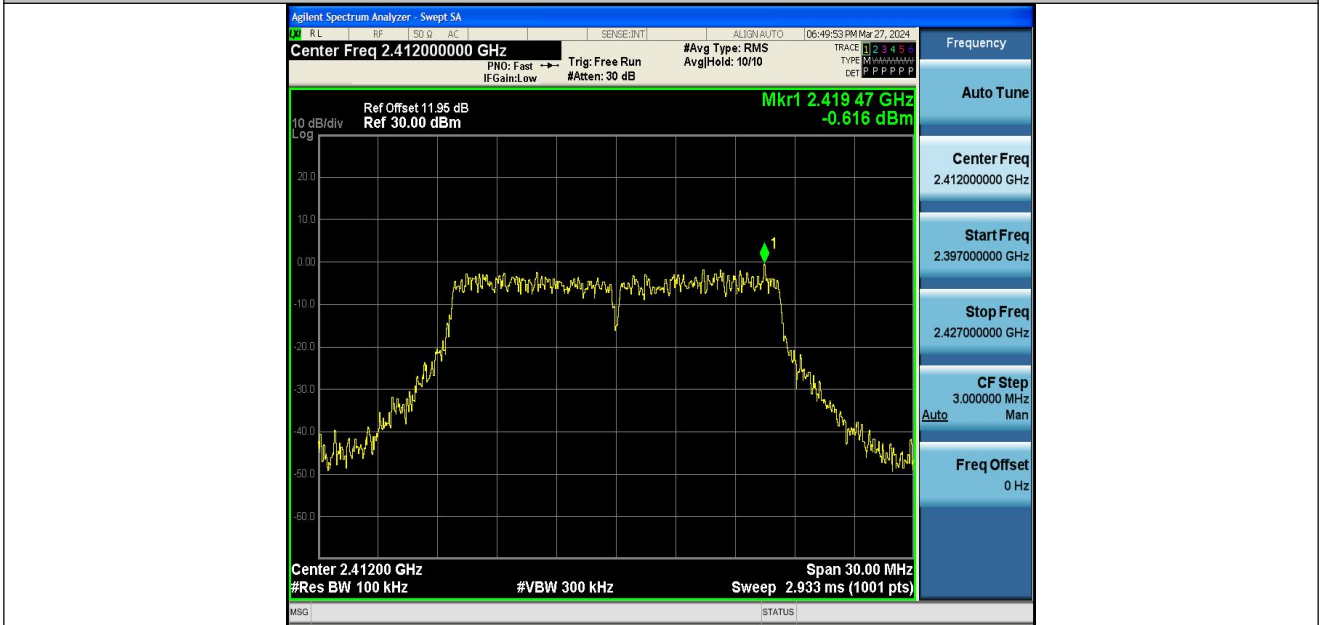
11G-Ant1-2412-0~Reference-PASS
