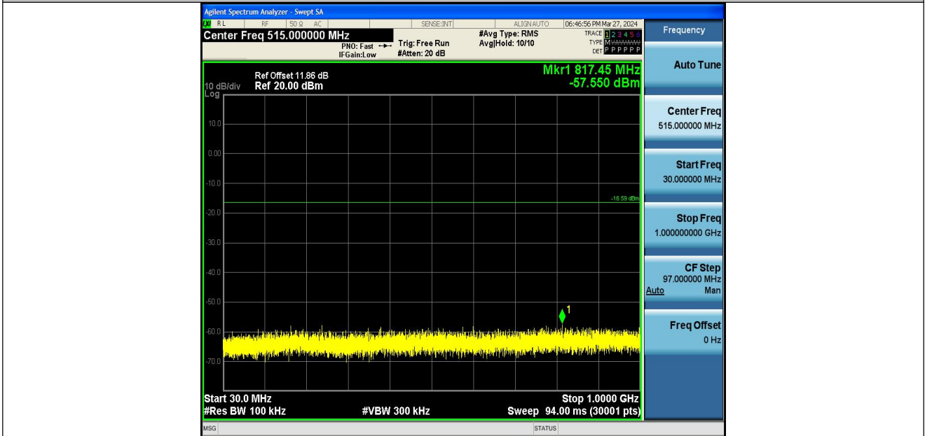
11B-Ant1-2462-30~1000-PASS
