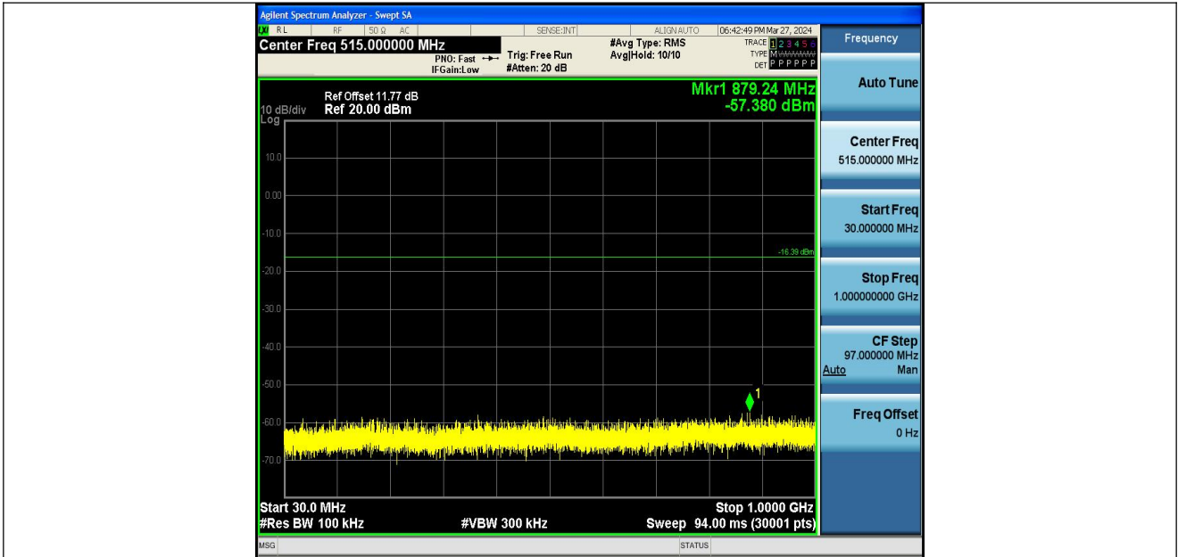
11B-Ant1-2437-30~1000-PASS
