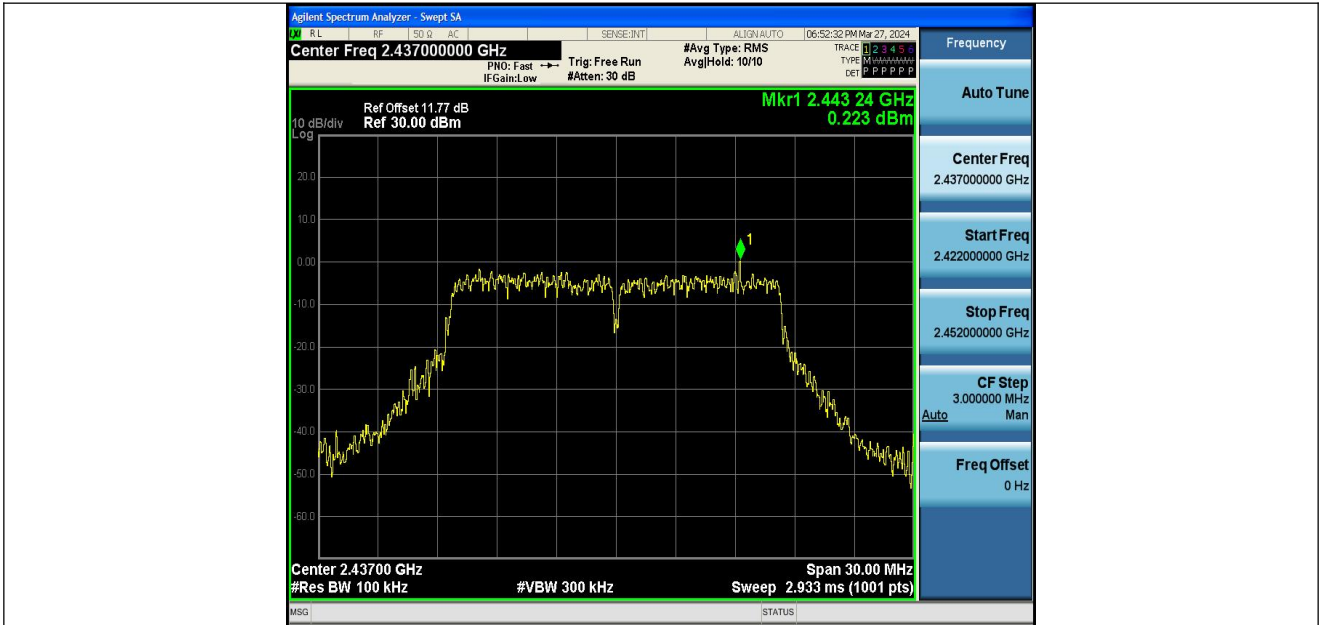
11G-Ant1-2437-0~Reference-PASS
