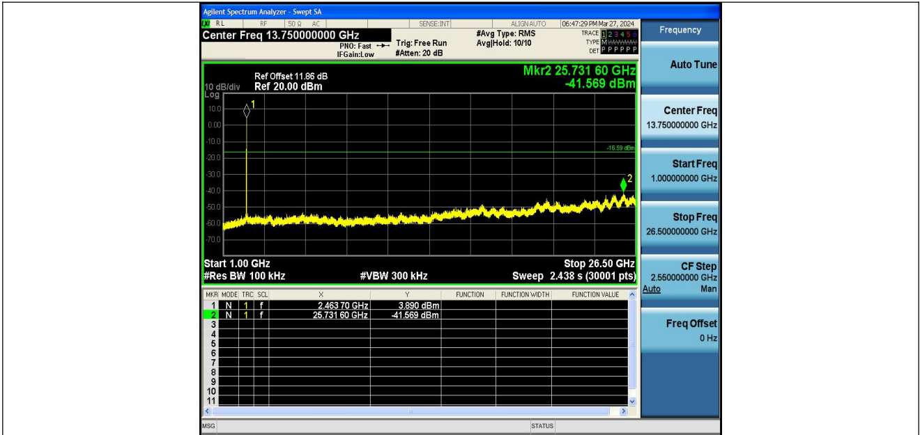
11B-Ant1-2462-1000~26500-PASS
