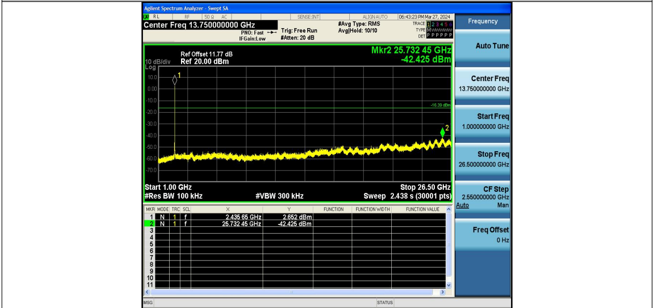
11B-Ant1-2437-1000~26500-PASS
