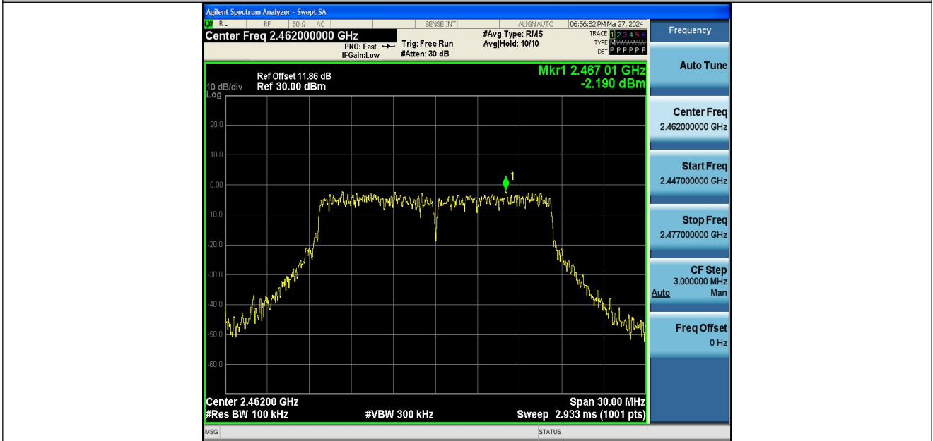
11G-Ant1-2462-0~Reference-PASS
