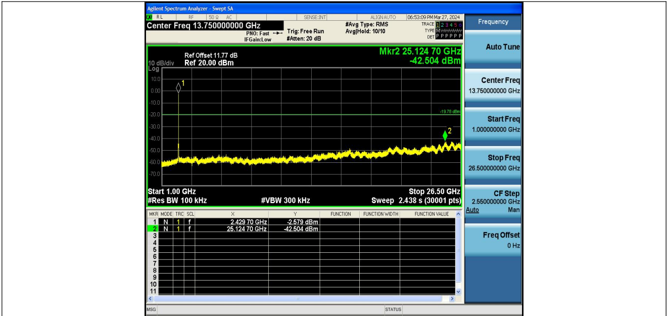
11G-Ant1-2437-1000~26500-PASS
