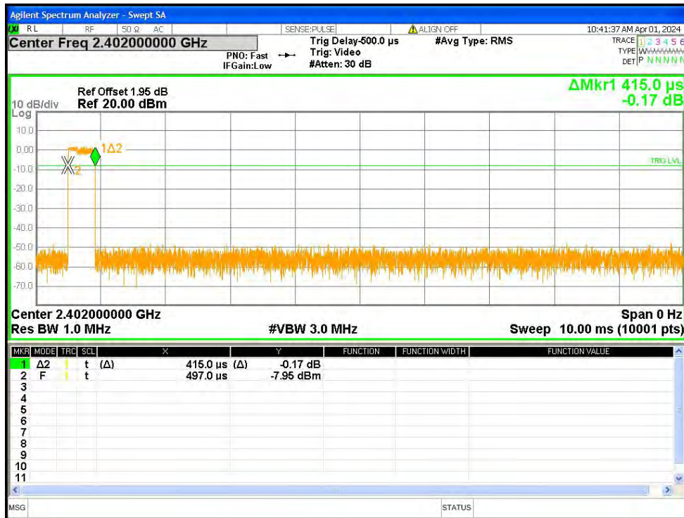
Dwell NVNT 3-DH1 2402MHz Ant1 One Burst
