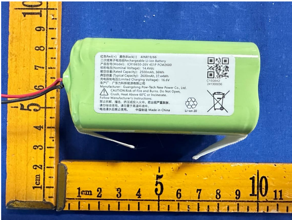
ICR18650-26V 4S1P PCM2600 (Primary protection)
