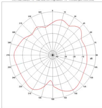
Far-field Power Distribution(H+V) on X-Z Plane Plot Peak Gain(H+V)= 1.20 dBi; Plot AvgGain(H+V)=- 3.83dBi @2.440GHz
