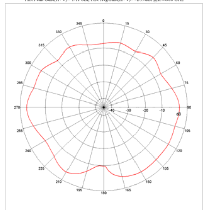
Far-field Power Distribution(H+V) on Y-Z Plane Plot Peak Gain(H+V)= 1.11 dBi; Plot AvgGain(H+V)=- 2.99dBi @2.440GHz
