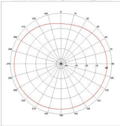
Far-field Power Distribution(H+V) on X-Y Plane Plot Peak Gain(H+V)= 1.03 dBi; Plot AvgGain(H+V)=- 0.48dBi @2.440GHz
