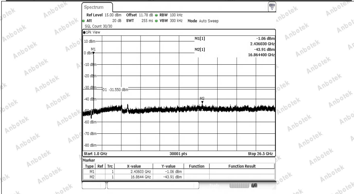
11G-Ant1-2437-1000~26500-PASS
