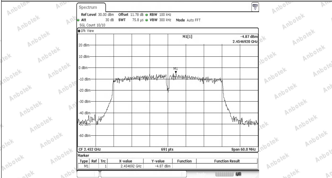
11N40SISO-Ant1-2452-0~Reference-PASS
