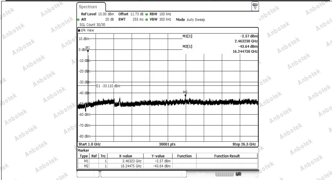
11N20SISO-Ant1-2462-1000~26500-PASS
