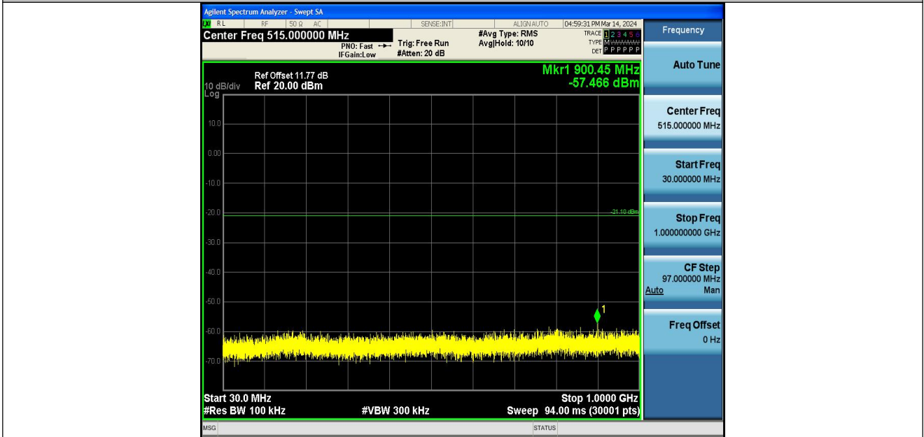
11N40SISO-Ant1-2437-30~1000-PASS
