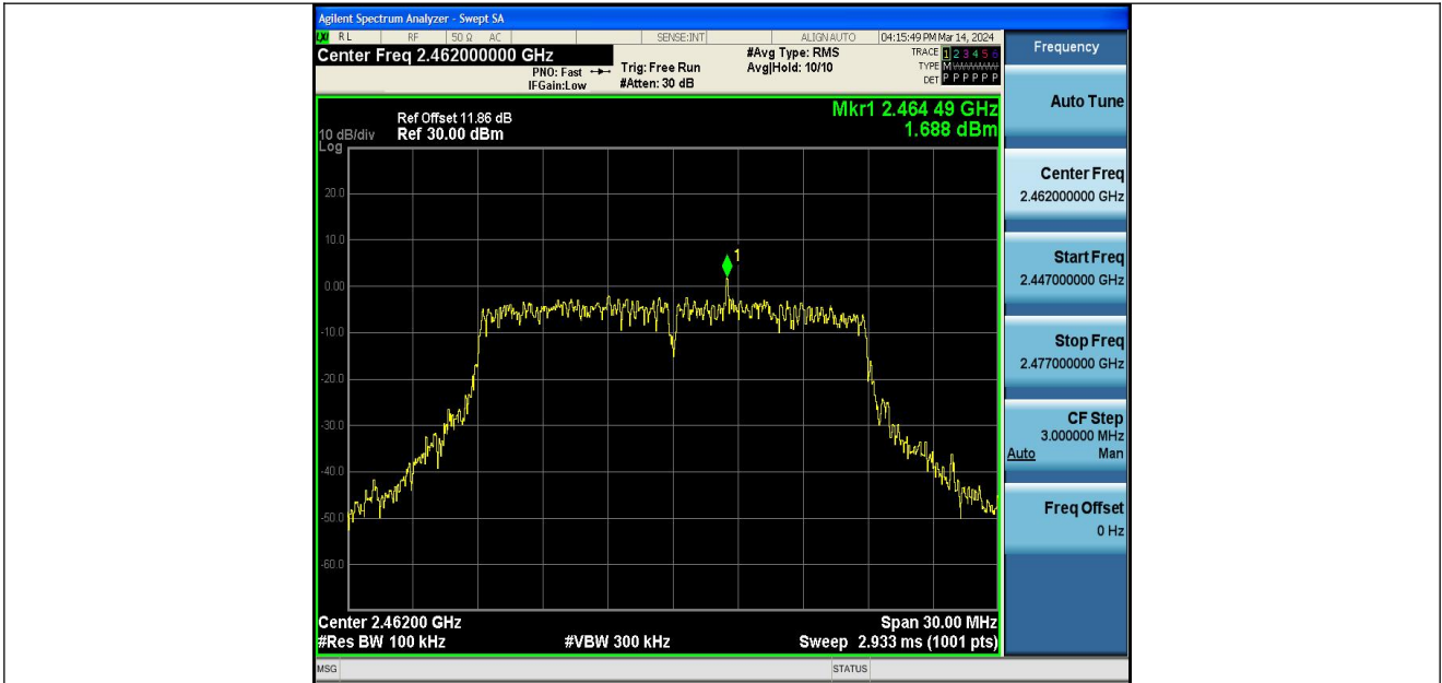
11N20SISO-Ant1-2462-0~Reference-PASS
