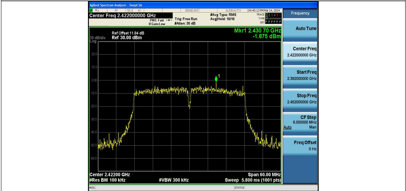
11N40SISO-Ant1-2422-0~Reference-PASS
