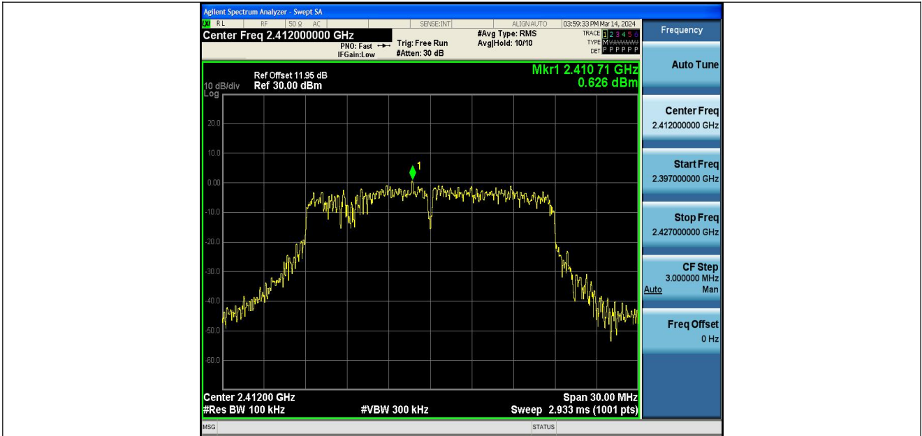
11N20SISO-Ant1-2412-0~Reference-PASS
