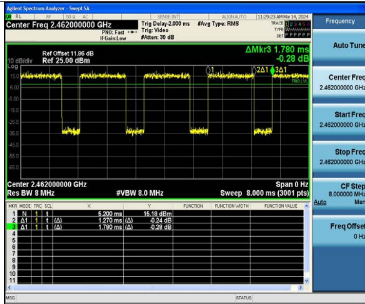
NTVN-11N20SISO-Ant1-2462
