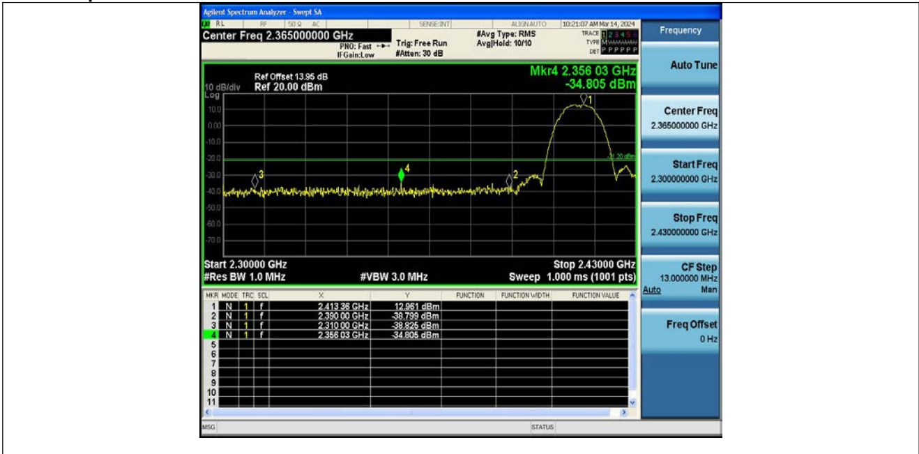
11B-Ant1-2412-PASS
