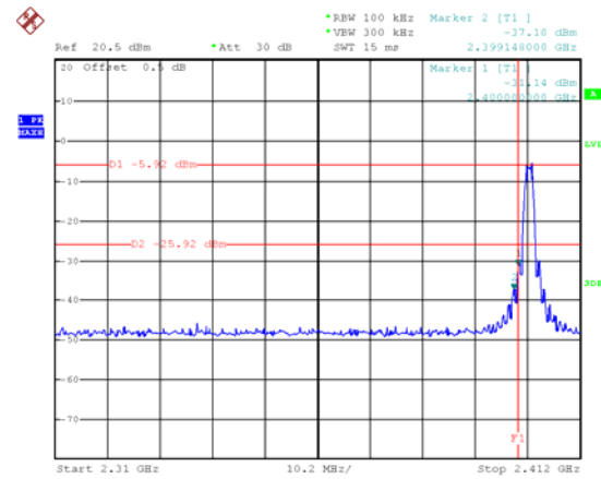
Band edge-left side
