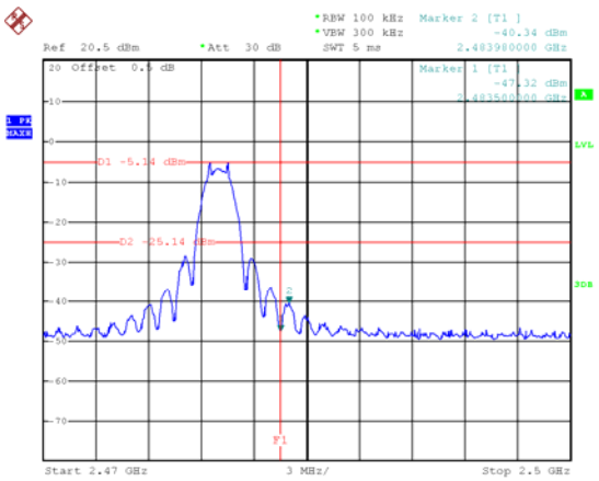
Band edge-right side
