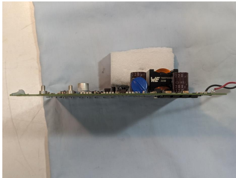
Photograph 8: Side 1 of the PCB
