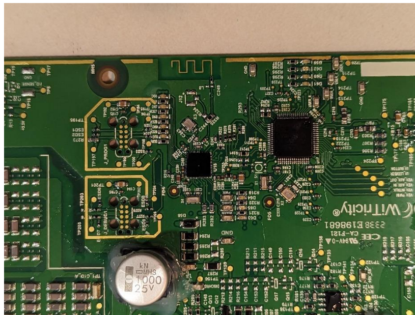
Photograph 7: Closeup View of the RF Circuitry
