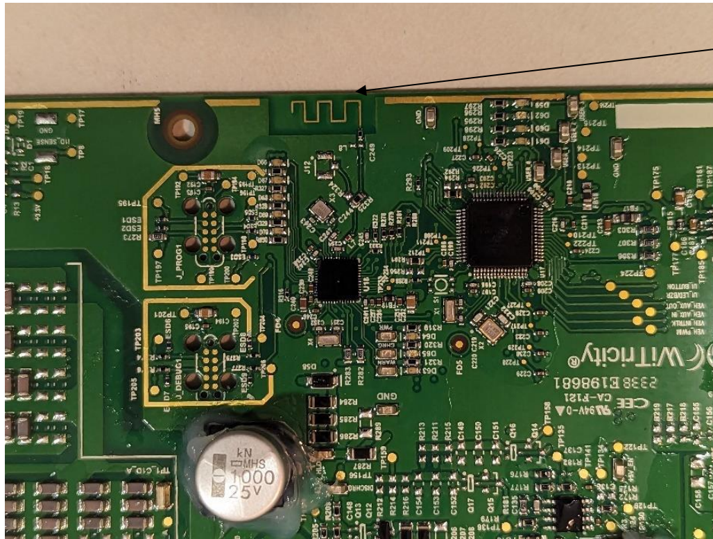
Photograph 3 – Close-up view of RF section
