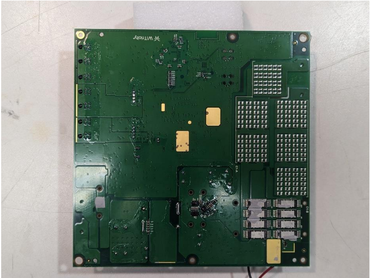
Photograph 2 – Back View of the PCBA
