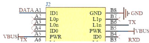
Figure 2 Android Type-C interface circuit
