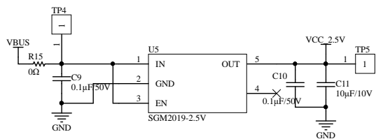
2.5V_LDO电路
