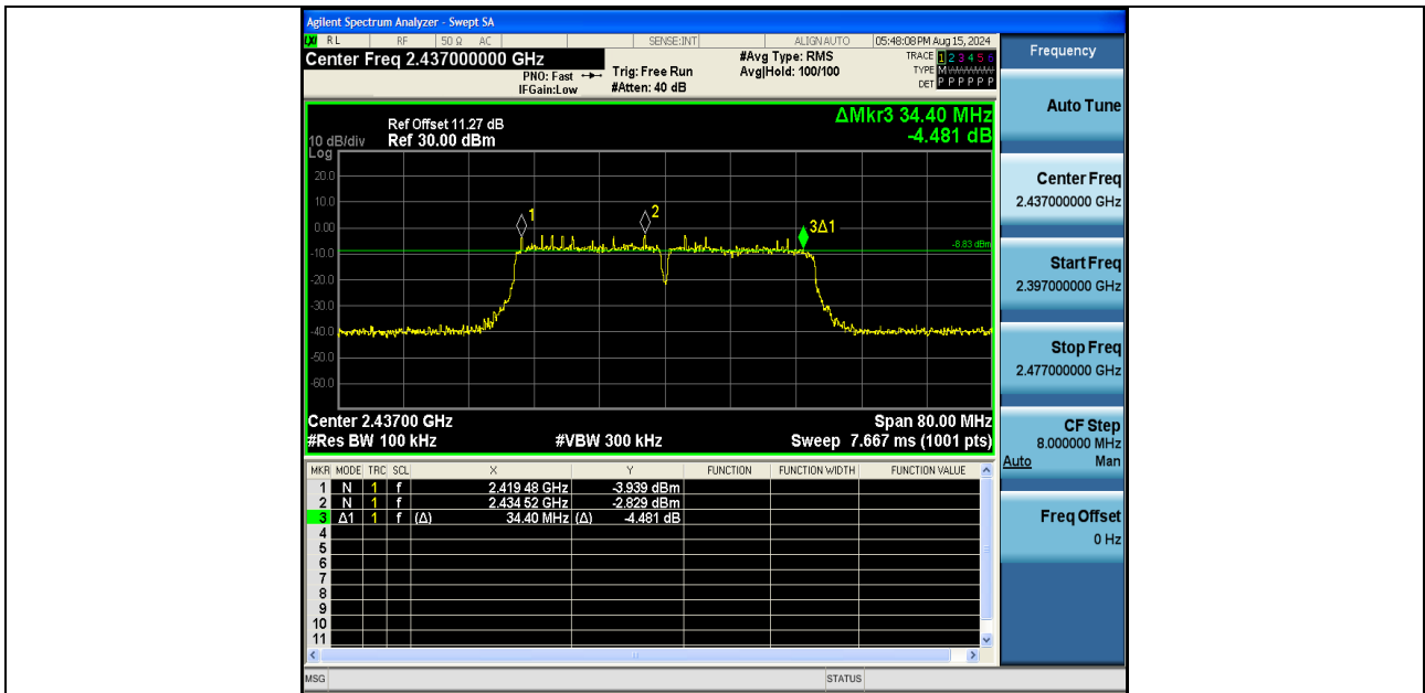
11N40SISO-Ant2-2437-PASS
