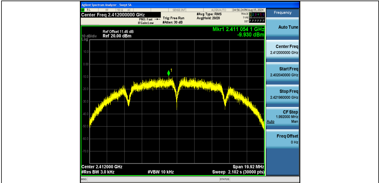
11B-Ant2-2412-PASS
