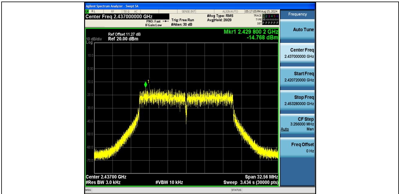
11G-Ant2-2437-PASS
