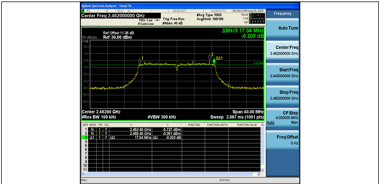
11N20SISO-Ant2-2462-PASS
