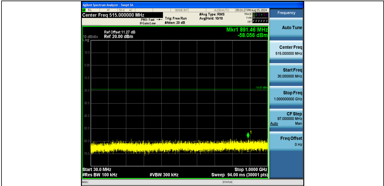
11B-Ant2-2437-30~1000-PASS
