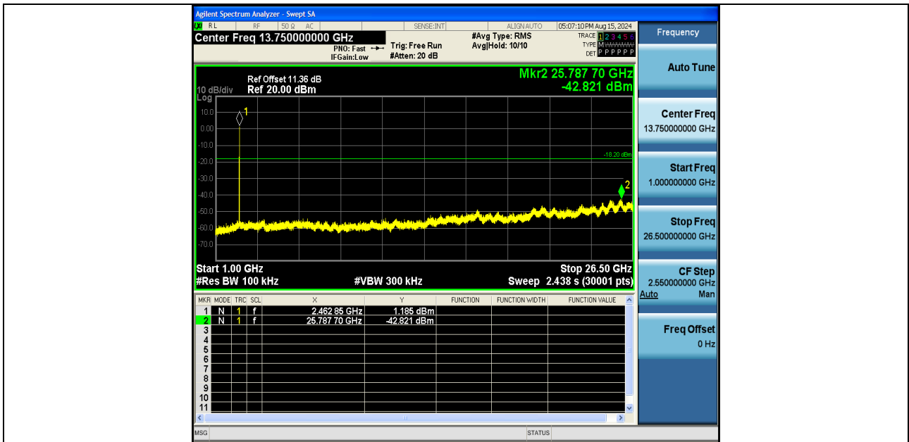
11B-Ant2-2462-1000~26500-PASS
