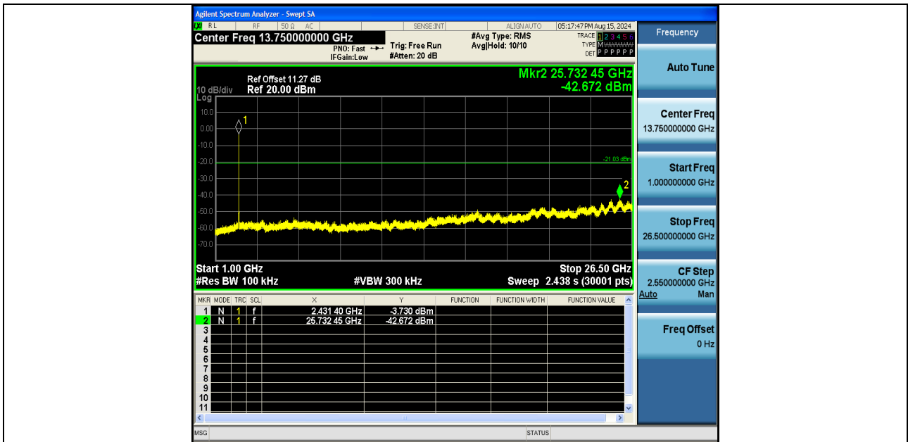
11G-Ant2-2437-1000~26500-PASS
