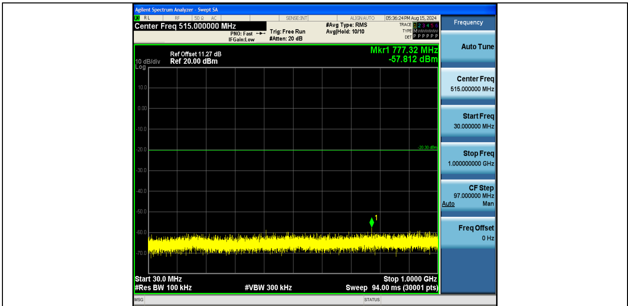
11N20SISO-Ant2-2437-30~1000-PASS
