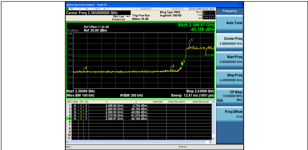
11N40SISO-Ant2-2422-PASS
