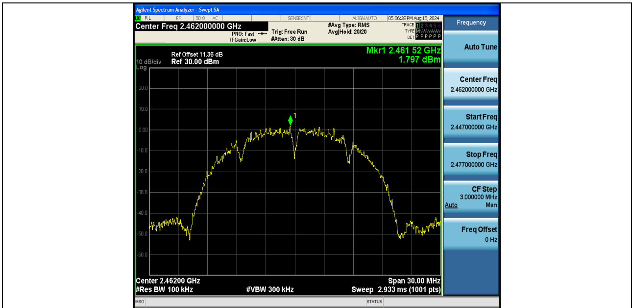
11B-Ant2-2462-0~Reference-PASS
