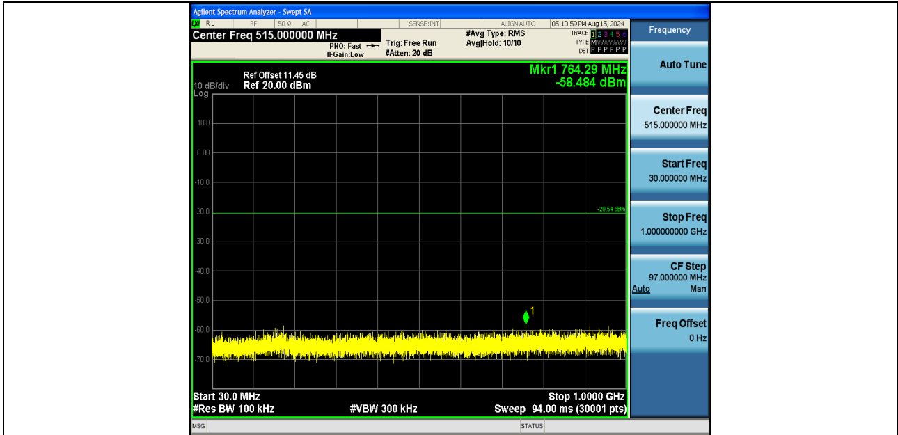
11G-Ant2-2412-30~1000-PASS
