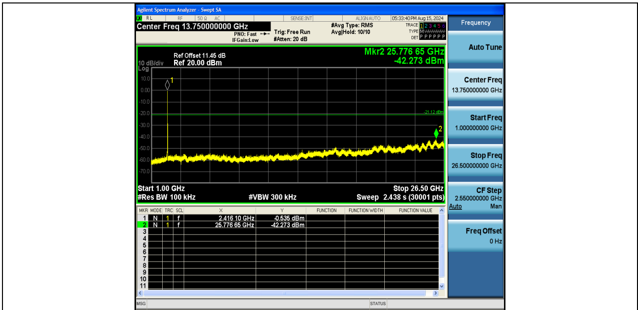
11N20SISO-Ant2-2412-1000~26500-PASS
