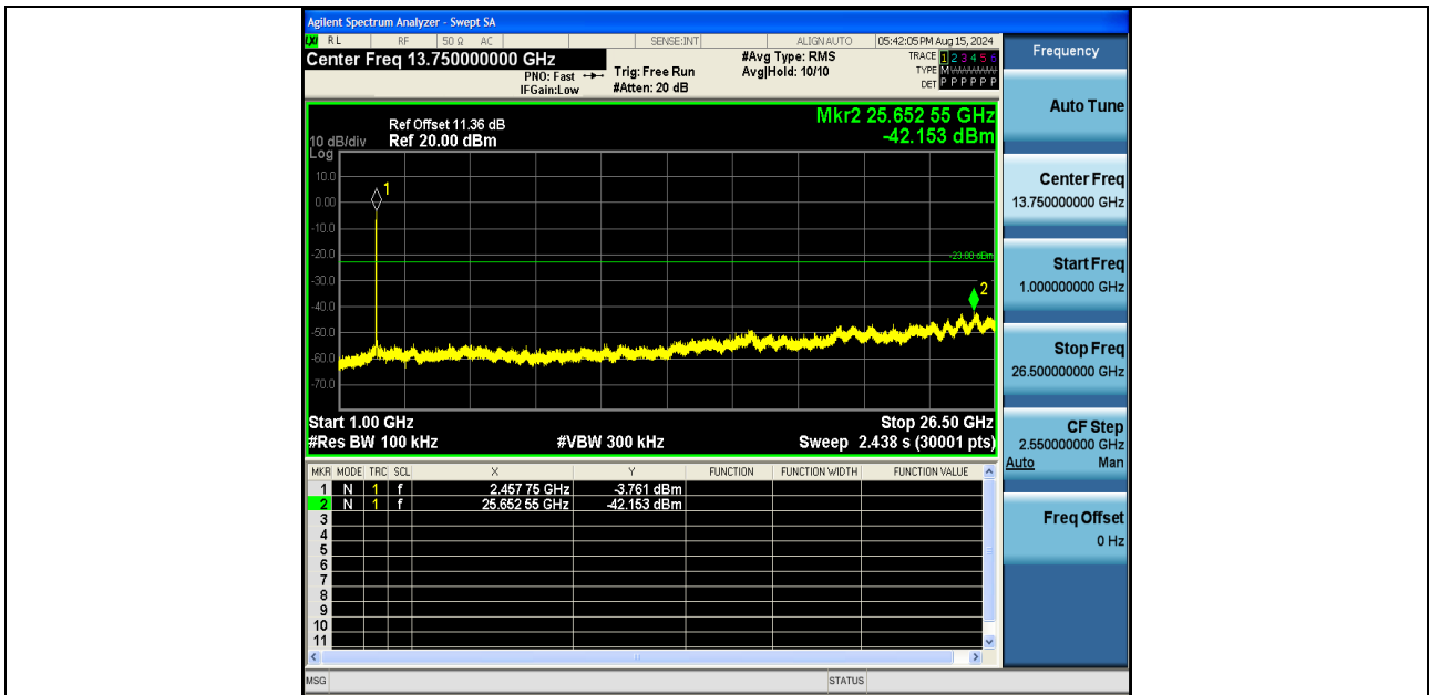
11N20SISO-Ant2-2462-1000~26500-PASS
