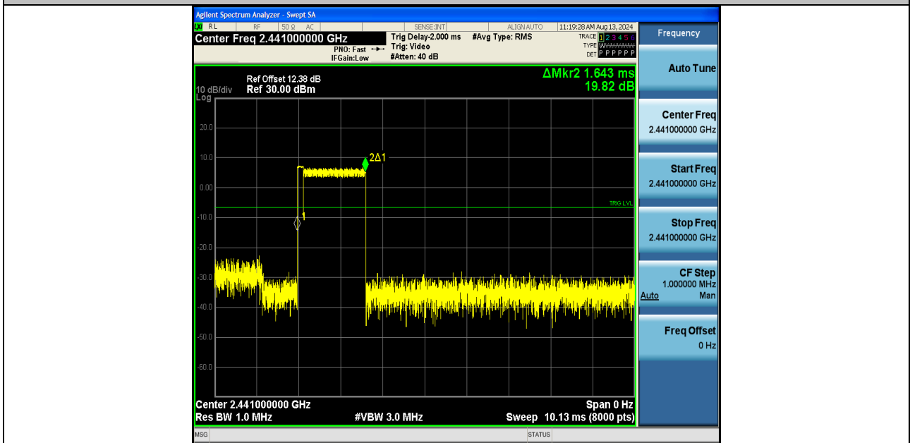
2DH3-Ant1-Hop-PASS
