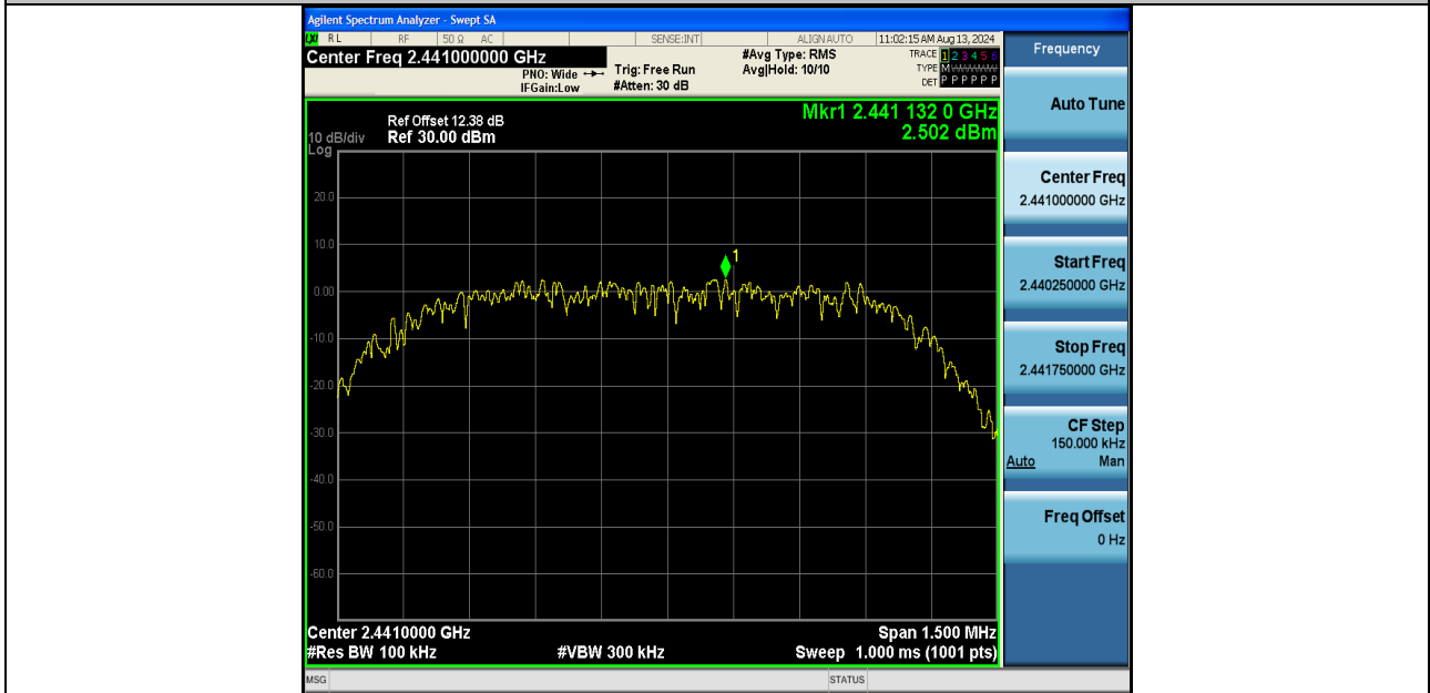
3DH5-Ant1-2441-0~Reference-PASS
