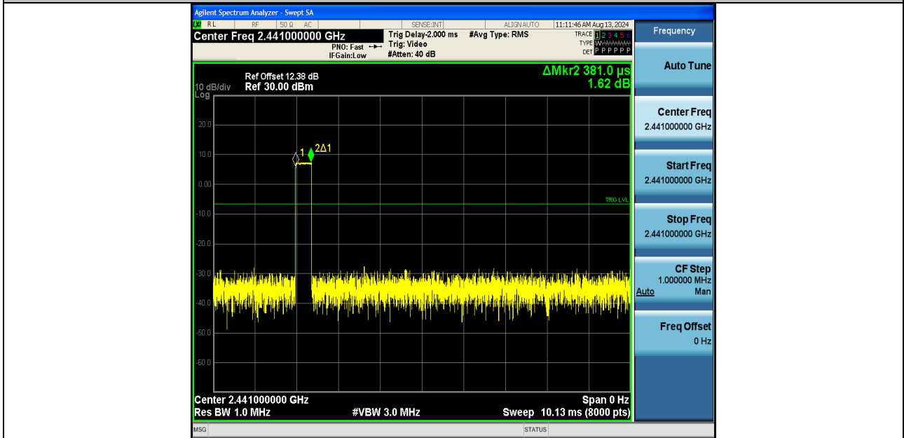
DH1-Ant1-Hop-PASS
