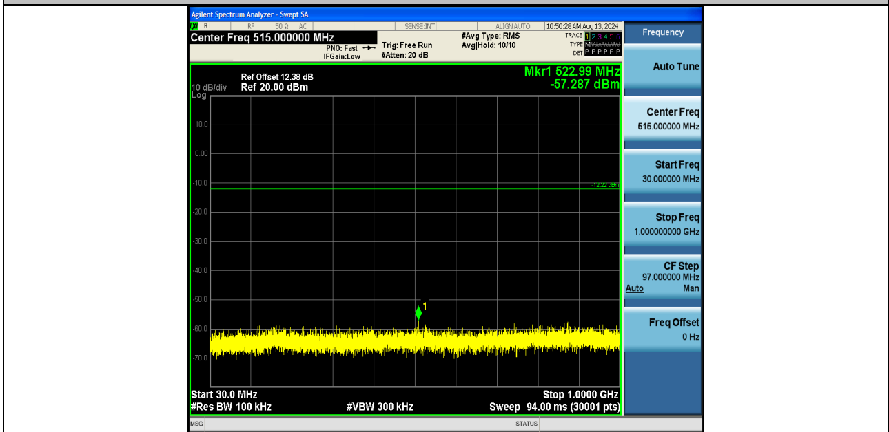
2DH5-Ant1-2441-30~1000-PASS
