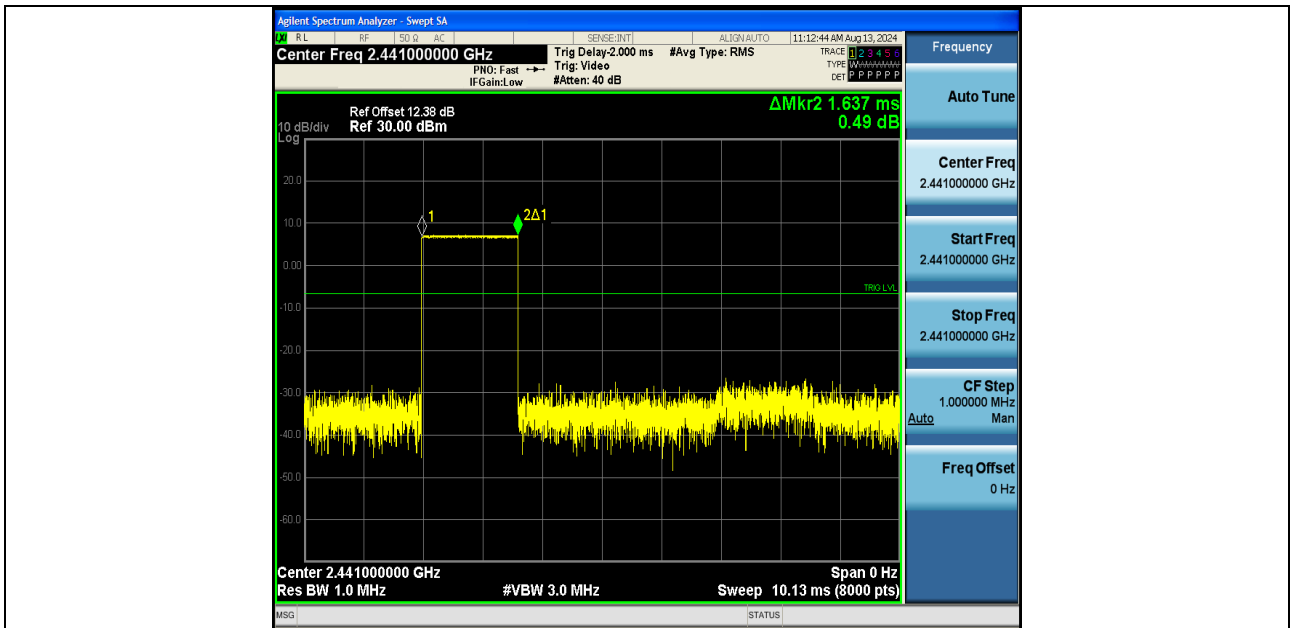
DH3-Ant1-Hop-PASS
