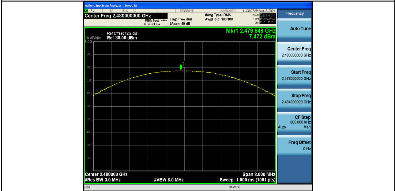
2DH5-Ant1-2480-PASS
