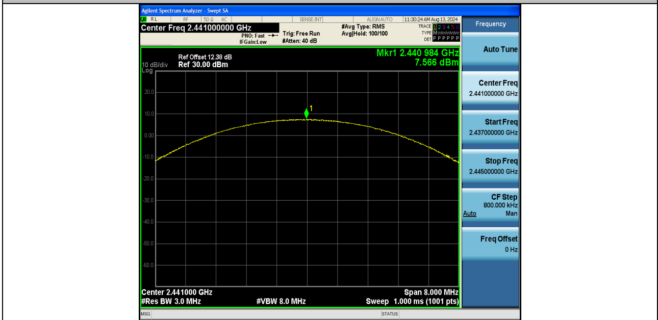
3DH5-Ant1-2441-PASS
