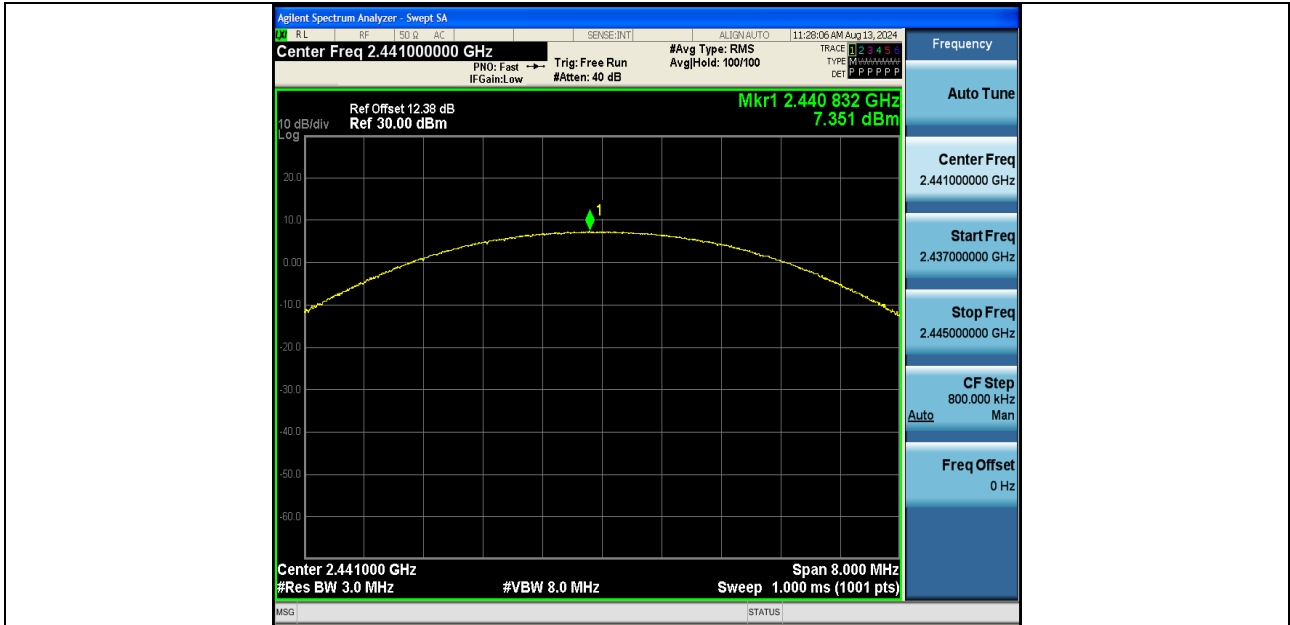
2DH5-Ant1-2441-PASS
