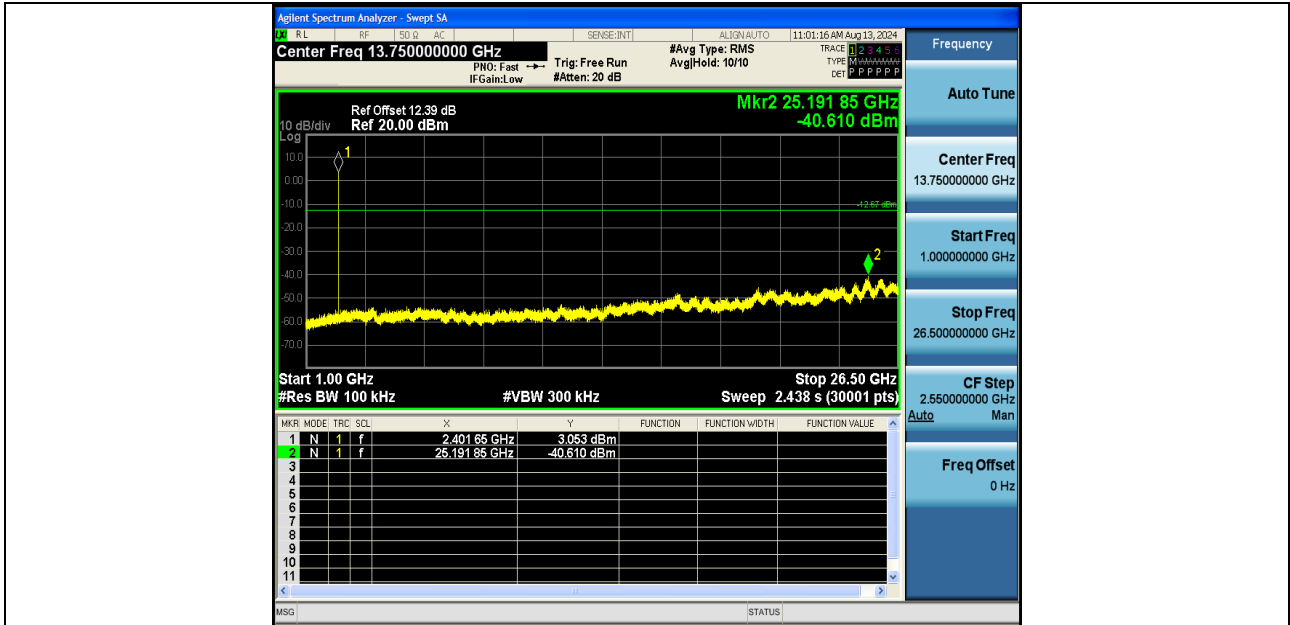
3DH5-Ant1-2402-1000~26500-PASS
