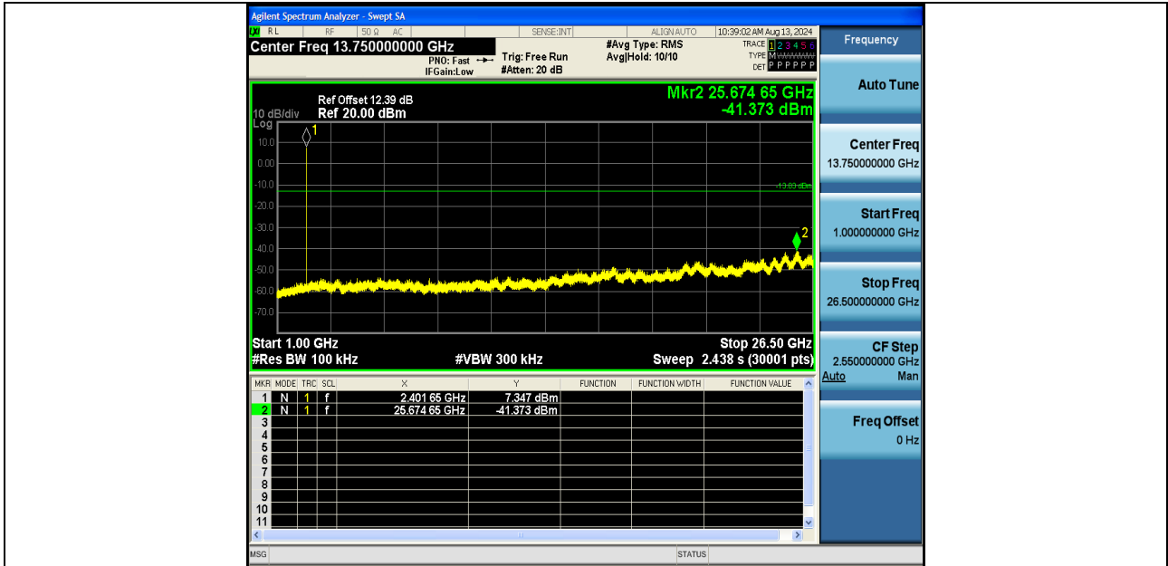
DH5-Ant1-2402-1000~26500-PASS
