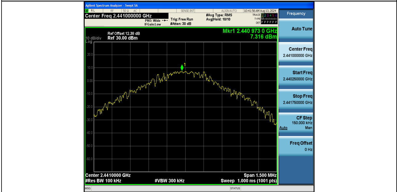
DH5-Ant1-2441-0~Reference-PASS
