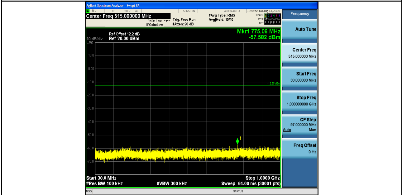
DH5-Ant1-2480-30~1000-PASS
