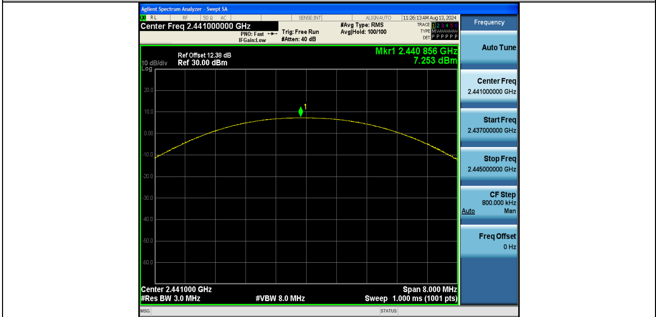
DH5-Ant1-2441-PASS
