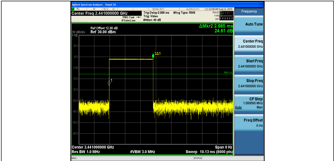
DH5-Ant1-Hop-PASS
