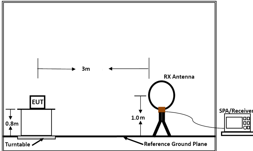
Below 30MHz
