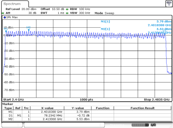
EDR (8DPSK): Number of Hopping Channels
