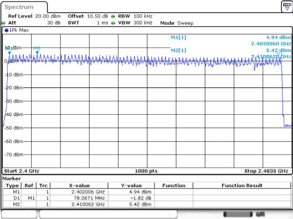
EDR (π/4-DQPSK): Number of Hopping Channels
