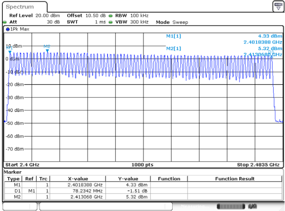
BDR (GFSK):Number of Hopping Channels
