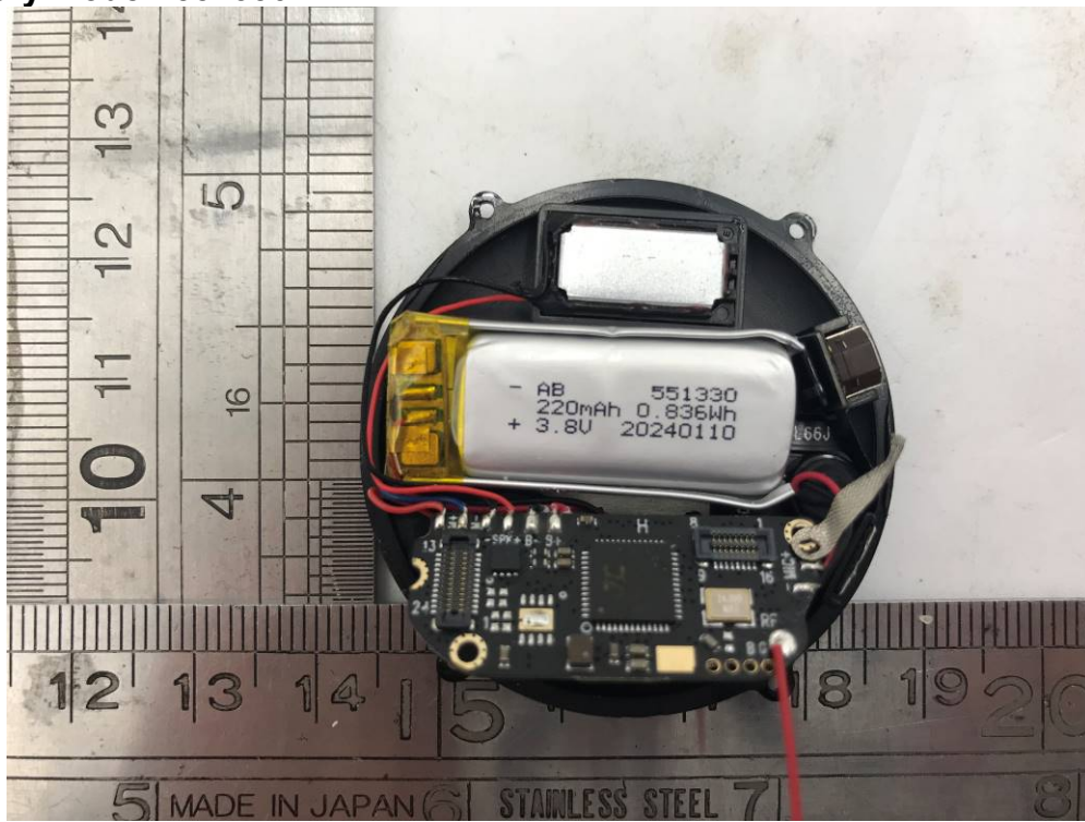
Battery Model: 551330
