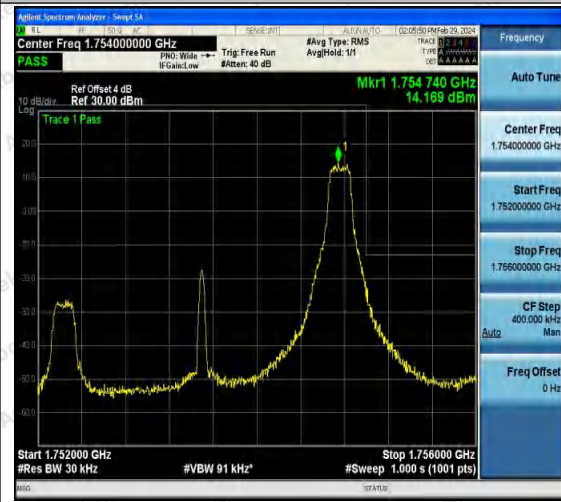
Band4_3MHz_16QAM_20385_1RB#14
