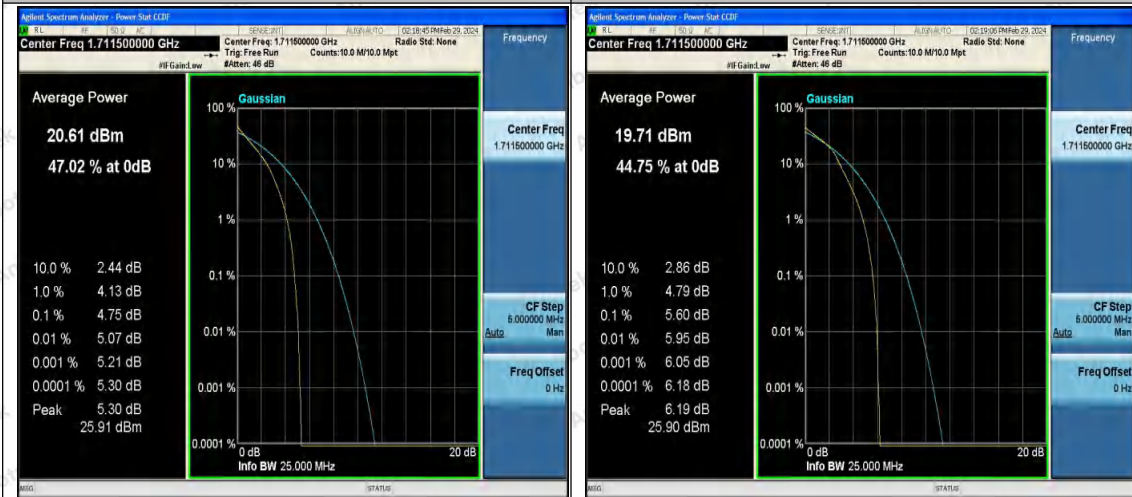
Band4-3MHz-QPSK-19965-15RB#0-PASS
