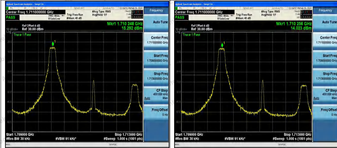
Band4_3MHz_QPSK_19965_1RB#0
