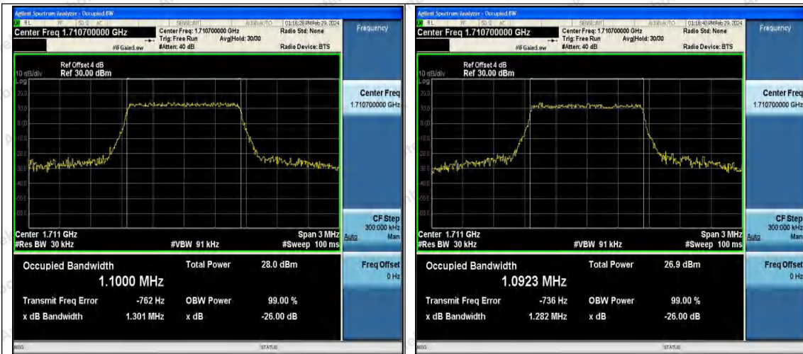
Band4-1.4MHz-QPSK-19957-6RB#0-PASS
