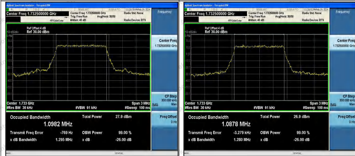
Band4-1.4MHz-QPSK-20175-6RB#0-PASS
