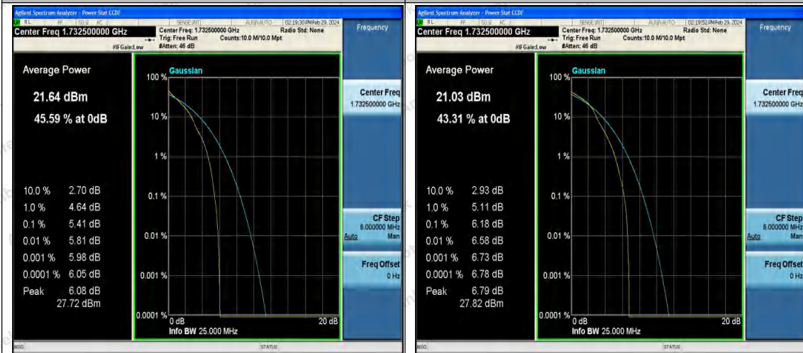
Band4-3MHz-QPSK-20175-1RB#0-PASS
