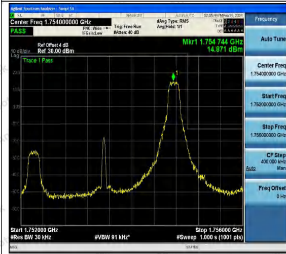
Band4_3MHz_QPSK_20385_1RB#14
