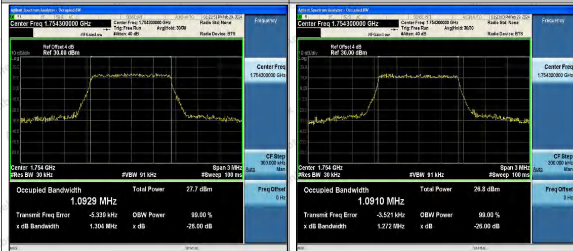
Band4-1.4MHz-QPSK-20393-6RB#0-PASS
