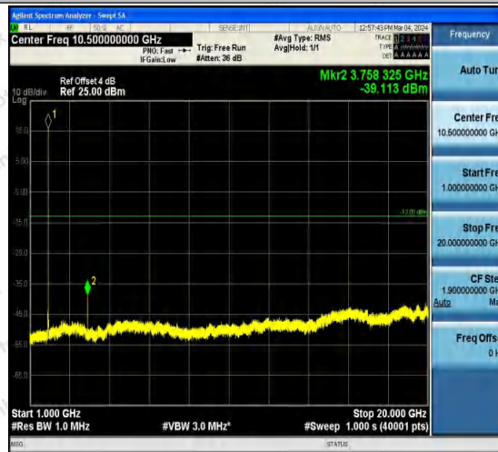
Band2-9400-1-1000~20000MHz-PASS
