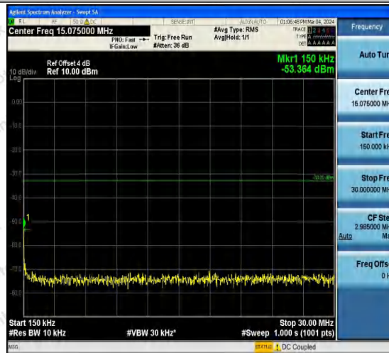
Band2-9262-5-0.15~30MHz-PASS
