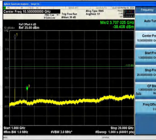
Band2-9262-5-1000~20000MHz-PASS
