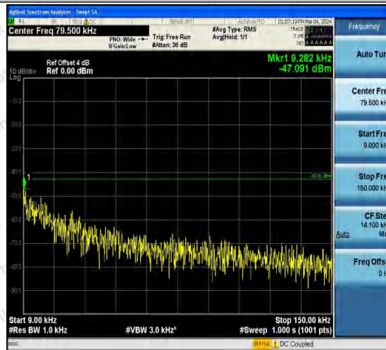
Band2-9400-5-0.009~0.15MHz-PASS
