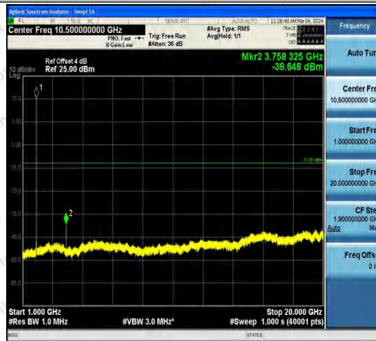
Band2-9400-4-1000~20000MHz-PASS
