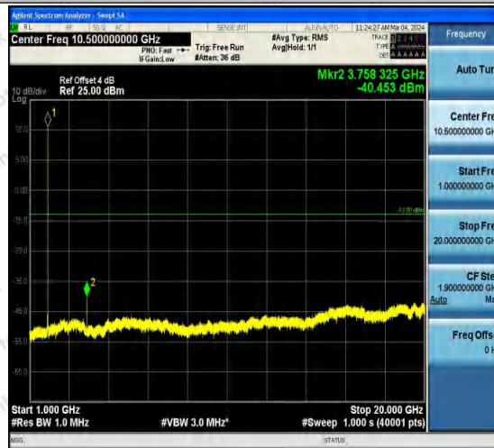
Band2-9400-2-1000~20000MHz-PASS
