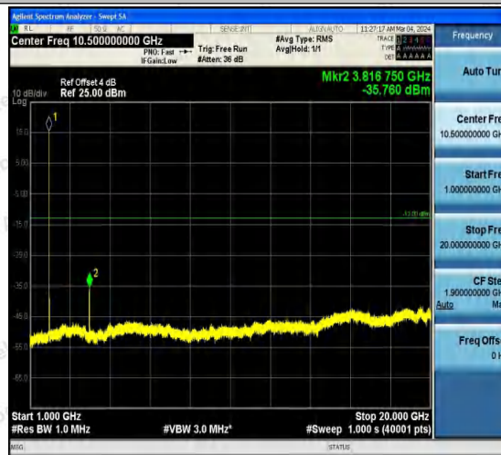
Band2-9538-3-1000~20000MHz-PASS
