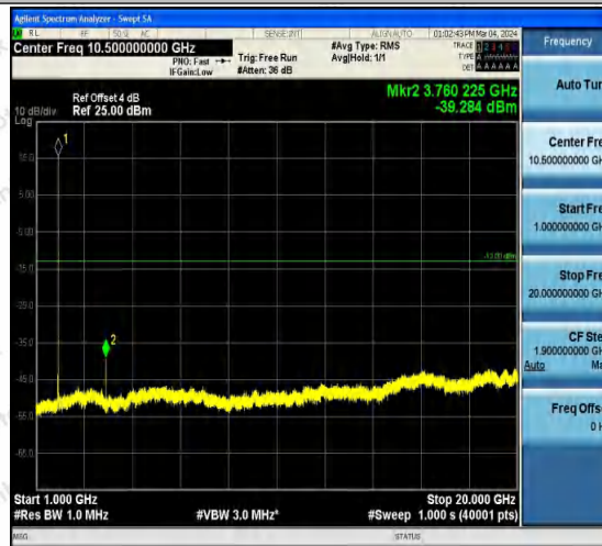
Band2-9400-3-1000~20000MHz-PASS
