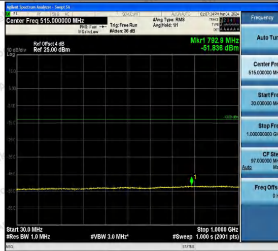
Band2-9400-5-30~1000MHz-PASS
