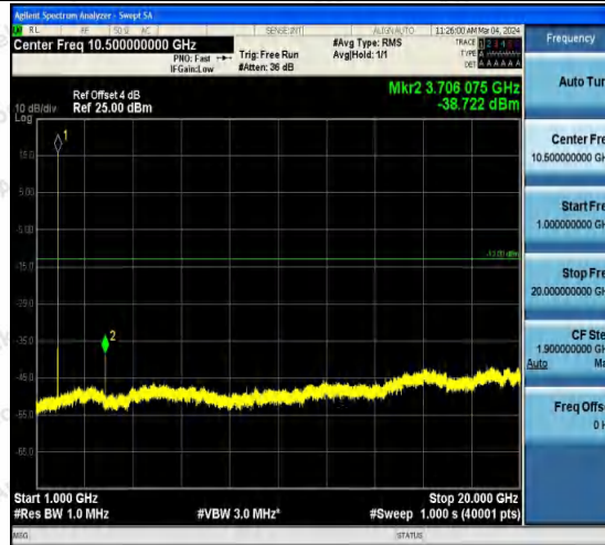
Band2-9262-3-1000~20000MHz-PASS
