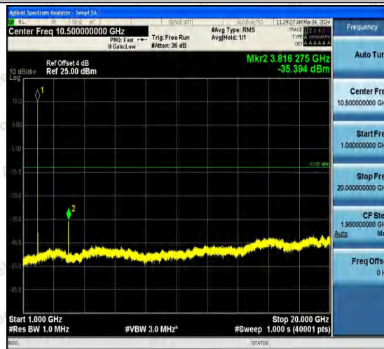
Band2-9538-4-1000~20000MHz-PASS
