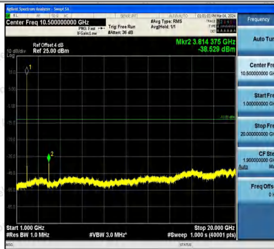
Band2-9538-2-1000~20000MHz-PASS
