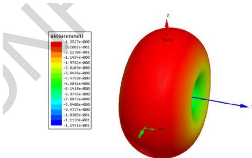
3D Gain Diagram:
