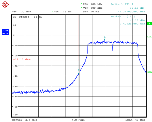
n20_2412MHz_Chain 0
