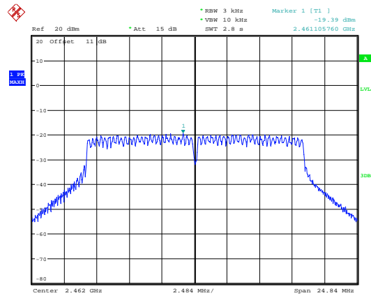
g_2462MHz_Chain 0
