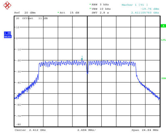
g_2412MHz_Chain 0
