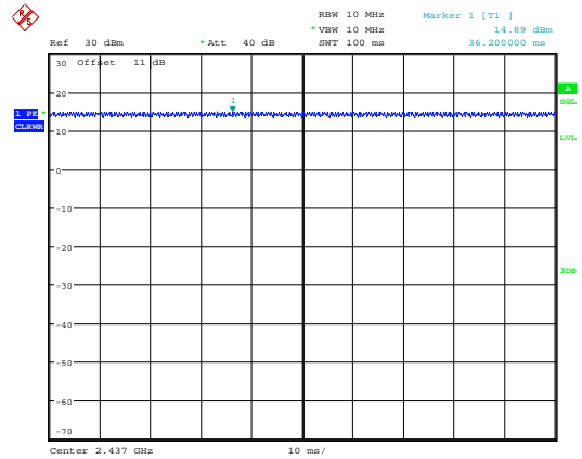
g_2437MHz_Chain 0
