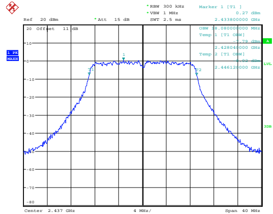
n20_2437MHz_Chain 0
