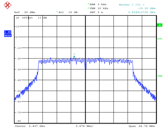
n20_2437MHz_Chain 0
