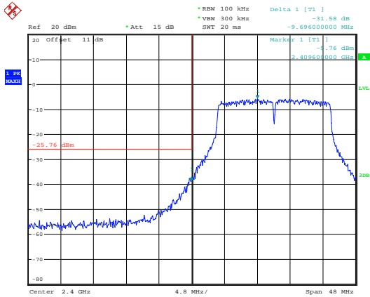
g_2412MHz_Chain 0
