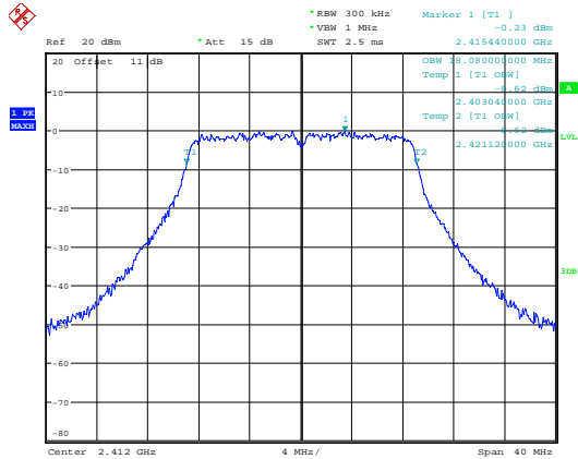
n20_2412MHz_Chain 0
