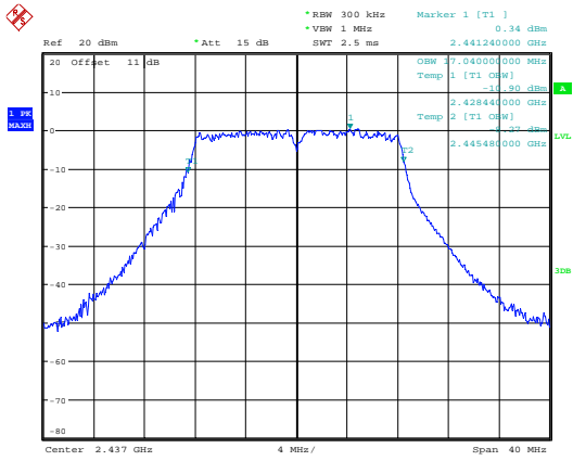
g_2437MHz_Chain 0
