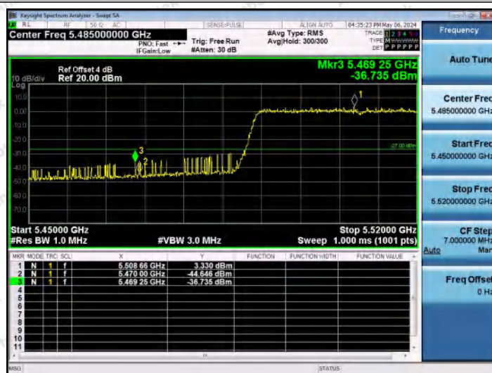
11AX40MIMO-Ant0-5510-PASS
