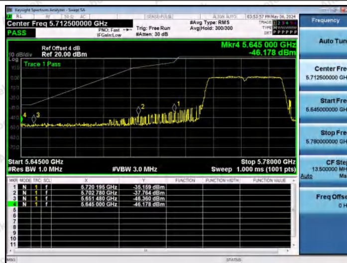
11AC40MIMO-Ant0-5755-PASS
