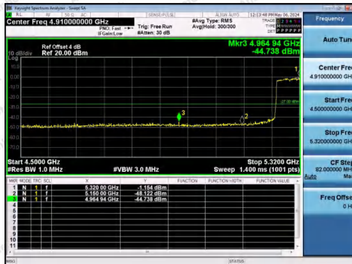
11AC80MIMO-Ant1-5290-PASS
