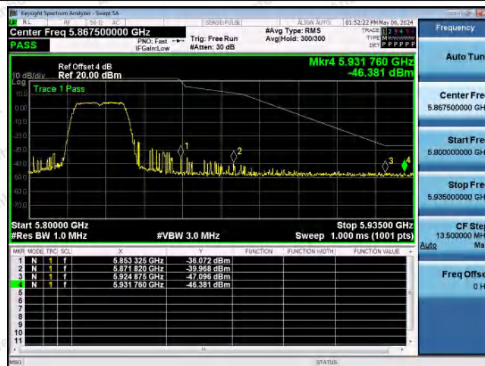
11AC20MIMO-Ant1-5825-PASS
