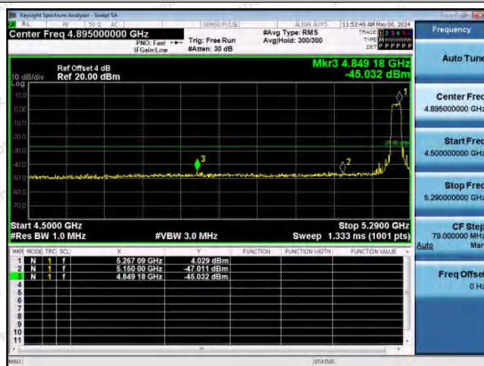
11AC20MIMO-Ant1-5260-PASS
