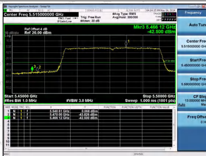
11AC80MIMO-Ant0-5530-PASS
