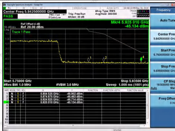
11AX80MIMO-Ant0-5775-PASS
