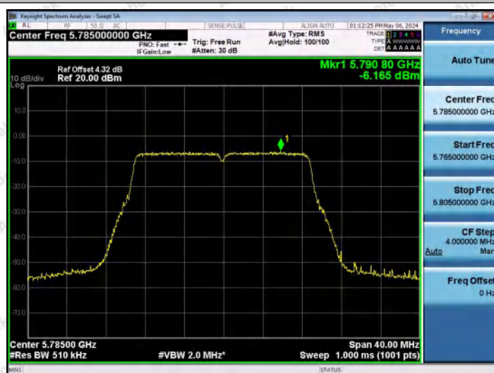
11N20MIMO-Ant1-5785-PASS
