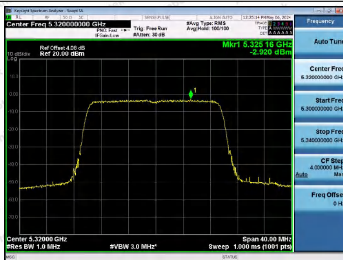
11AX20MIMO-Ant1-5320-PASS
