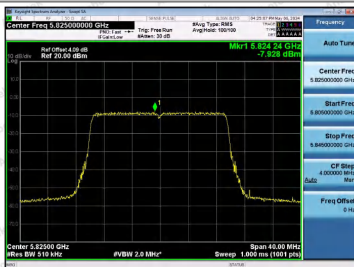
11AX20MIMO-Ant1-5825-PASS
