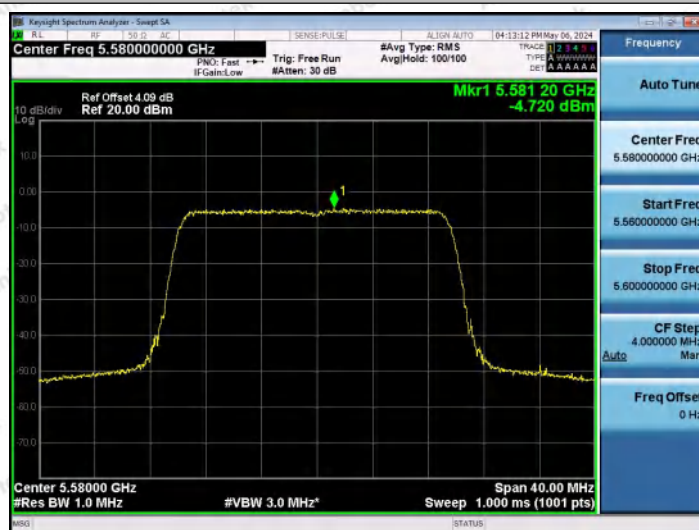
11AX20MIMO-Ant0-5580-PASS
