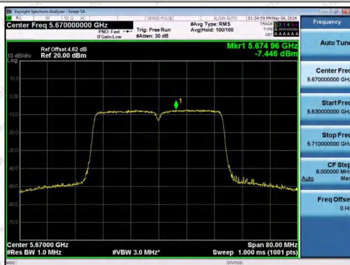
11N40MIMO-Ant1-5670-PASS
