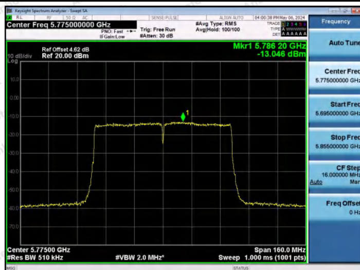
11AC80MIMO-Ant0-5775-PASS
