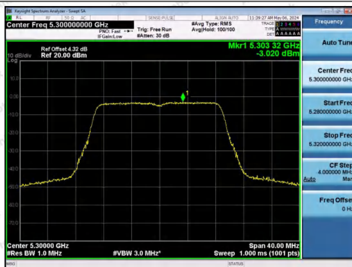
11N20MIMO-Ant0-5300-PASS
