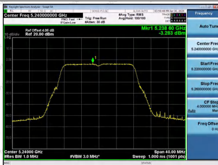
11A-Ant1-5240-PASS
