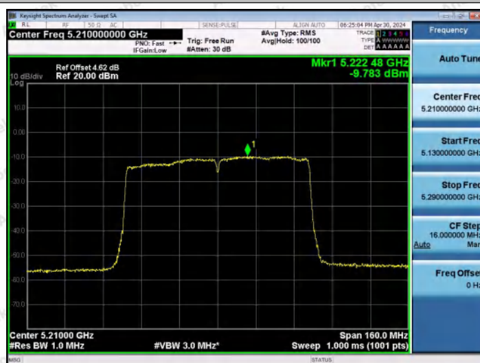
11AC80MIMO-Ant0-5210-PASS
