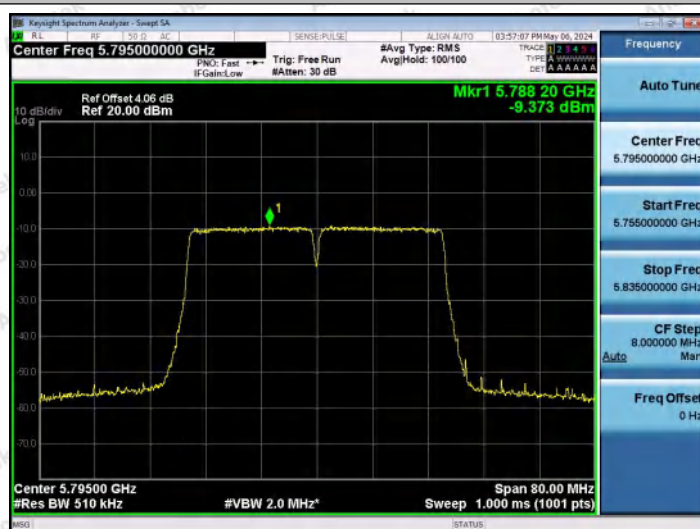
11AC40MIMO-Ant0-5795-PASS
