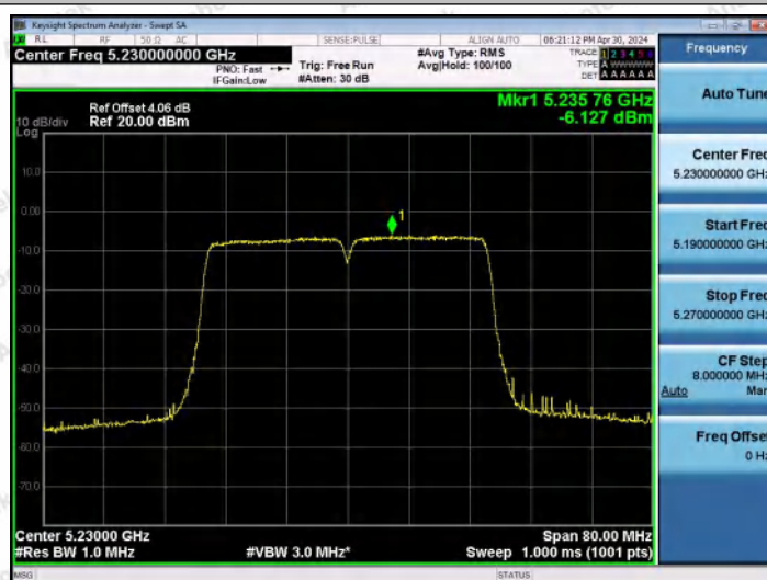
11AC40MIMO-Ant0-5230-PASS
