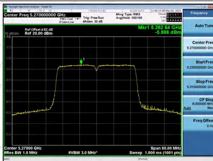
11N40MIMO-Ant1-5270-PASS
