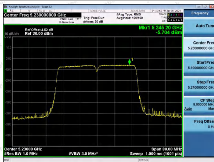
11N40MIMO-Ant0-5230-PASS
