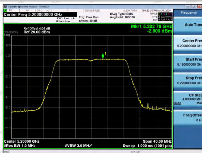
11AC20MIMO-Ant0-5200-PASS
