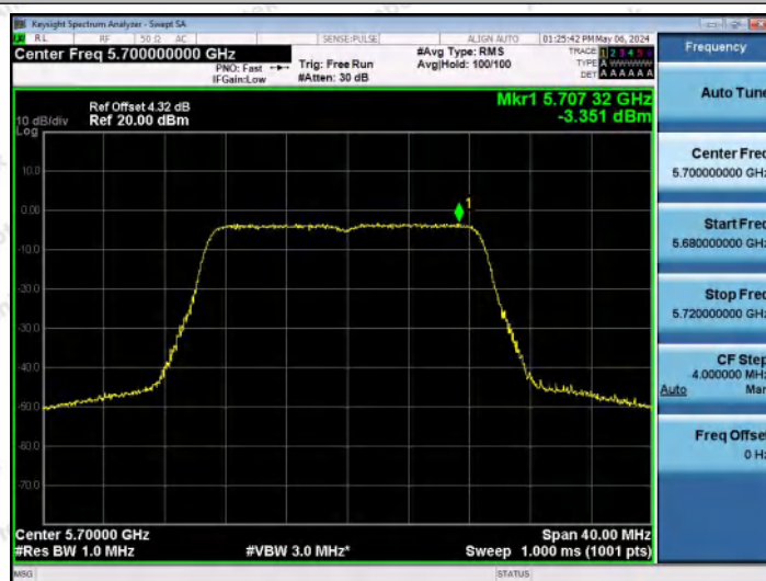
11N20MIMO-Ant1-5700-PASS
