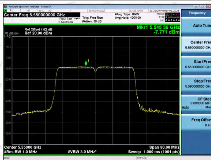
11N40MIMO-Ant1-5550-PASS
