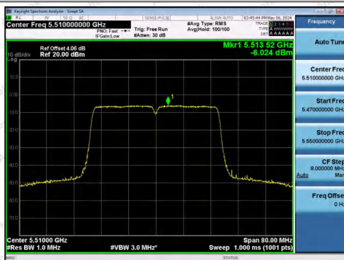
11AC40MIMO-Ant0-5510-PASS
