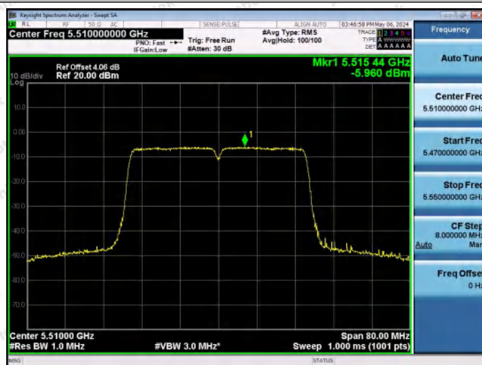
11AC40MIMO-Ant1-5510-PASS
