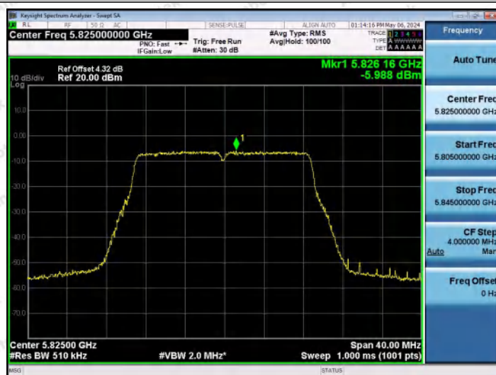
11N20MIMO-Ant0-5825-PASS
