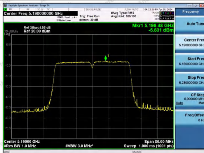
11N40MIMO-Ant0-5190-PASS
