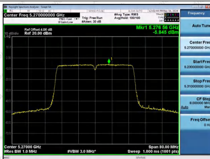
11AC40MIMO-Ant1-5270-PASS
