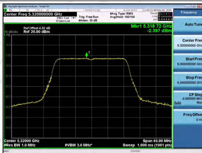
11N20MIMO-Ant1-5320-PASS
