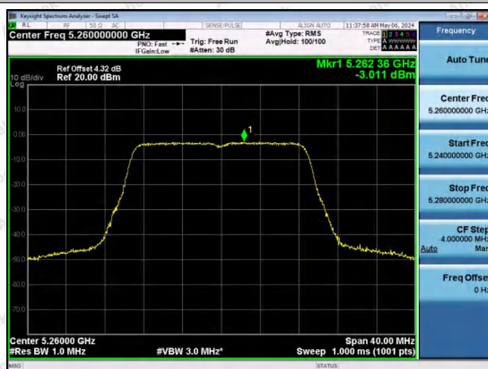
11N20MIMO-Ant1-5260-PASS
