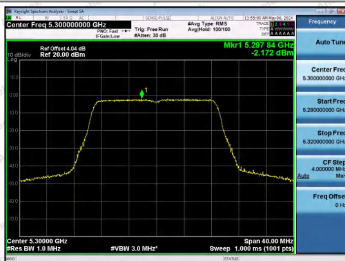
11AC20MIMO-Ant0-5300-PASS
