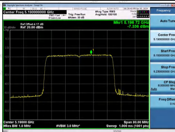
11AX40MIMO-Ant0-5190-PASS
