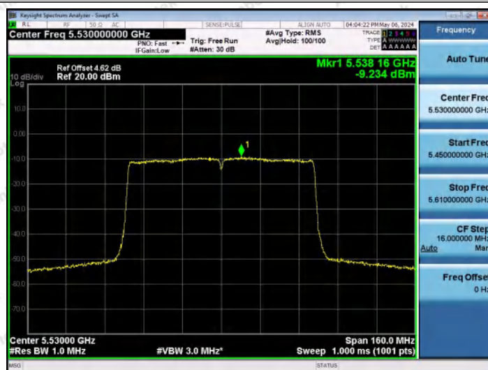
11AC80MIMO-Ant0-5530-PASS
