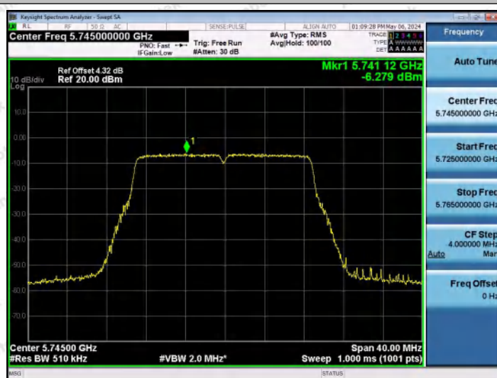
11N20MIMO-Ant1-5745-PASS
