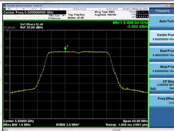
11N20MIMO-Ant1-5500-PASS
