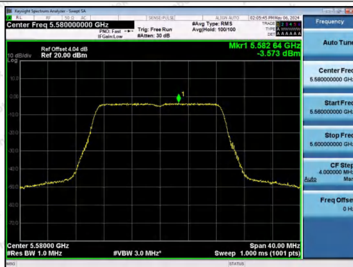
11AC20MIMO-Ant1-5580-PASS
