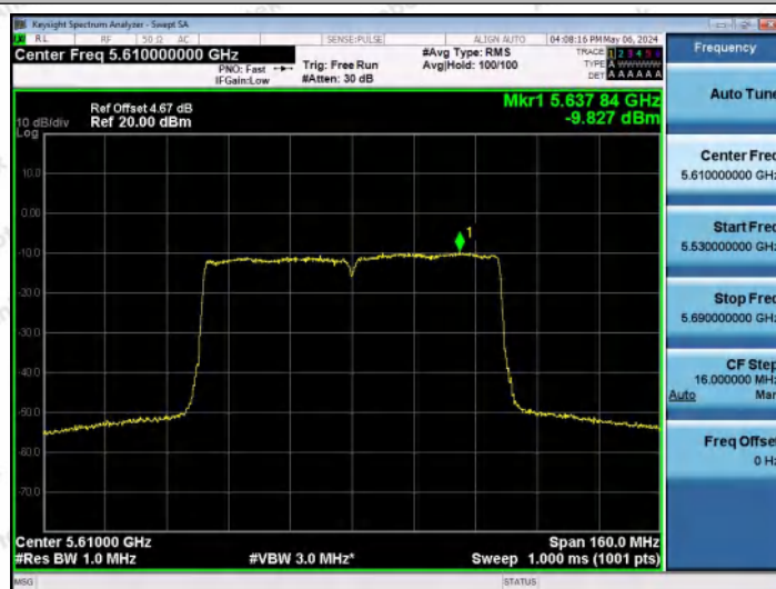
11AC80MIMO-Ant1-5610-PASS
