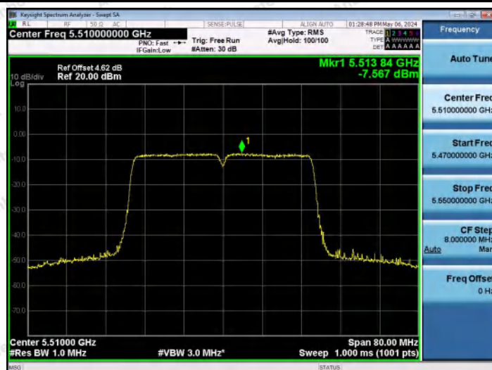
11N40MIMO-Ant1-5510-PASS
