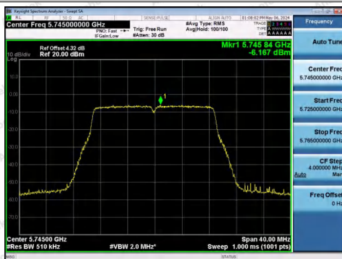
11N20MIMO-Ant0-5745-PASS
