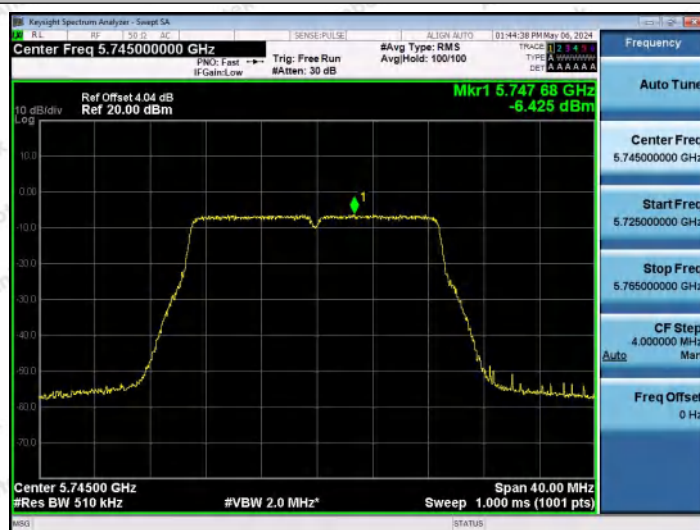
11AC20MIMO-Ant0-5745-PASS
