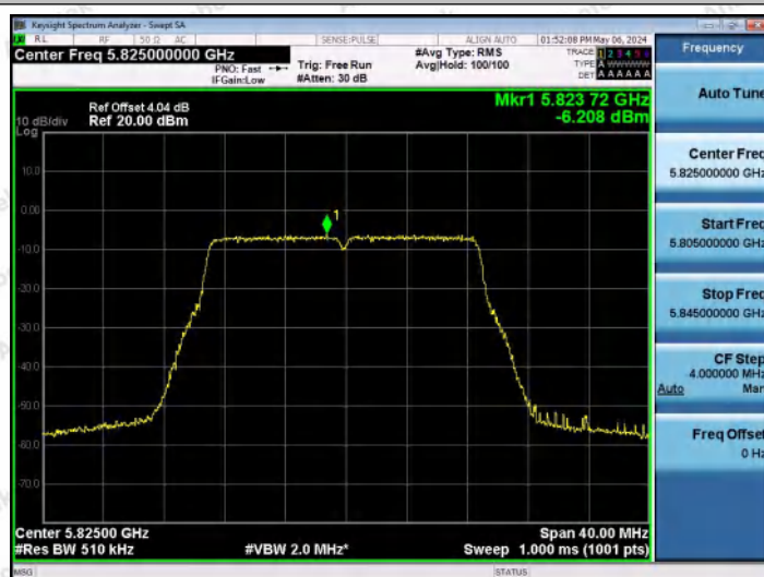
11AC20MIMO-Ant1-5825-PASS
