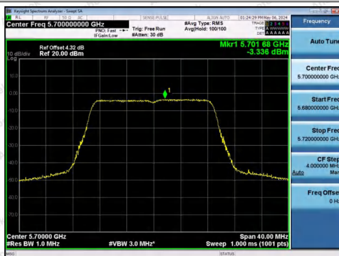
11N20MIMO-Ant0-5700-PASS
