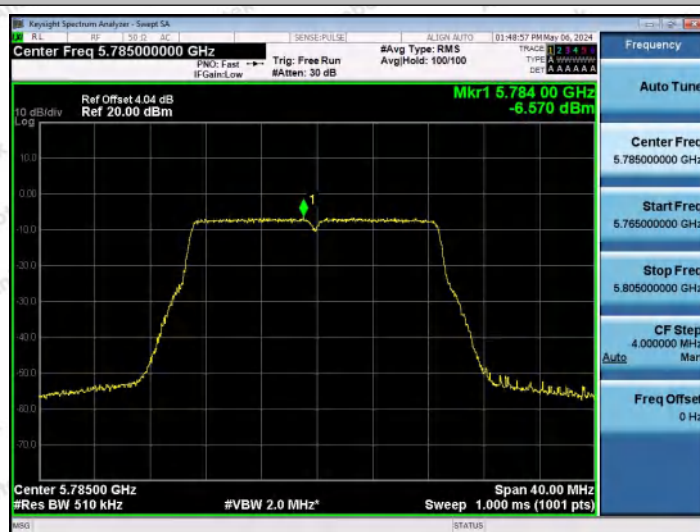
11AC20MIMO-Ant1-5785-PASS
