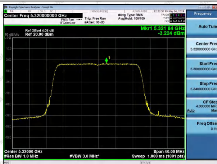
11AX20MIMO-Ant0-5320-PASS
