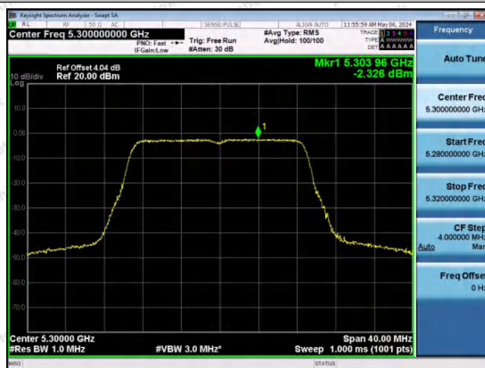
11AC20MIMO-Ant1-5300-PASS
