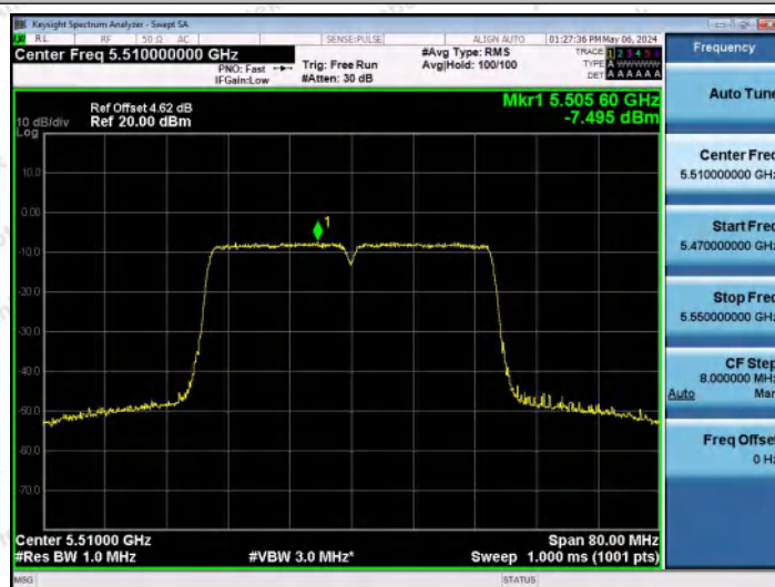
11N40MIMO-Ant0-5510-PASS
