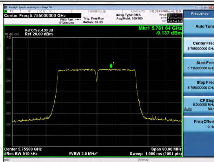
11AC40MIMO-Ant0-5755-PASS
