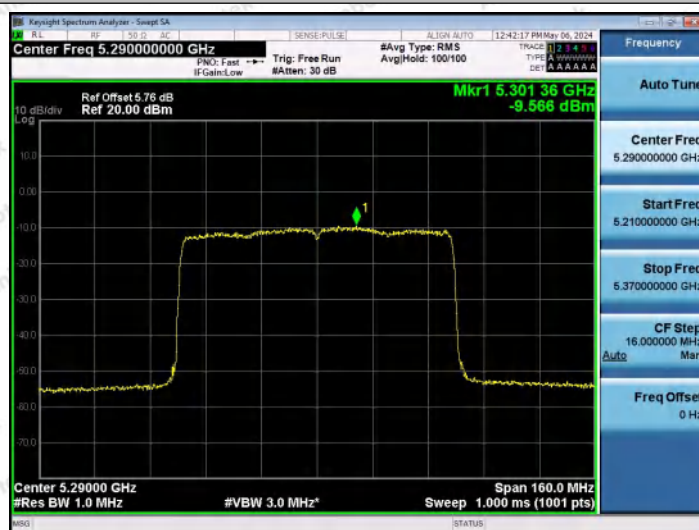
11AX80MIMO-Ant1-5290-PASS
