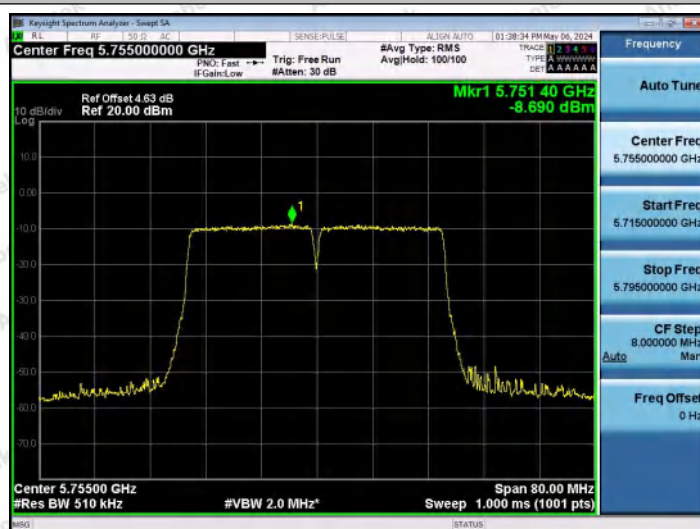
11N40MIMO-Ant0-5755-PASS
