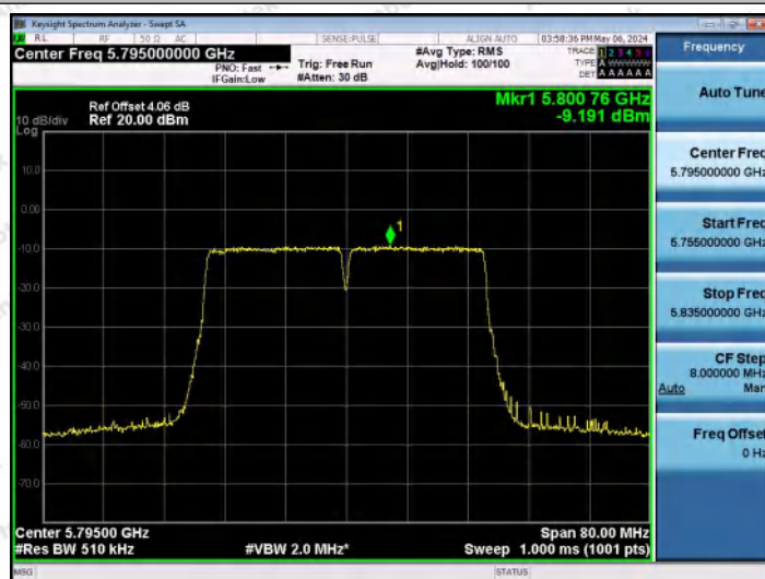
11AC40MIMO-Ant1-5795-PASS
