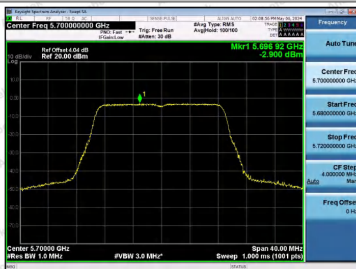
11AC20MIMO-Ant1-5700-PASS
