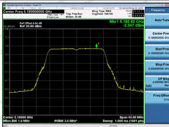
11A-Ant0-5180-PASS
