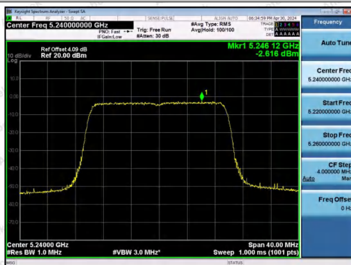
11AX20MIMO-Ant0-5240-PASS
