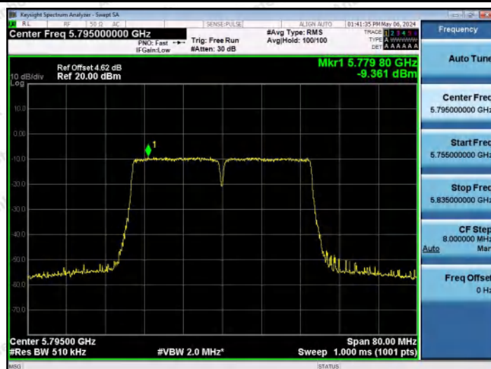
11N40MIMO-Ant0-5795-PASS
