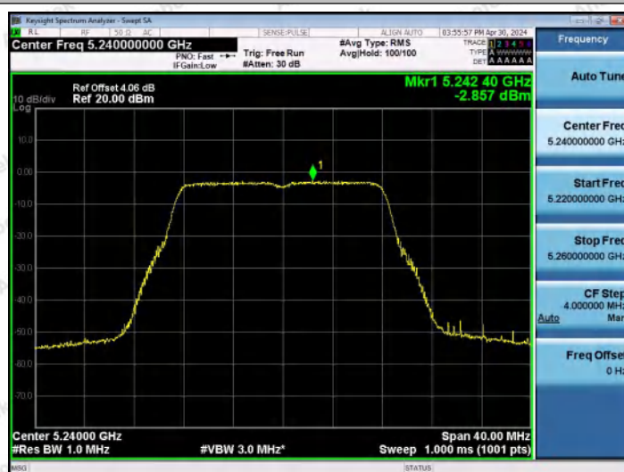
11A-Ant0-5240-PASS
