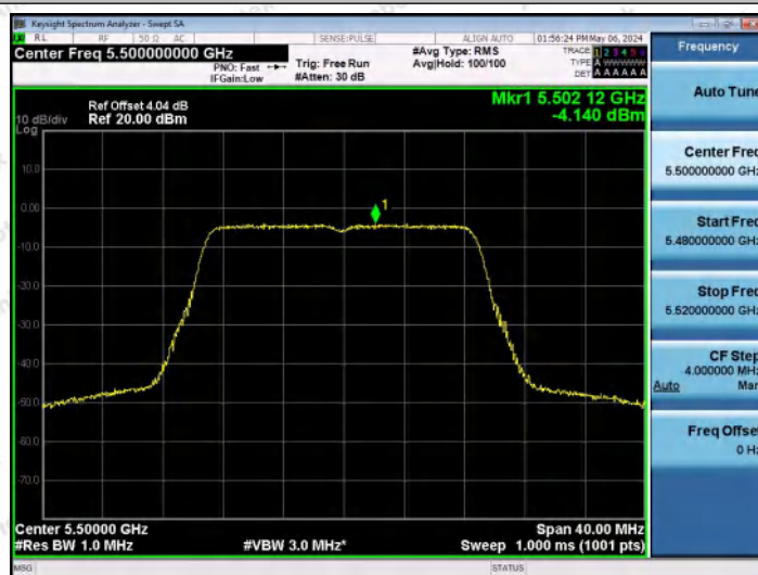
11AC20MIMO-Ant0-5500-PASS
