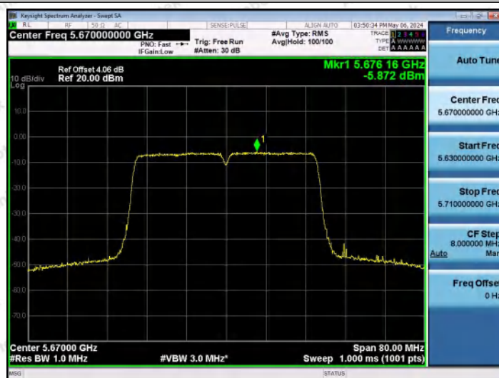
11AC40MIMO-Ant0-5670-PASS
