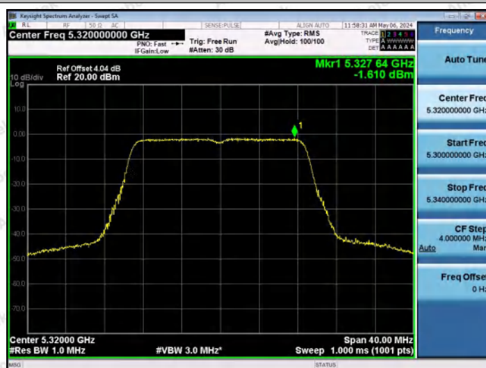
11AC20MIMO-Ant1-5320-PASS
