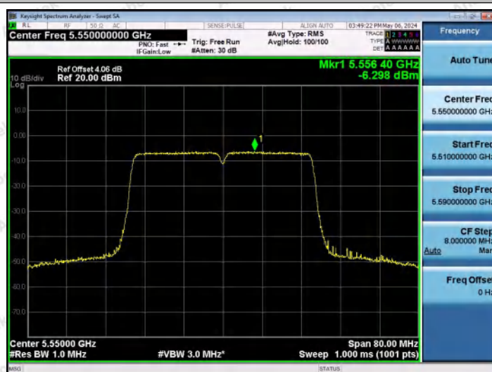
11AC40MIMO-Ant1-5550-PASS
