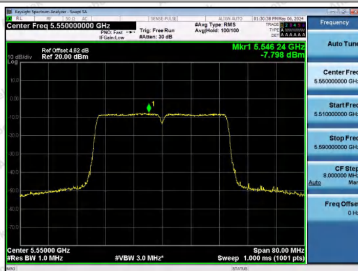
11N40MIMO-Ant0-5550-PASS
