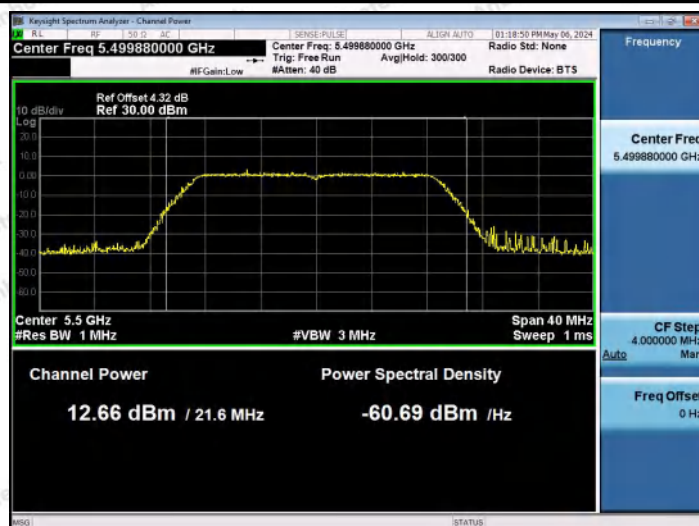
11N20MIMO-Ant0-5500-PASS
