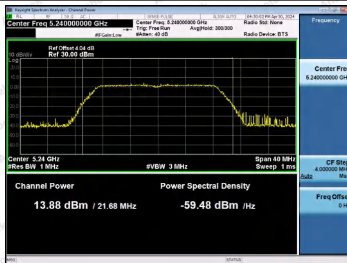
11AC20MIMO-Ant0-5240-PASS
