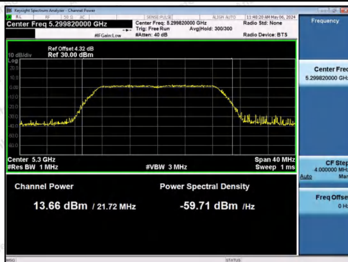
11N20MIMO-Ant1-5300-PASS
