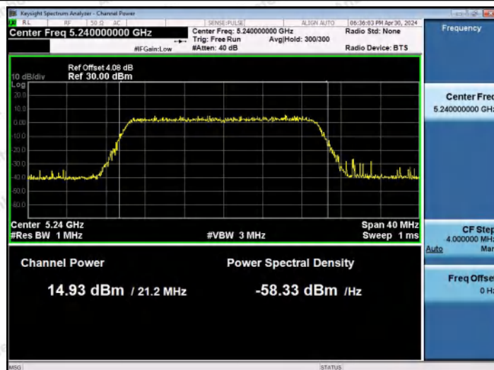
11AX20MIMO-Ant1-5240-PASS
