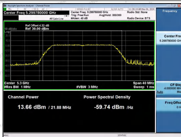
11N20MIMO-Ant0-5300-PASS
