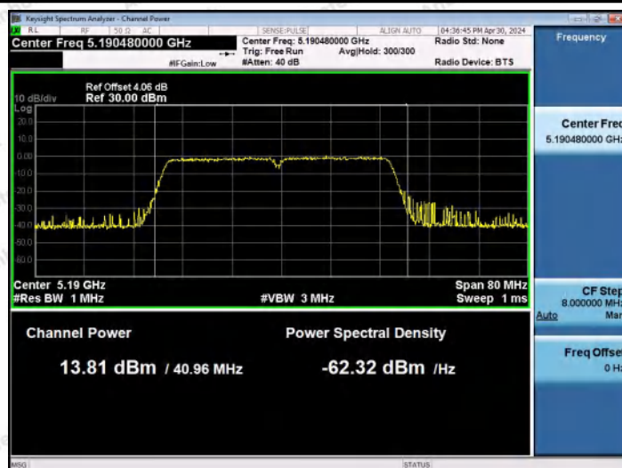
11AC40MIMO-Ant0-5190-PASS
