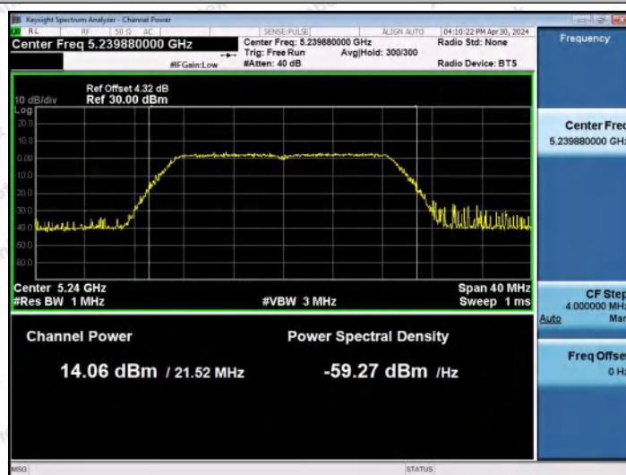
11N20MIMO-Ant1-5240-PASS
