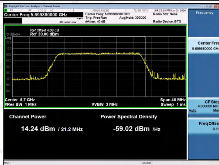
11AX20MIMO-Ant0-5700-PASS
