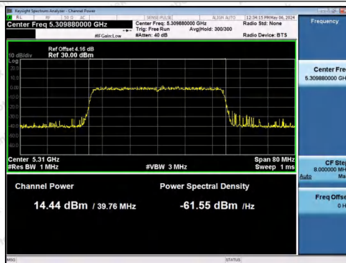
11AX40MIMO-Ant1-5310-PASS
