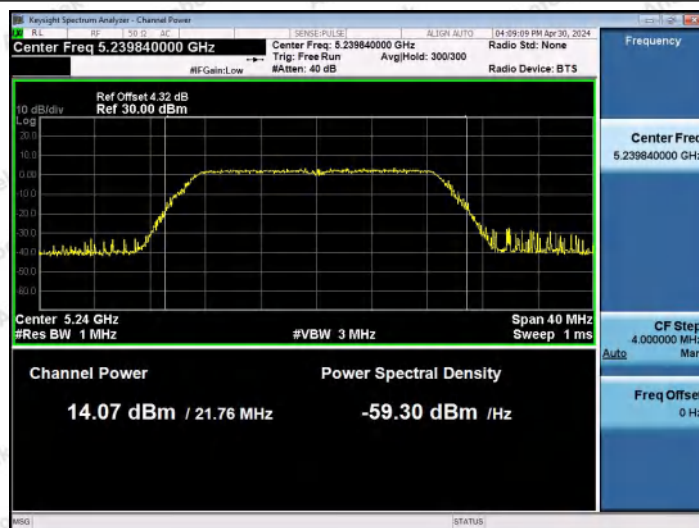
11N20MIMO-Ant0-5240-PASS
