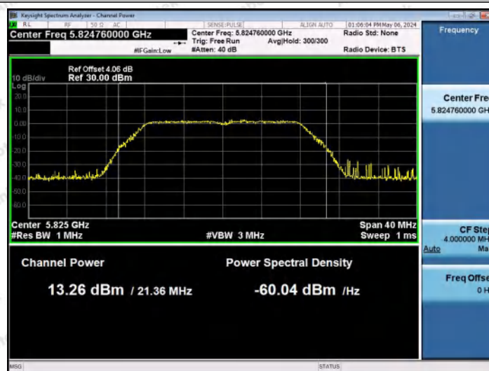
11A-Ant1-5825-PASS
