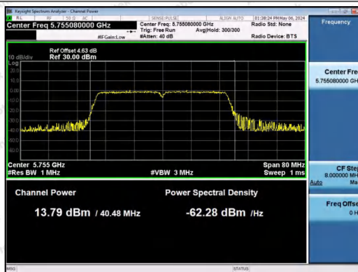
11N40MIMO-Ant0-5755-PASS
