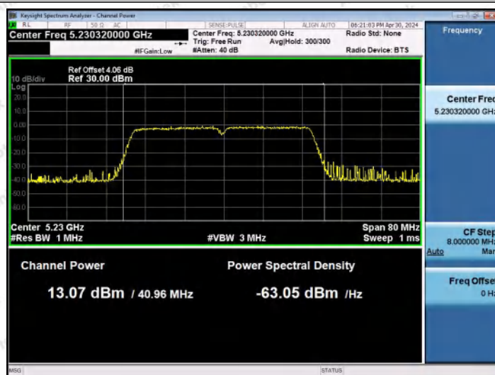
11AC40MIMO-Ant0-5230-PASS
