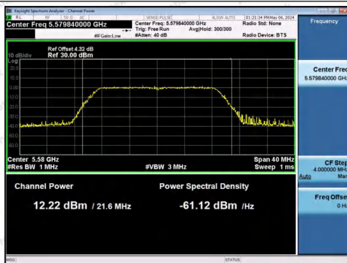
11N20MIMO-Ant0-5580-PASS
