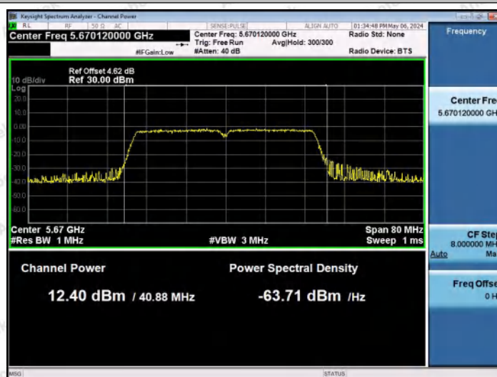
11N40MIMO-Ant1-5670-PASS
