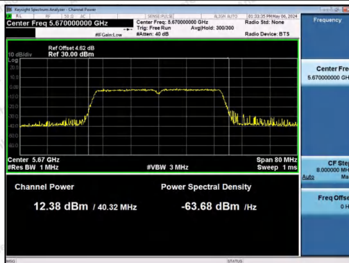
11N40MIMO-Ant0-5670-PASS
