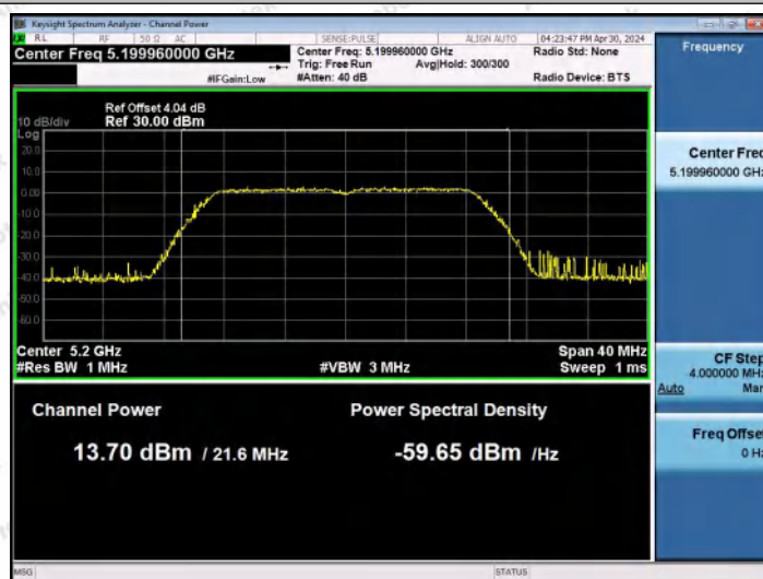
11AC20MIMO-Ant0-5200-PASS
