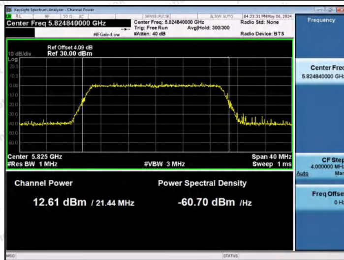
11AX20MIMO-Ant0-5825-PASS
