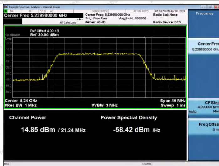
11AX20MIMO-Ant0-5240-PASS
