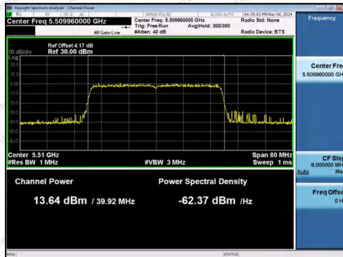
11AX40MIMO-Ant0-5510-PASS
