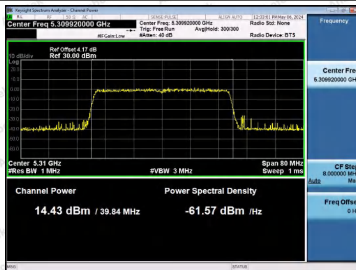
11AX40MIMO-Ant0-5310-PASS
