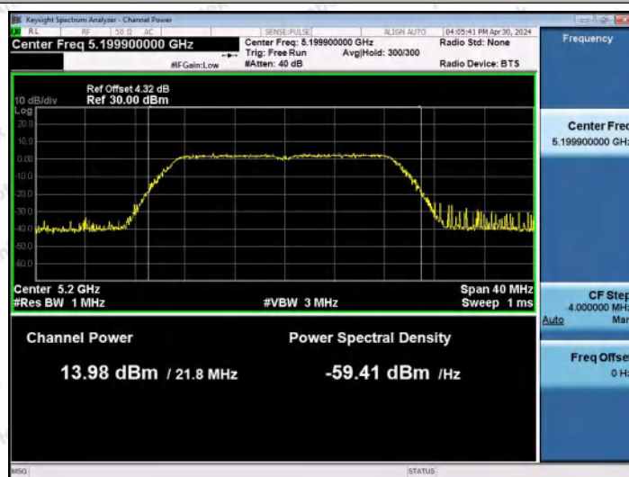
11N20MIMO-Ant0-5200-PASS
