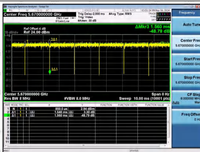
NTNV-11AC40MIMO-Ant1-5670
