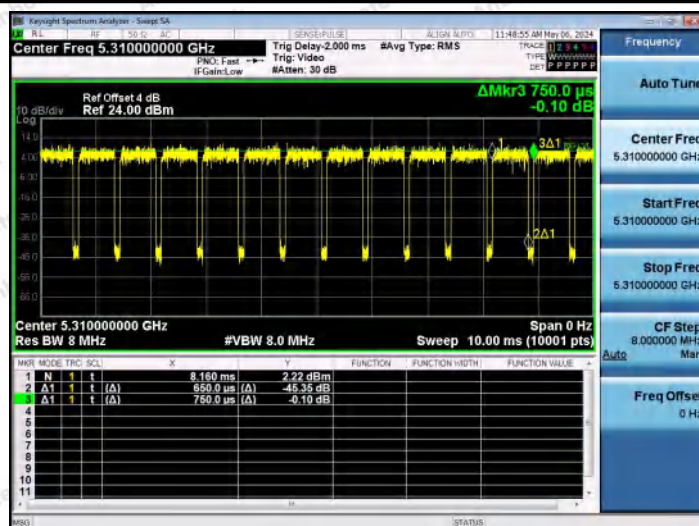
NTNV-11N40MIMO-Ant0-5310
