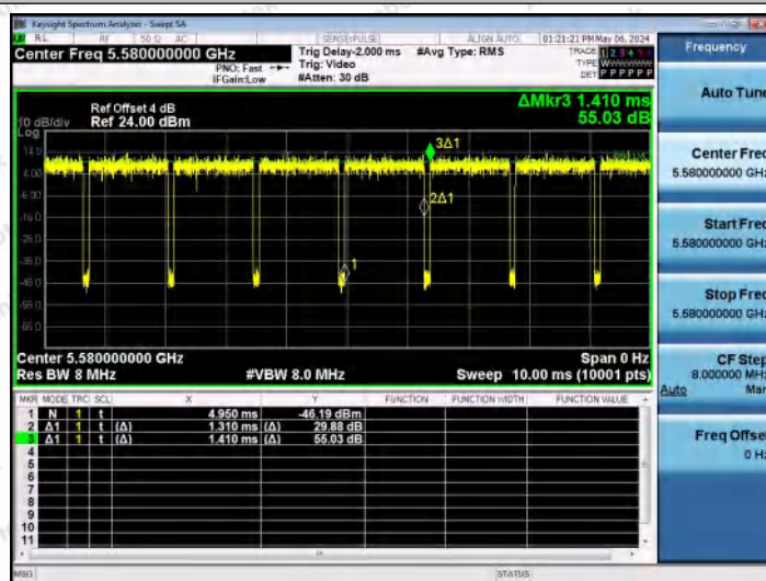
NTNV-11N20MIMO-Ant0-5580
