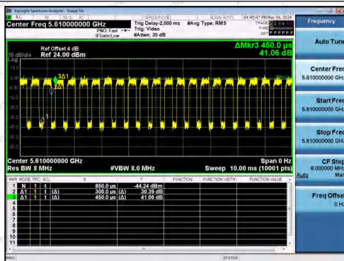
NTNV-11AX80MIMO-Ant1-5610
