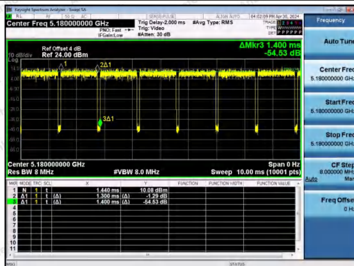
NTVN-11N20MIMO-Ant0-5180
