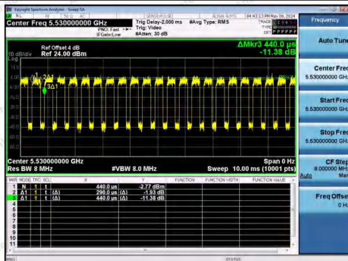
NTNV-11AX80MIMO-Ant1-5530
