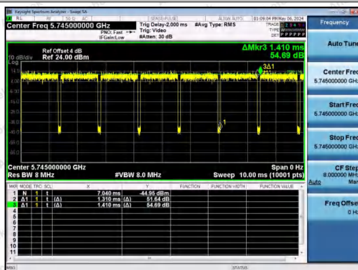
NTVN-11N20MIMO-Ant1-5745
