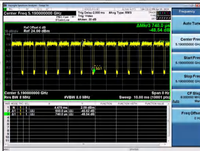
NTVN-11N40MIMO-Ant0-5190
