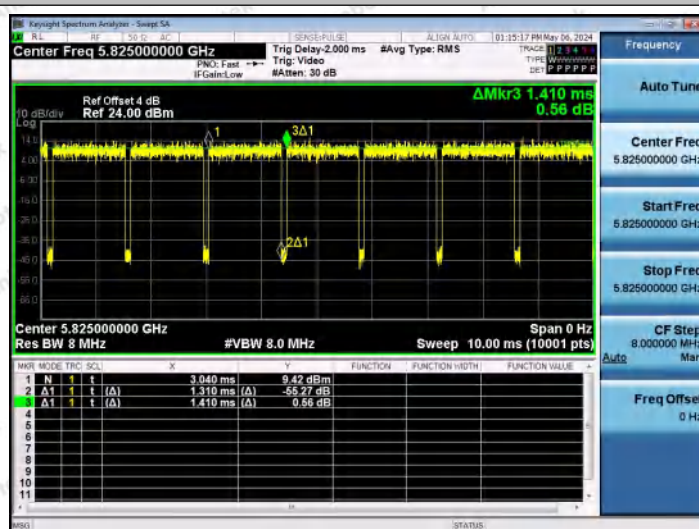
NTVN-11N20MIMO-Ant1-5825
