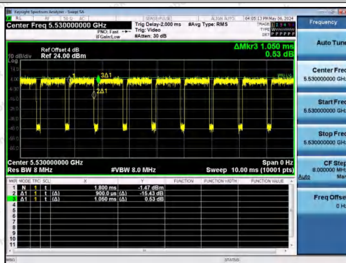
NTNV-11AC80MIMO-Ant1-5530
