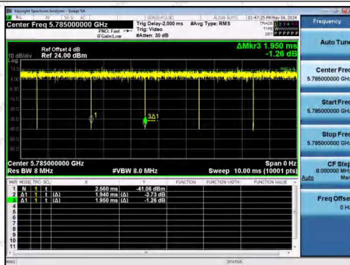
NTNV-11AC20MIMO-Ant0-5785
