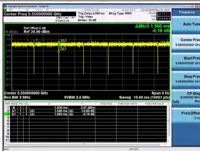
NTNV-11AC40MIMO-Ant1-5550
