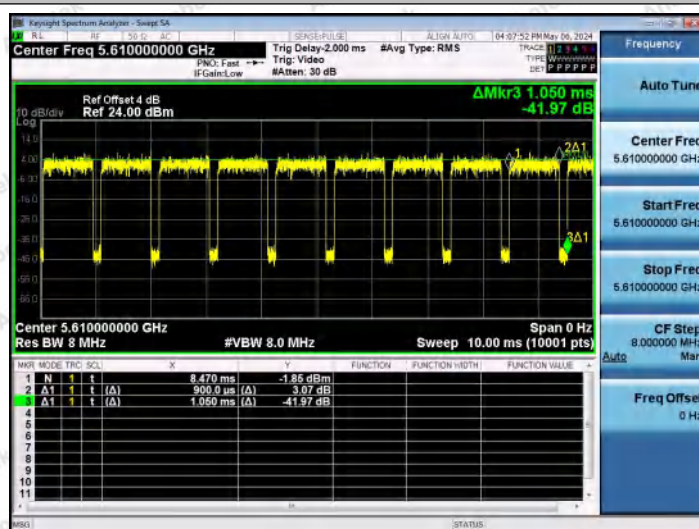
NTNV-11AC80MIMO-Ant1-5610
