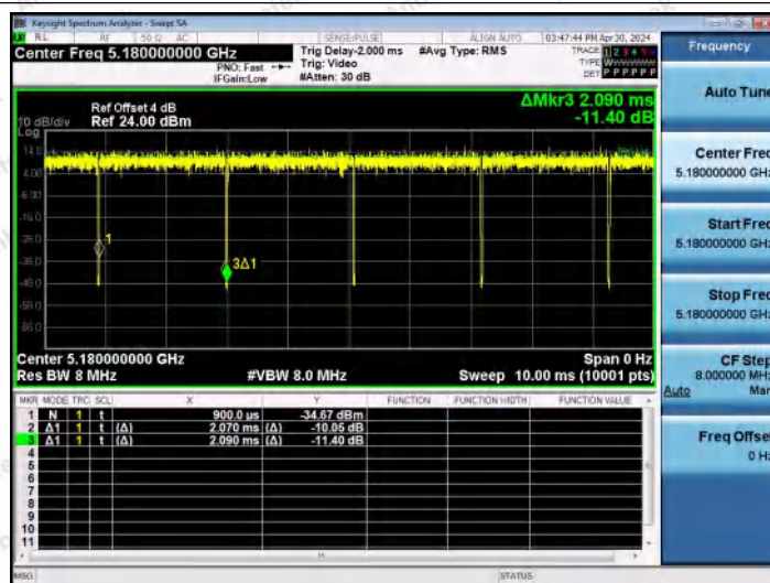
NTNV-11A-Ant0-5180
