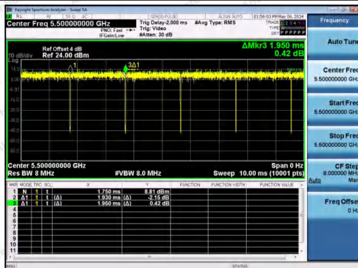
NTNV-11AC20MIMO-Ant0-5500
