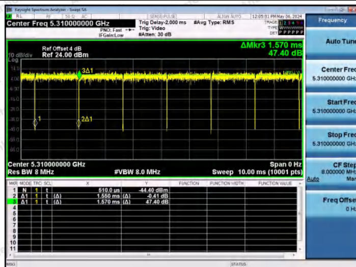
NTNV-11AC40MIMO-Ant0-5310
