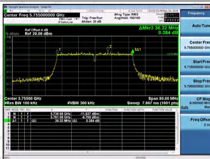
11AC40MIMO-Ant0-5755-PASS
