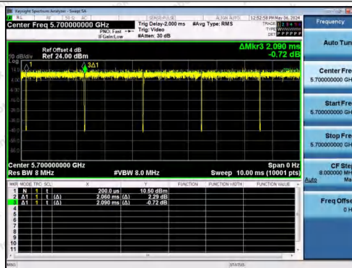
NTNV-11A-Ant1-5700
