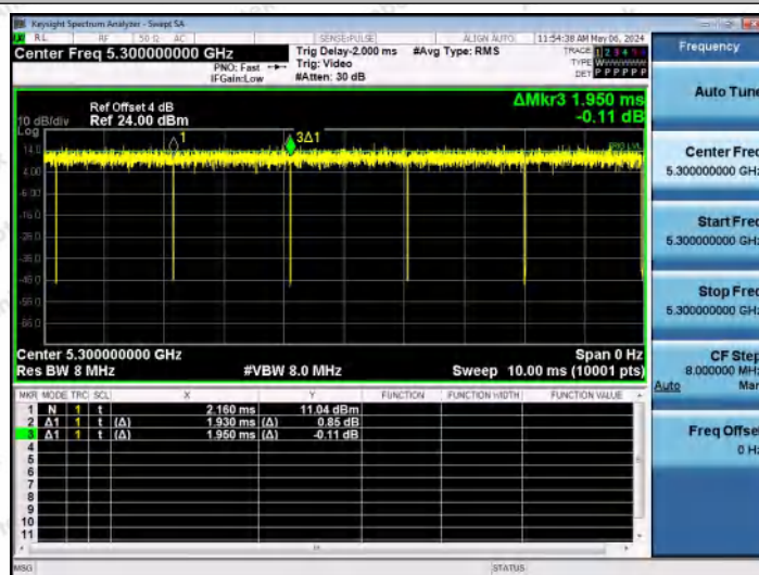
NTNV-11AC20MIMO-Ant0-5300
