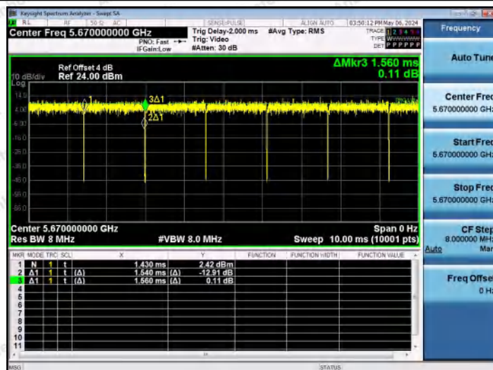
NTNV-11AC40MIMO-Ant0-5670
