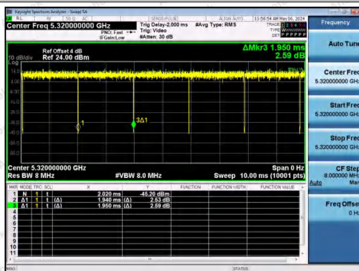
NTNV-11AC20MIMO-Ant0-5320
