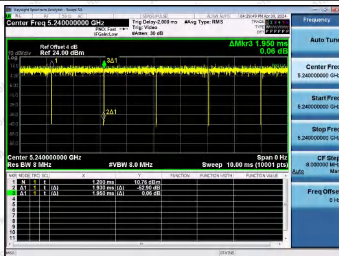
NTNV-11AC20MIMO-Ant0-5240
