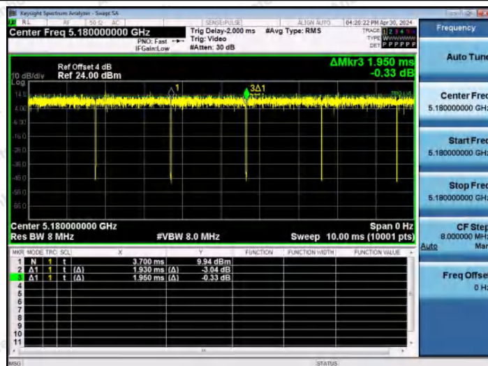
NTNV-11AC20MIMO-Ant0-5180
