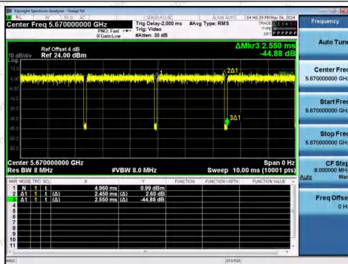
NTNV-11AX40MIMO-Ant1-5670
