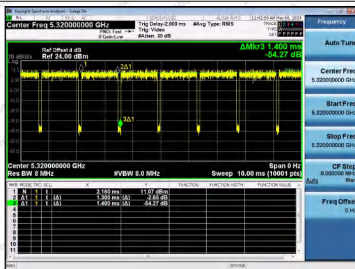
NTVN-11N20MIMO-Ant1-5320
