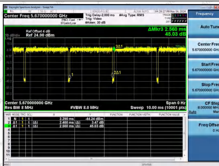
NTNV-11AX40MIMO-Ant0-5670
