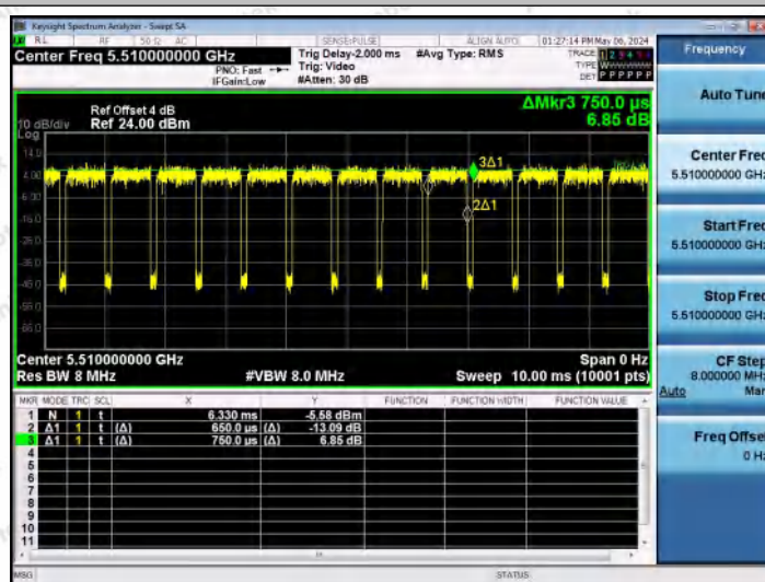
NTNV-11N40MIMO-Ant0-5510
