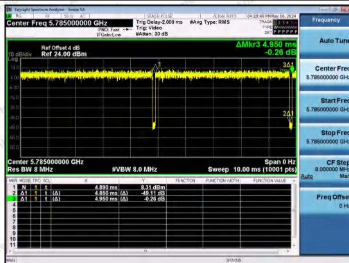
NTNV-11AX20MIMO-Ant0-5785
