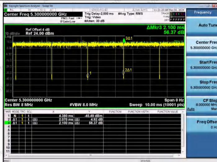
NTNV-11A-Ant1-5300
