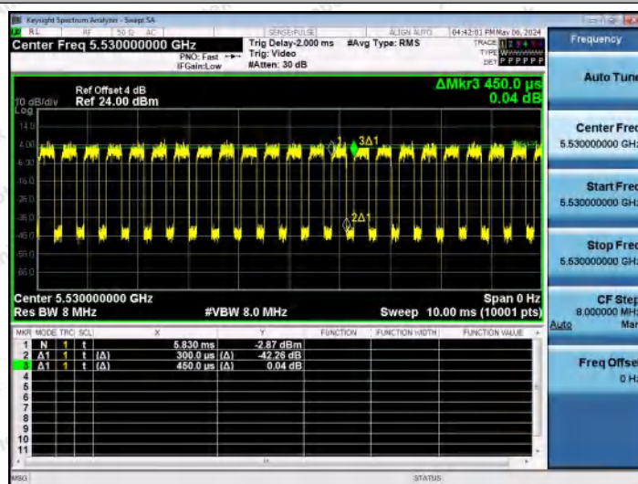
NTNV-11AX80MIMO-Ant0-5530
