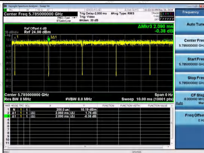
NTNV-11A-Ant0-5785
