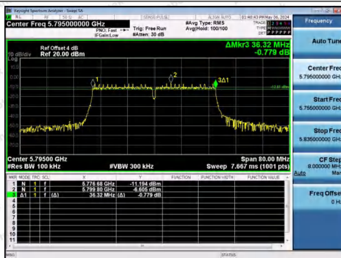
11N40MIMO-Ant0-5795-PASS
