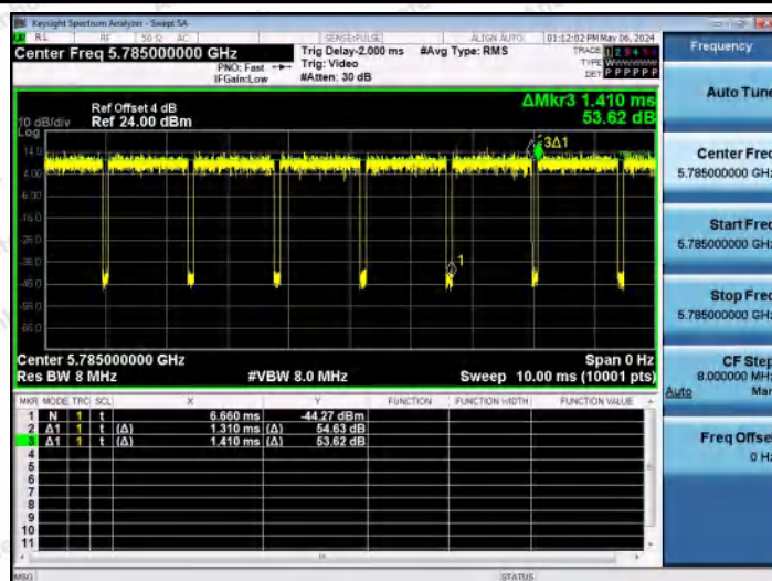
NTVN-11N20MIMO-Ant1-5785
