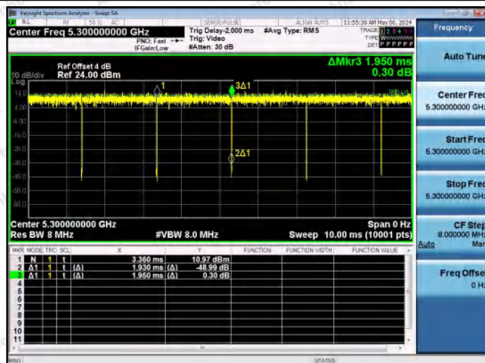
NTNV-11AC20MIMO-Ant1-5300
