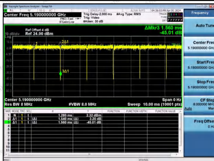
NTNV-11AC40MIMO-Ant0-5190
