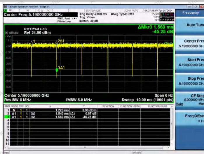
NTNV-11AC40MIMO-Ant1-5190
