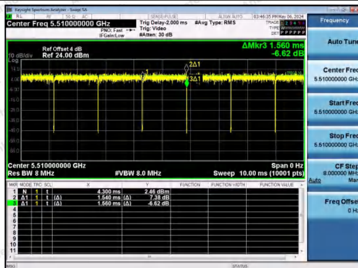
NTNV-11AC40MIMO-Ant1-5510
