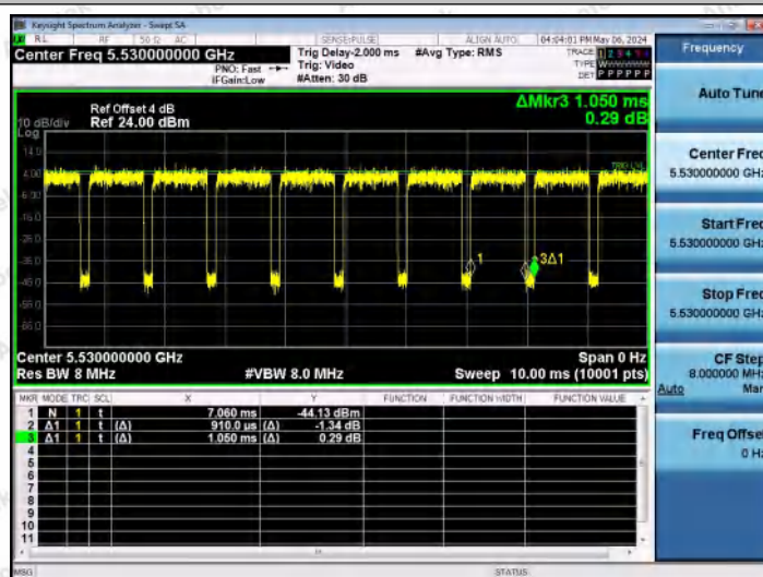
NTNV-11AC80MIMO-Ant0-5530
