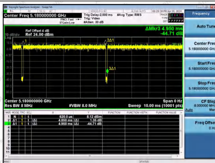
NTNV-11AX20MIMO-Ant0-5180
