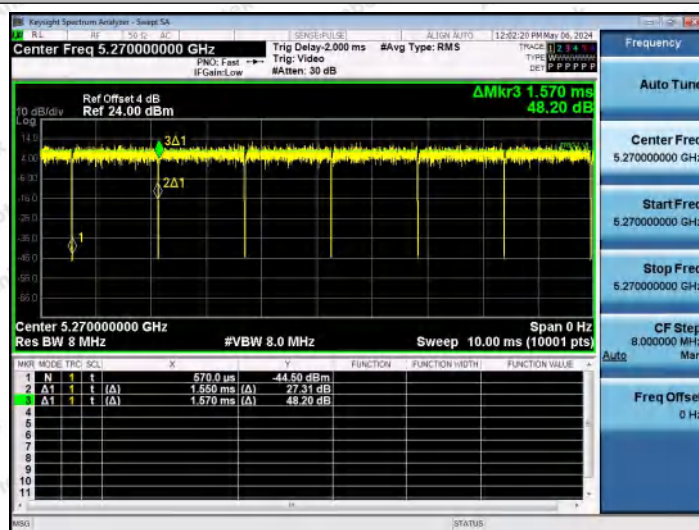
NTNV-11AC40MIMO-Ant1-5270
