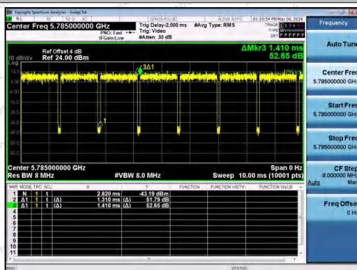
NTVN-11N20MIMO-Ant0-5785
