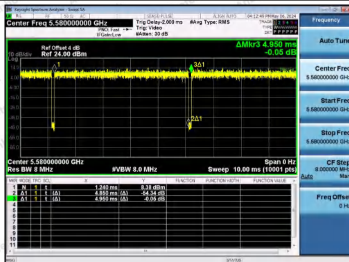
NTNV-11AX20MIMO-Ant0-5580
