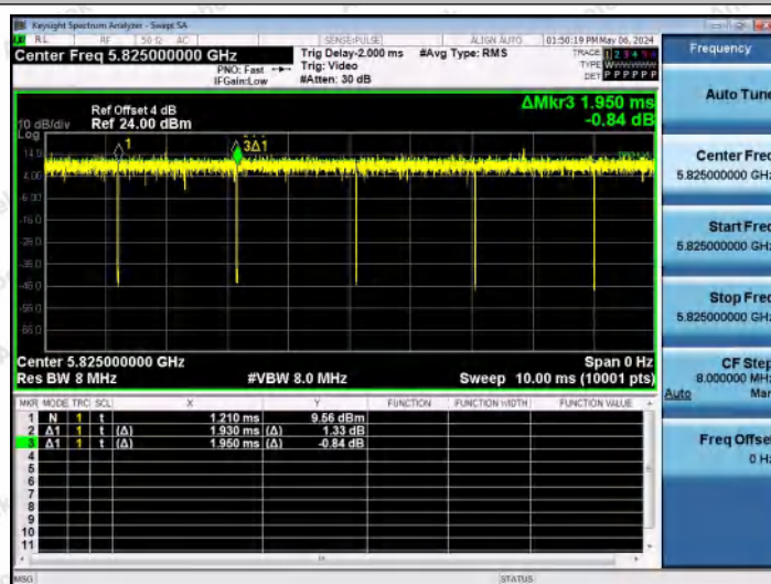
NTNV-11AC20MIMO-Ant0-5825
