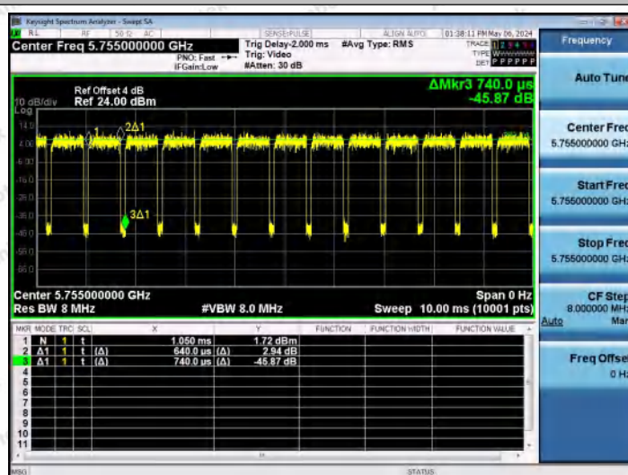
NTNV-11N40MIMO-Ant0-5755
