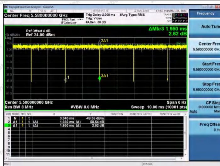
NTNV-11AC20MIMO-Ant0-5580
