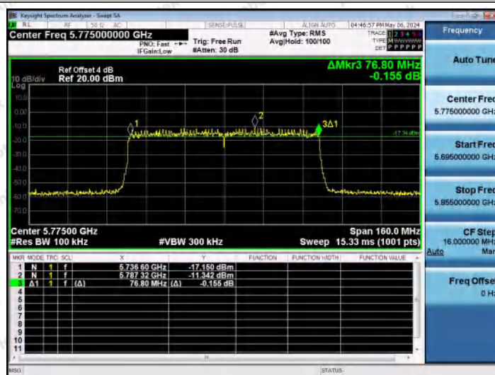
11AX80MIMO-Ant0-5775-PASS
