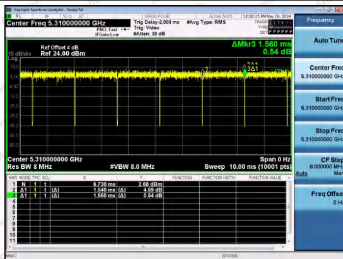
NTNV-11AC40MIMO-Ant1-5310
