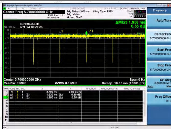
NTNV-11AC20MIMO-Ant1-5700
