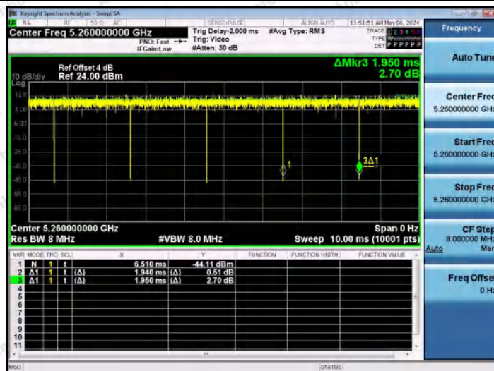
NTNV-11AC20MIMO-Ant0-5260
