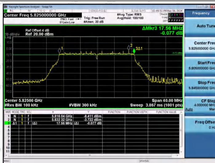
11AC20MIMO-Ant0-5825-PASS
