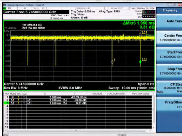
NTNV-11AC20MIMO-Ant0-5745
