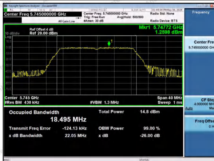
11AC20MIMO-Ant0-5745
