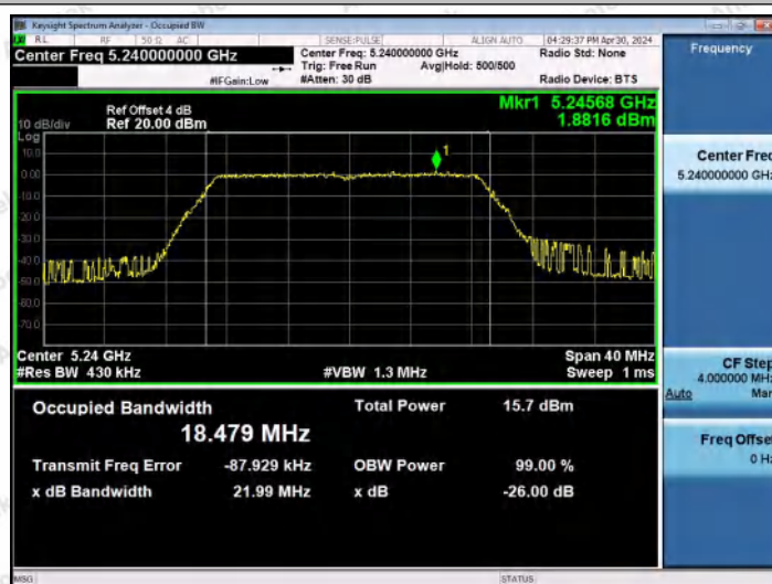
11AC20MIMO-Ant0-5240
