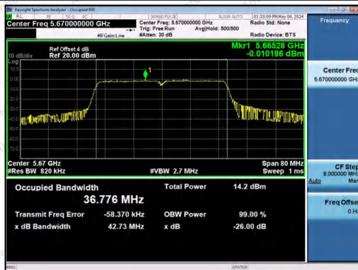
11N40MIMO-Ant0-5670
