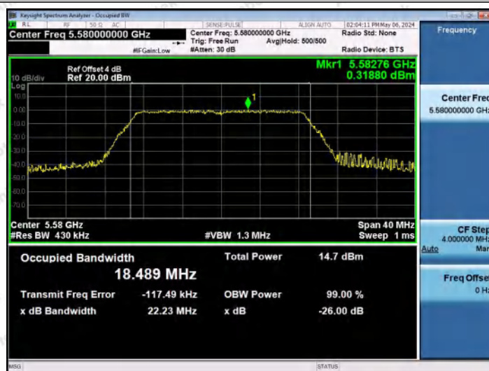
11AC20MIMO-Ant0-5580
