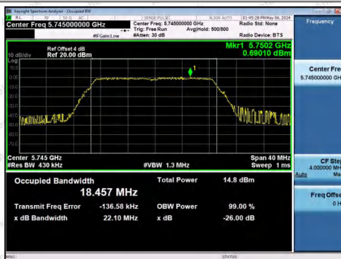
11AC20MIMO-Ant1-5745
