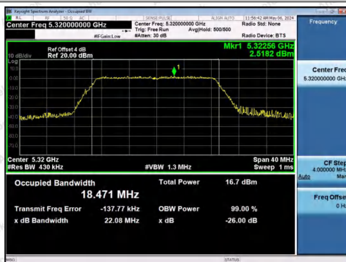
11AC20MIMO-Ant0-5320
