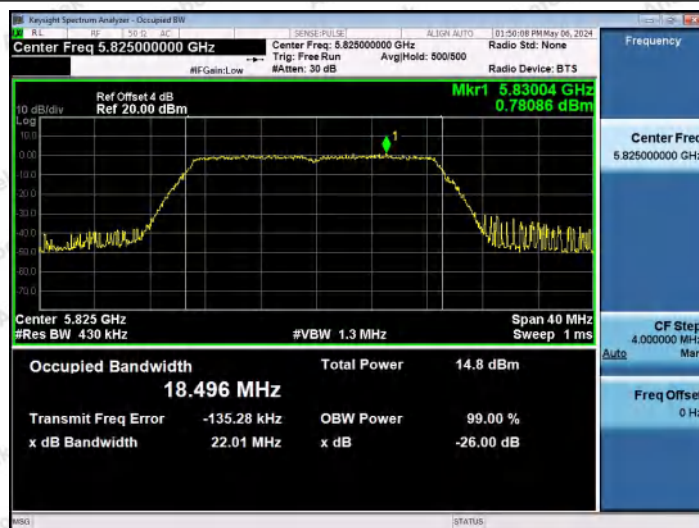
11AC20MIMO-Ant0-5825
