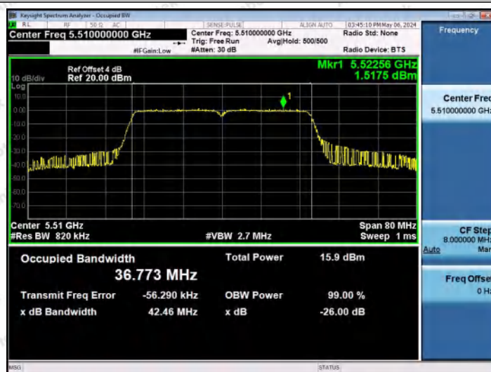
11AC40MIMO-Ant0-5510
