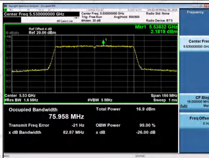
11AC80MIMO-Ant0-5530
