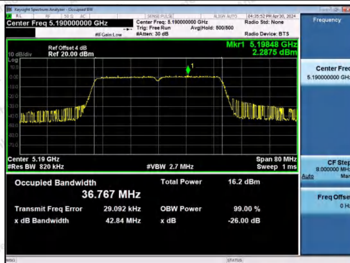
11AC40MIMO-Ant0-5190
