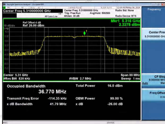
11AC40MIMO-Ant0-5310
