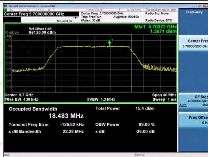
11AC20MIMO-Ant1-5700
