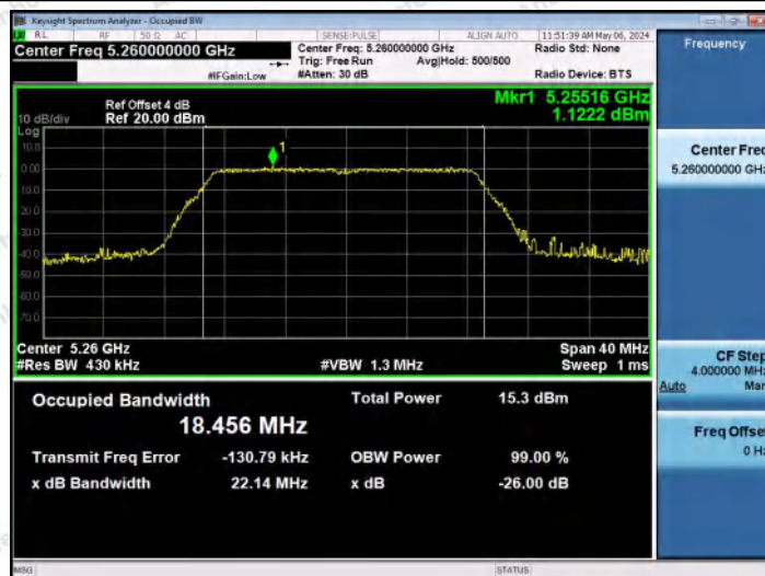
11AC20MIMO-Ant0-5260
