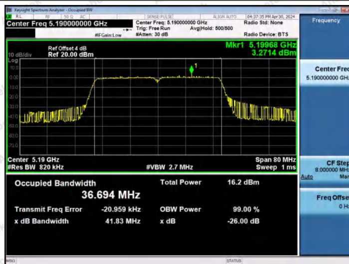
11AC40MIMO-Ant1-5190
