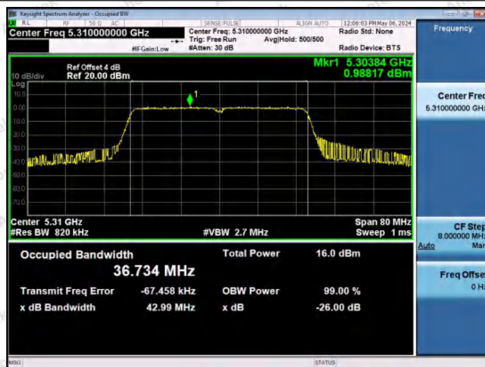
11AC40MIMO-Ant1-5310
