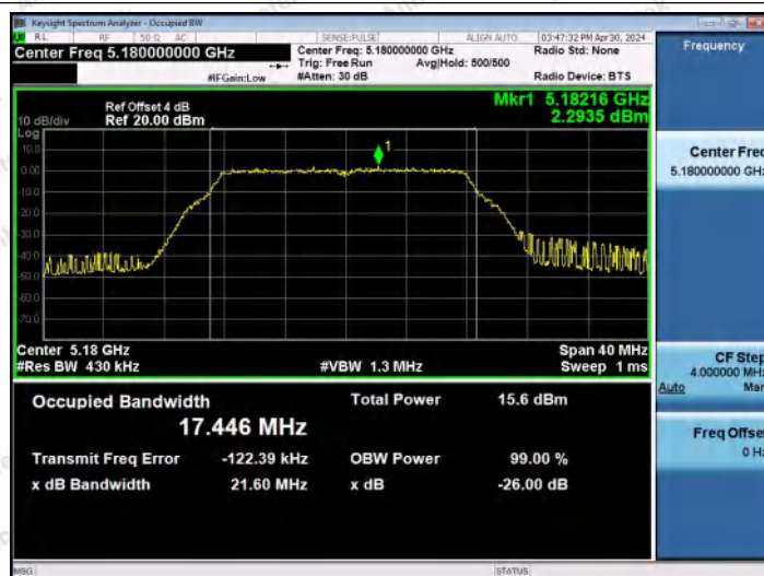
11A-Ant0-5180
