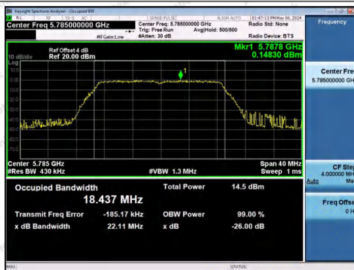
11AC20MIMO-Ant0-5785
