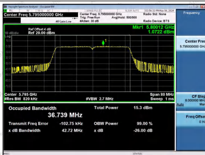
11AC40MIMO-Ant2-5795
