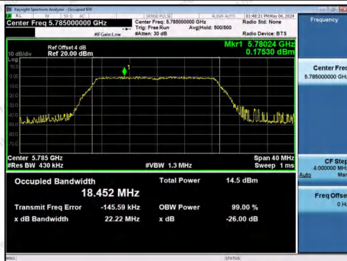
11AC20MIMO-Ant1-5785
