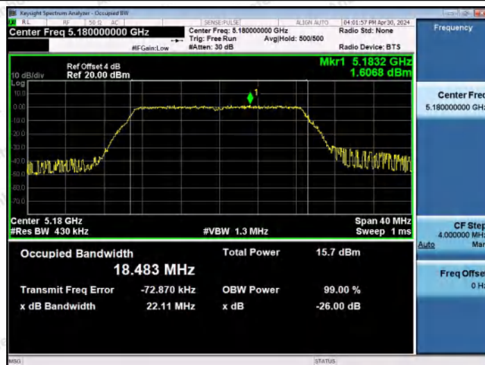
11N20MIMO-Ant0-5180
