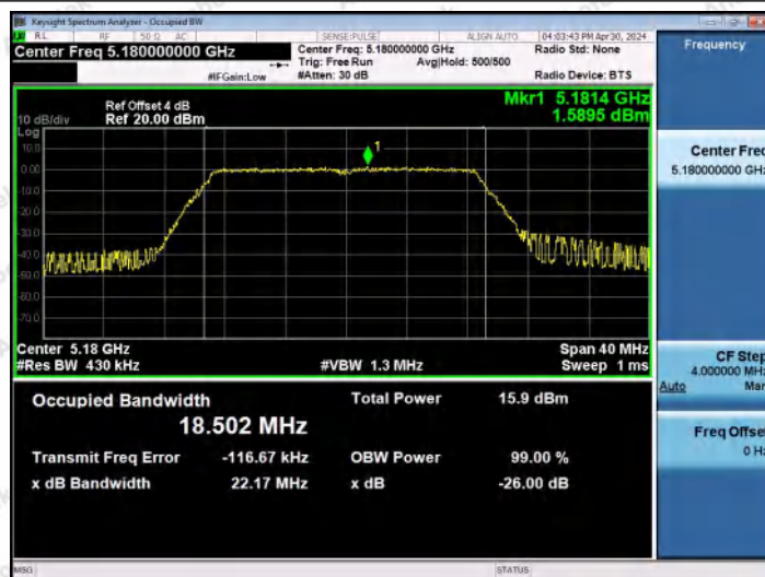
11N20MIMO-Ant1-5180
