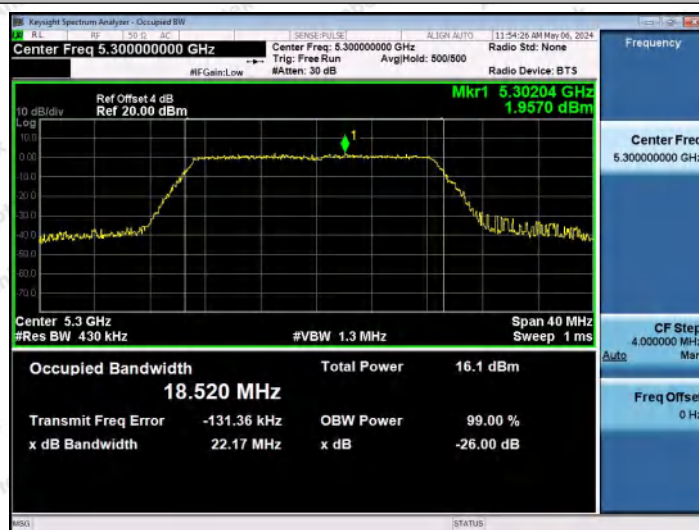
11AC20MIMO-Ant0-5300
