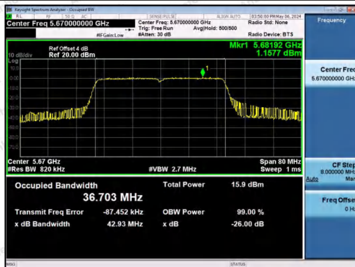
11AC40MIMO-Ant0-5670
