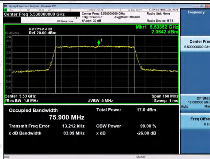
11AC80MIMO-Ant1-5530
