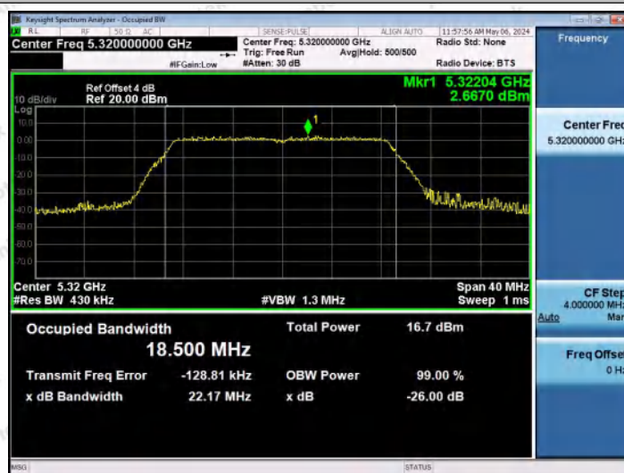
11AC20MIMO-Ant1-5320
