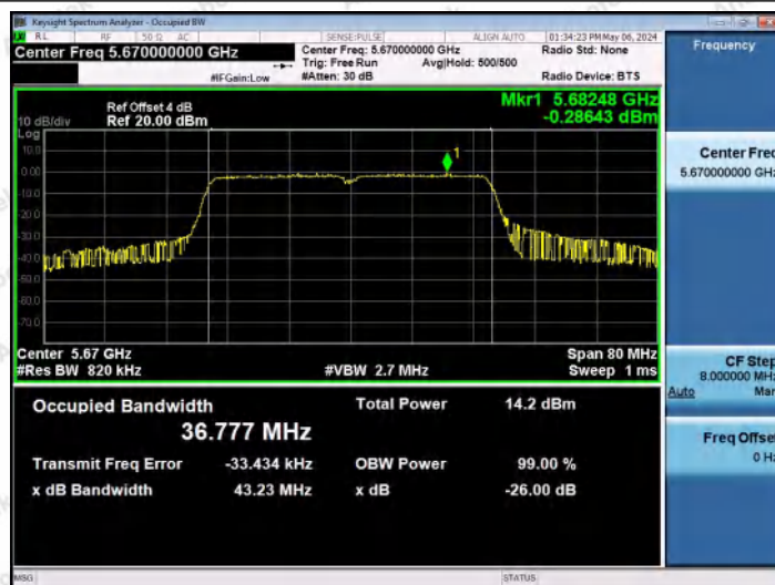
11N40MIMO-Ant1-5670
