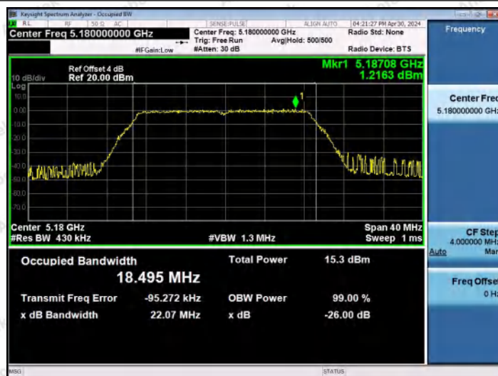
11AC20MIMO-Ant1-5180
