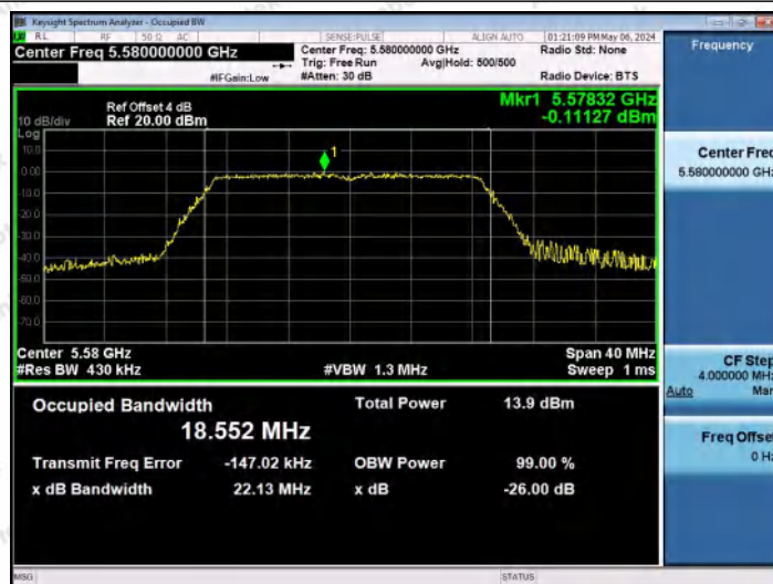
11N20MIMO-Ant0-5580
