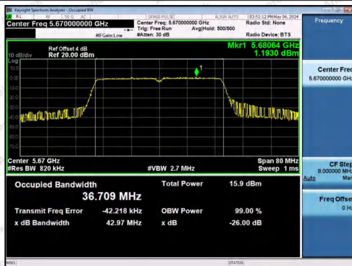
11AC40MIMO-Ant1-5670
