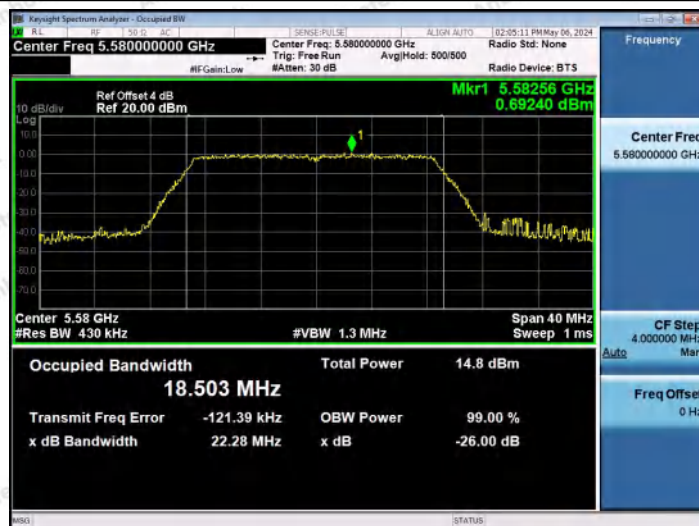
11AC20MIMO-Ant1-5580
