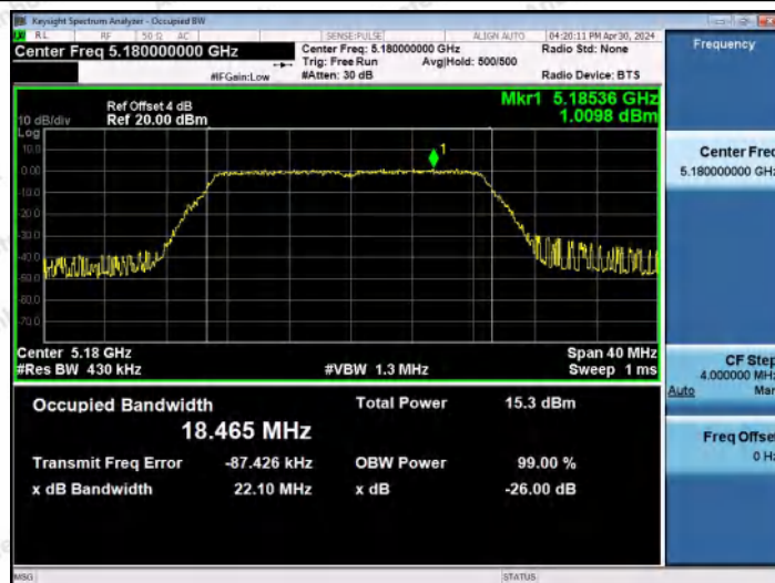
11AC20MIMO-Ant0-5180
