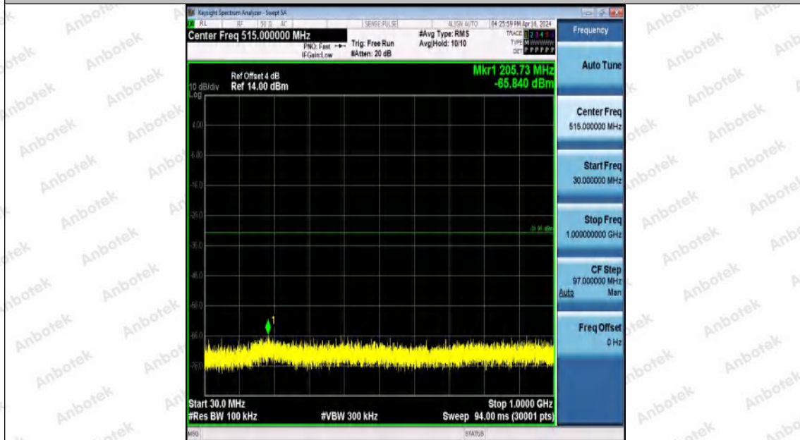
11N20MIMO-Ant1-2412-30~1000-PASS
