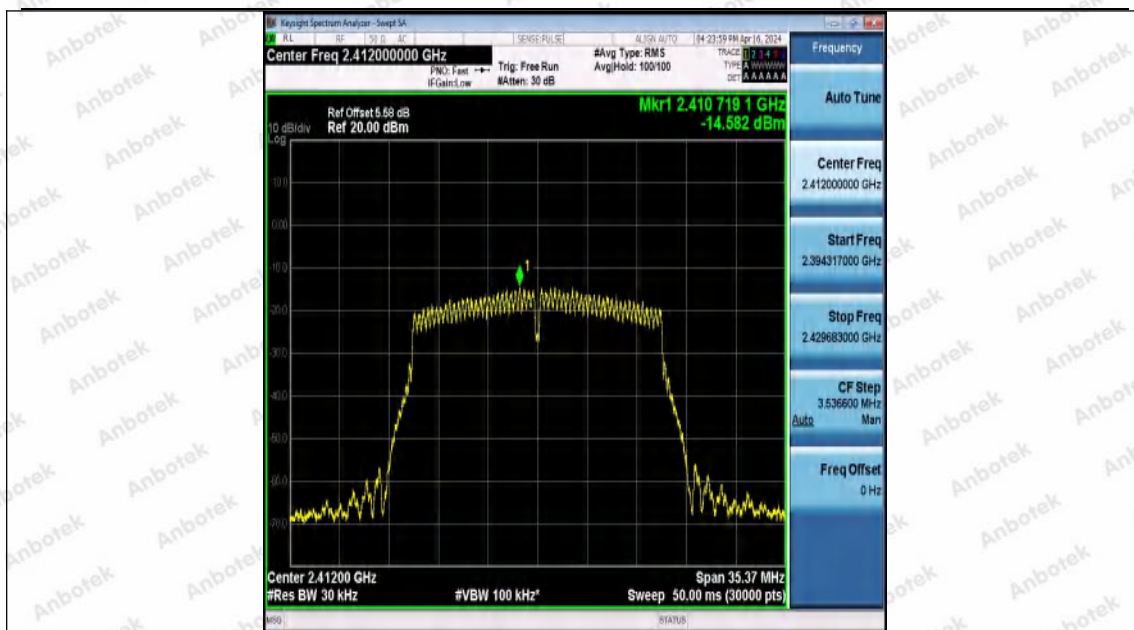
11N20MIMO-Ant0-2412-PASS
