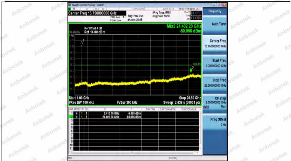
11AX20MIMO-Ant0-2412-1000~26500-PASS
