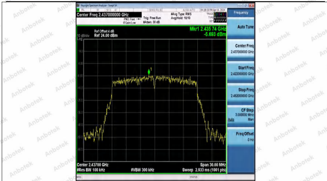
11N20MIMO-Ant0-2437-0-Reference-PASS
