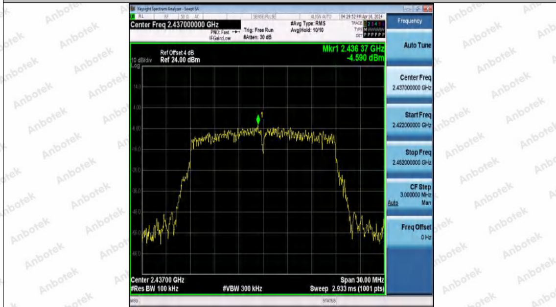
11N20MIMO-Ant1-2437-0-Reference-PASS
