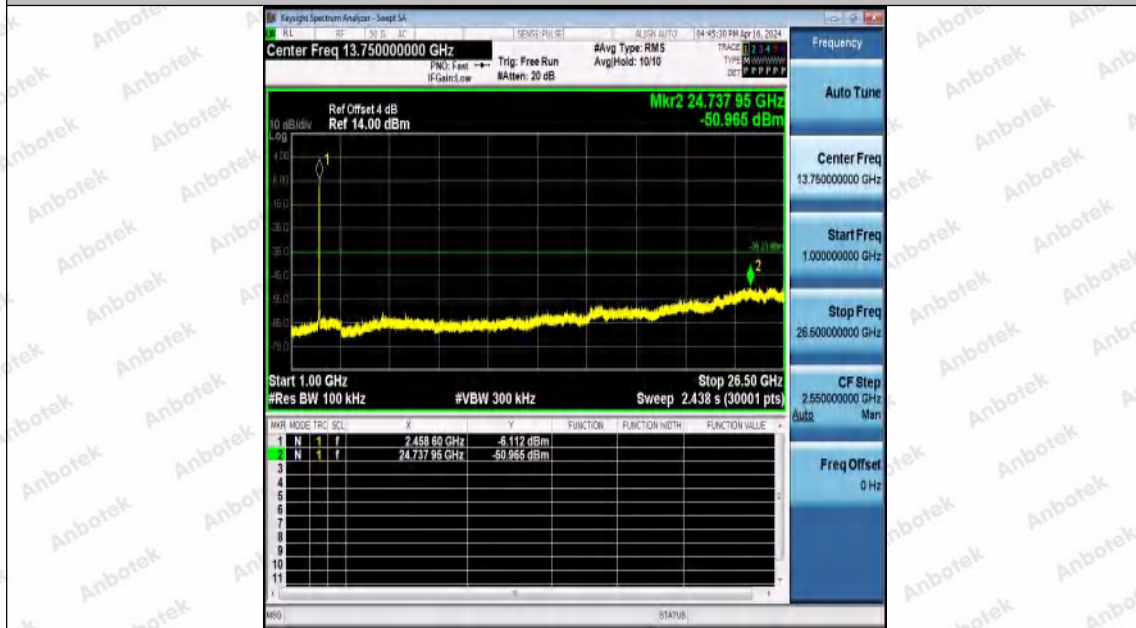
11AX20MIMO-Ant1-2462-1000~26500-PASS
