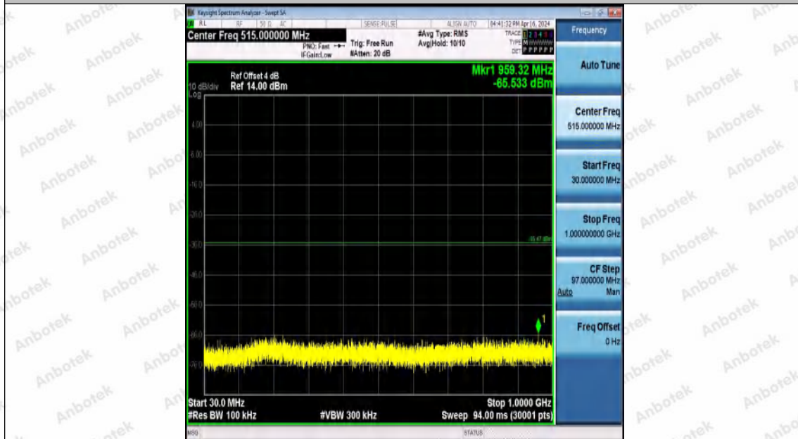
11AX20MIMO-Ant1-2437-30~1000-PASS
