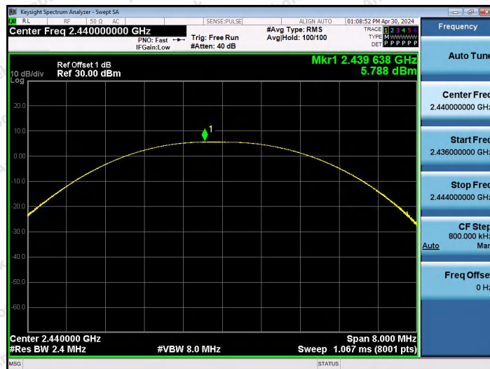
BLE_1M-Ant0-2440-PASS
