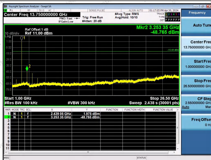
BLE_2M-Ant0-2440-1000~26500-PASS
