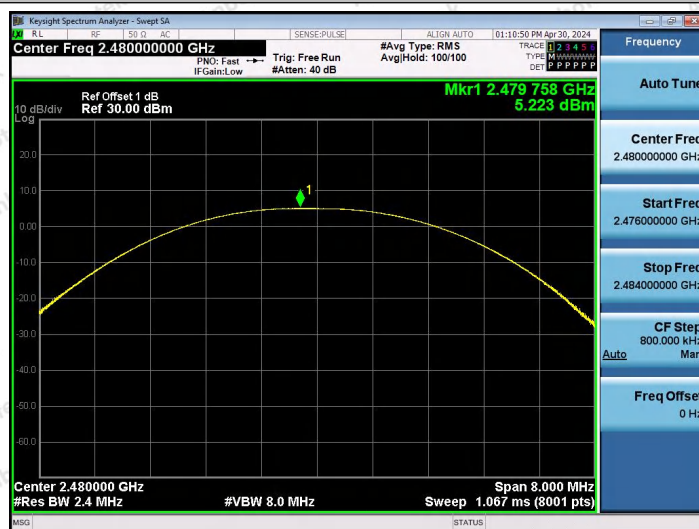
BLE_1M-Ant0-2480-PASS
