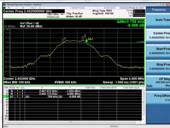
BLE_1M-Ant0-2402-PASS
