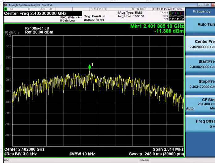
BLE_2M-Ant0-2402-PASS
