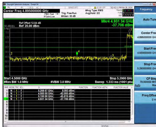
11AX40SISO_Ant1_High_5310_Peak
