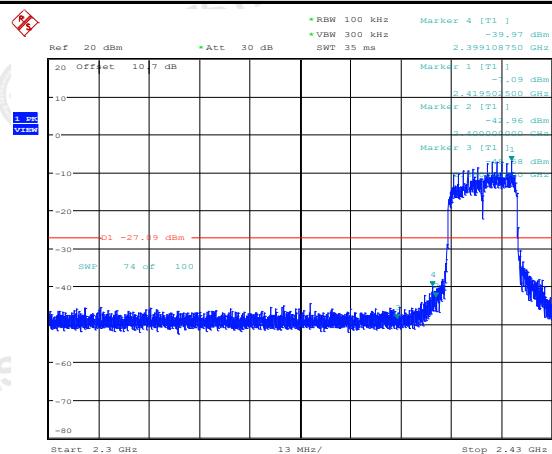
Left bandedge
