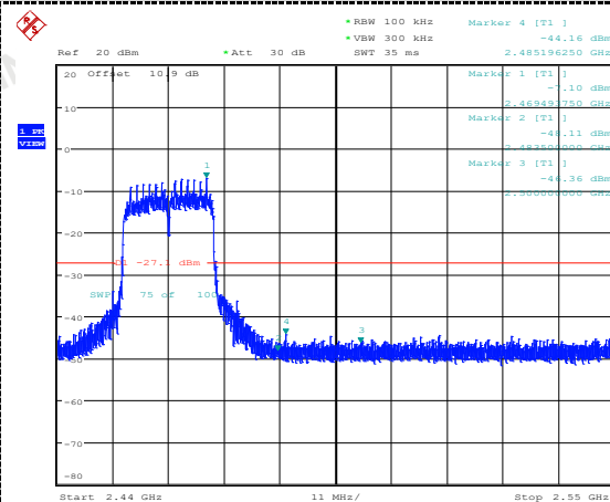
Right bandedge
