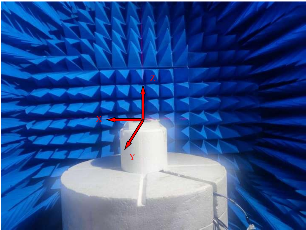
Test Arrangement
