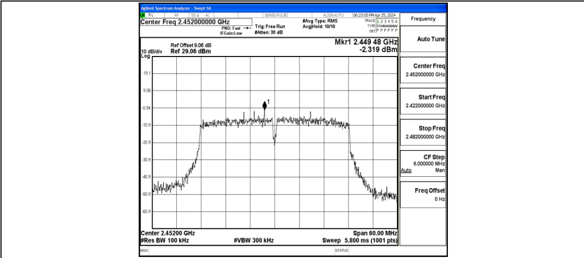
11N40SISO-Ant1-2452-0~Reference-PASS
