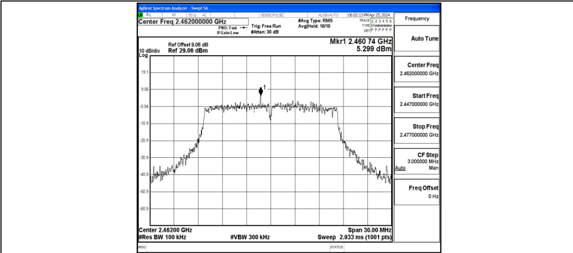
11G-Ant1-2462-0~Reference-PASS
