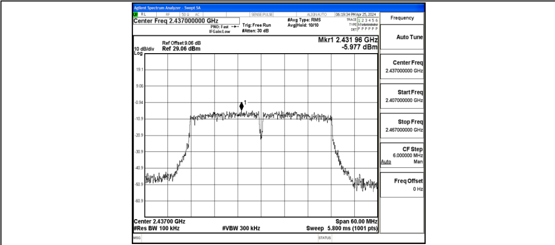
11N40SISO-Ant1-2437-0~Reference-PASS
