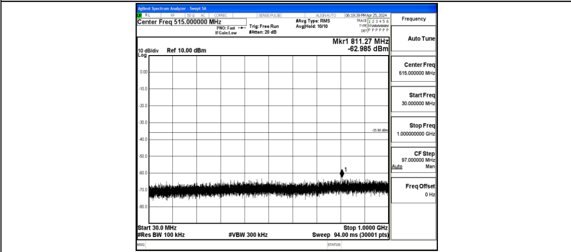
11N40SISO-Ant1-2437-30~1000-PASS
