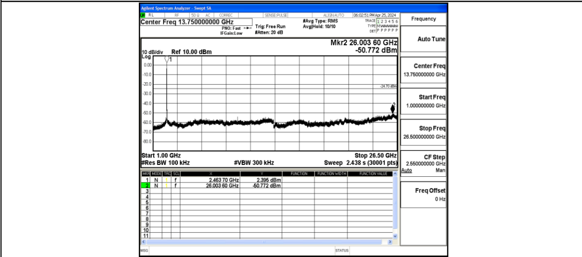
11G-Ant1-2462-1000~26500-PASS
