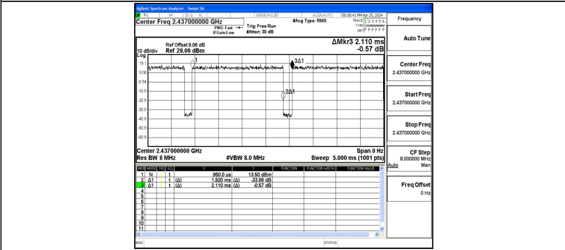
NTNV-11N20SISO-Ant1-2437
