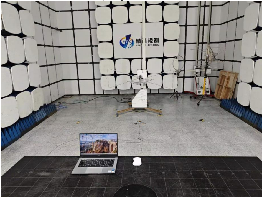
Radiated Spurious Emissions Test Frequency From 30MHz-1GHz
