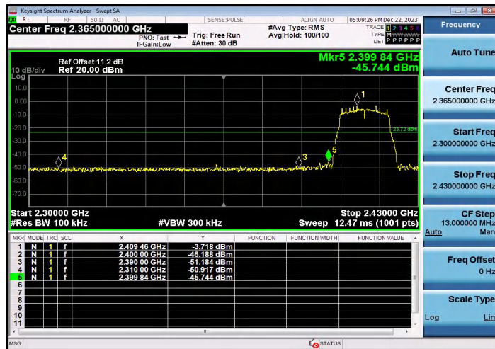
Left bandedge
