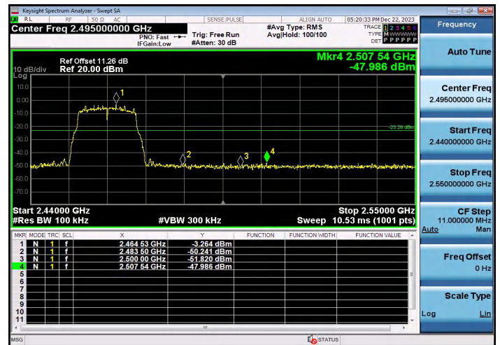
Right bandedge
