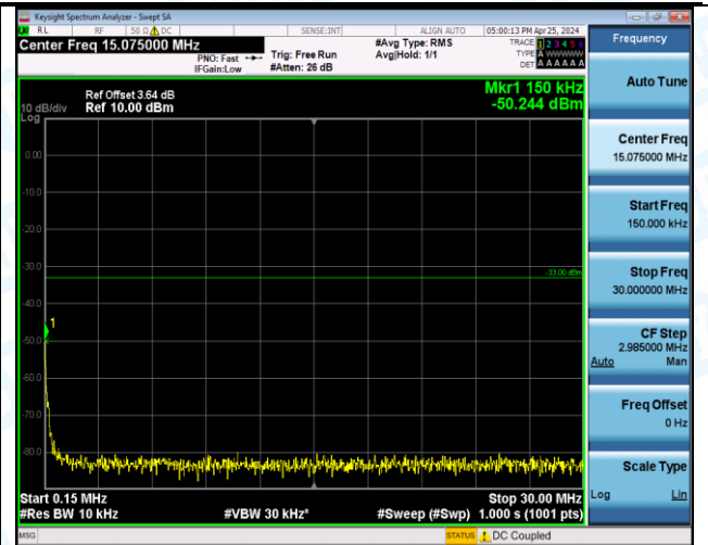
Band66_3MHz_16QAM_132322_1RB#0_1000~3000_1000~3000
