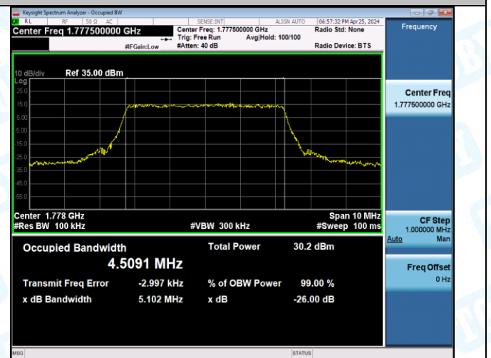
Band66-10MHz-QPSK-132322-50RB#0-PASS
