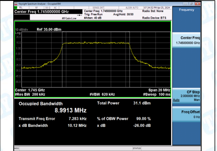
Band66-10MHz-16QAM-132022-27RB#0-PASS
