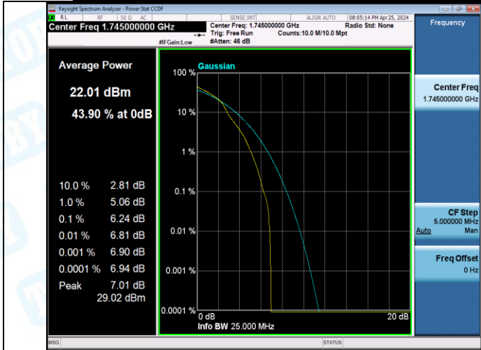
Band66-10MHz-16QAM-132622-1RB#0-PASS
