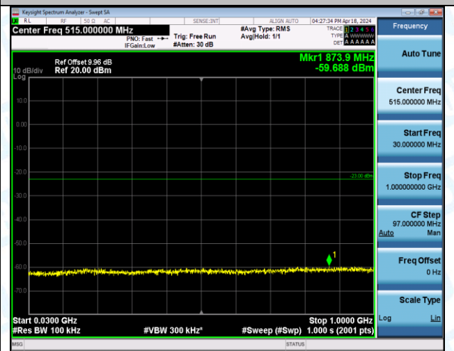
Band4_20MHz_16QAM_20175_1RB#0_3000~20000_3000~20000
