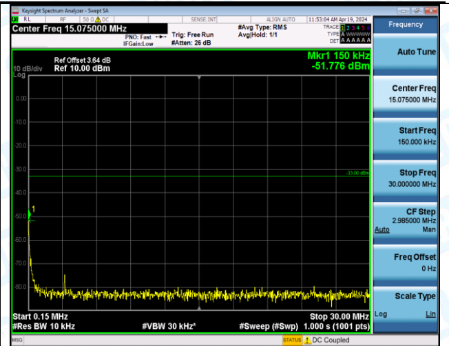
Band2_5MHz_QPSK_19175_1RB#0_1000~3000_1000~3000
