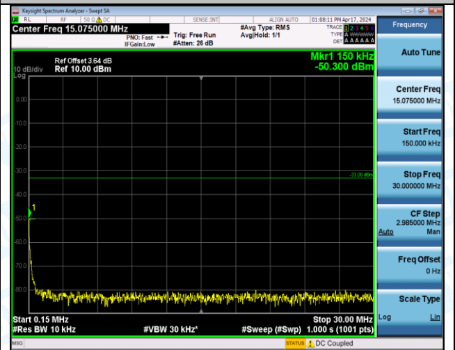
Band2_1.4MHz_16QAM_19193_1RB#5_1000~3000_1000~3000
