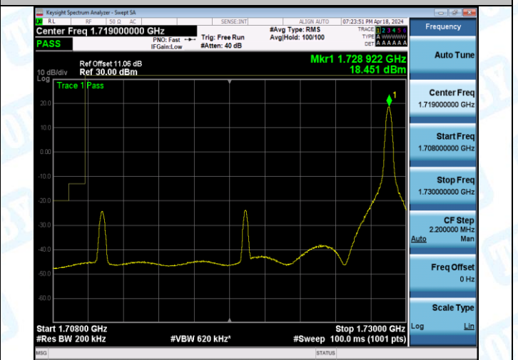
Band4_20MHz_16QAM_20300_1RB#99
