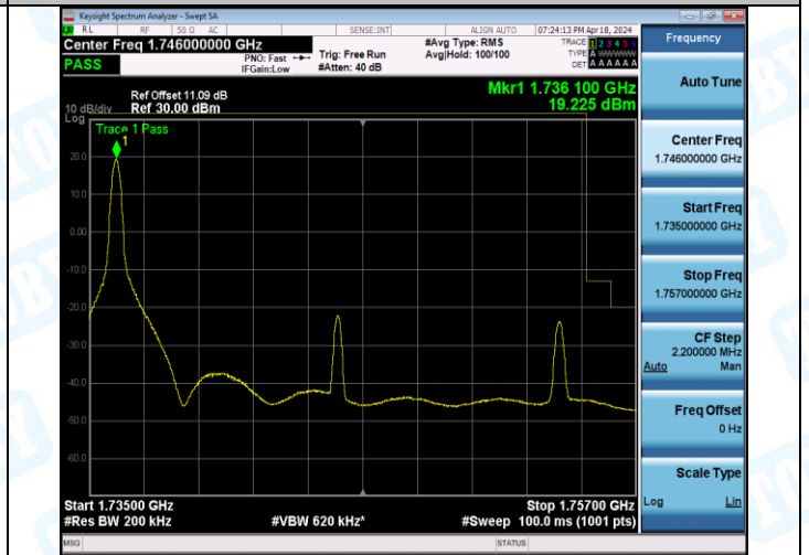
Band4_20MHz_QPSK_20300_100RB#0
