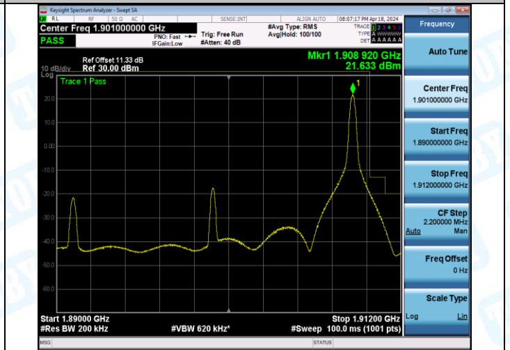
Band2_20MHz_16QAM_19100_1RB#99
