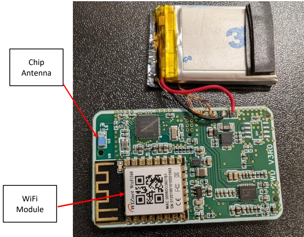
Photograph 1 – Front View of the PCBA
